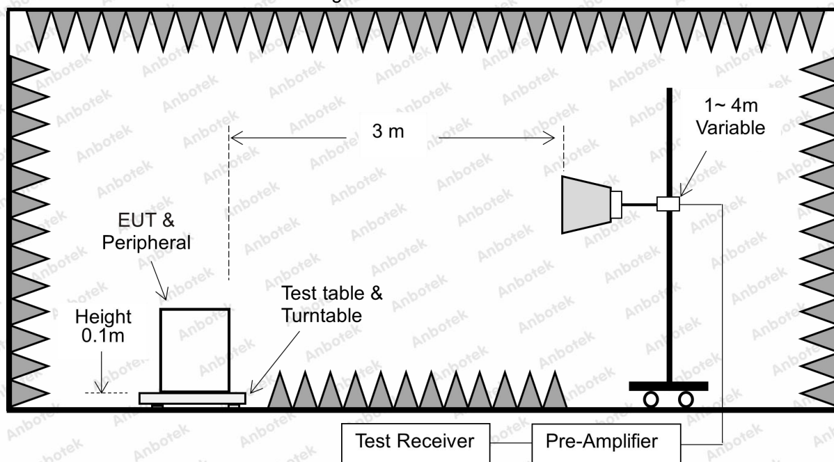
Figure 3. Above 1 GHz
