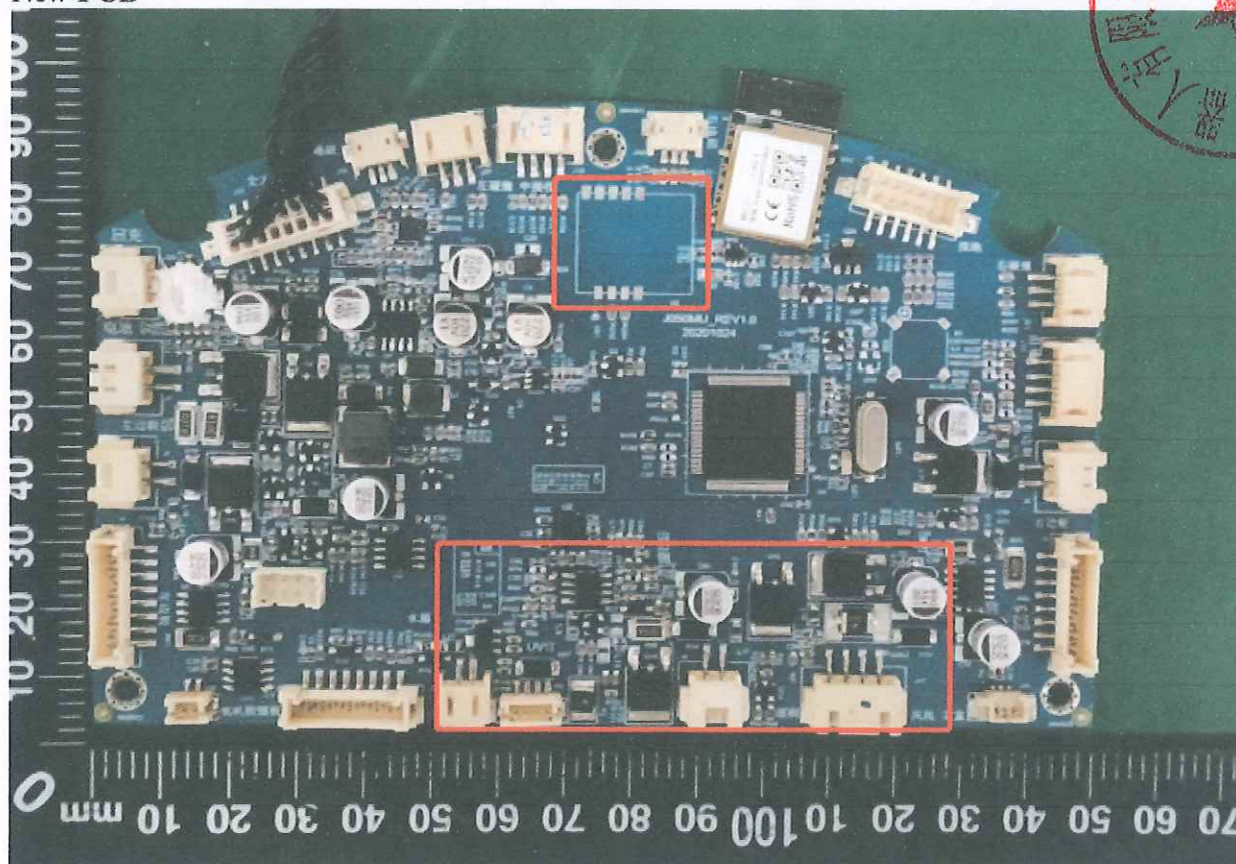
New PCB
