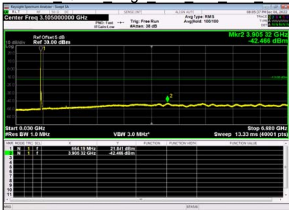
N71(20M)_DFT-s- OFDM QPSK Edge 1RB Left Low CH
