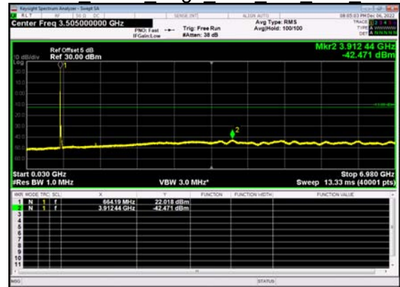
N71(20M)_DFT-s- OFDM BPSK Edge 1RB Left Low CH
