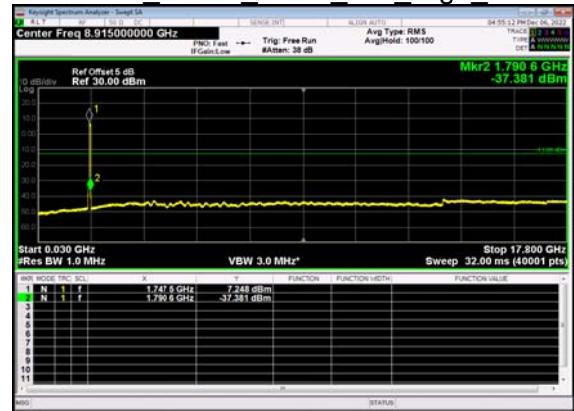
N66(40M)_DFT-s- OFDM QPSK Outer Full High CH
