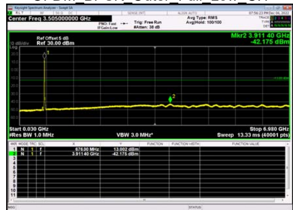
N71(15M)_DFT-s- OFDM BPSK Outer Full Low CH
