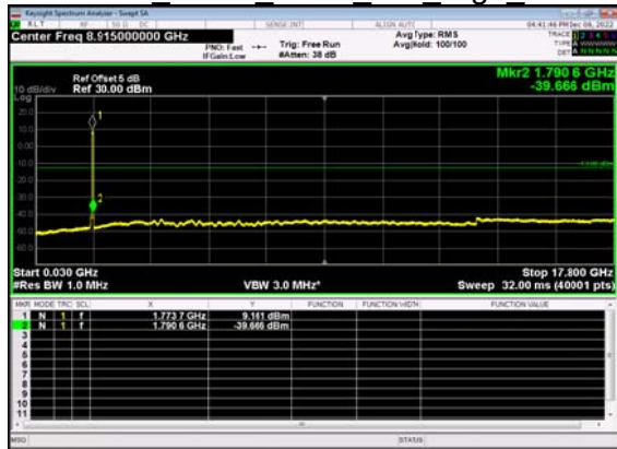
N66(30M)_DFT-s- OFDM BPSK Outer Full High CH
