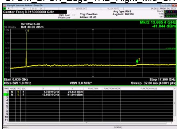
N66(30M)_DFT-s- OFDM BPSK Edge 1RB Right Mid CH
