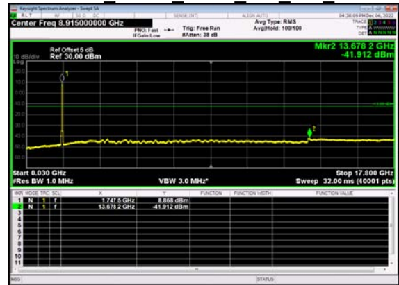
N66(30M)_DFT-s- OFDM QPSK Outer Full Mid CH
