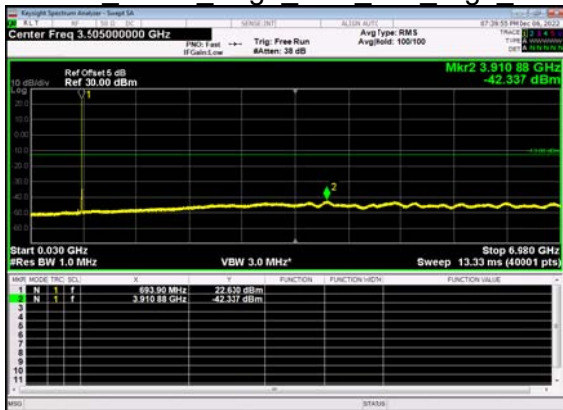
N71(5M)_DFT-s- OFDM BPSK Edge 1RB Left High CH
