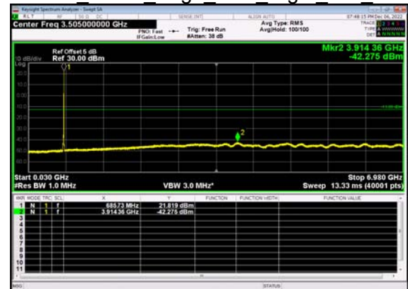
N71(10M)_DFT-s- OFDM BPSK Edge 1RB Right Mid CH
