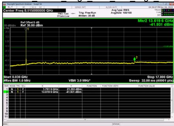
N66(30M)_DFT-s- OFDM BPSK Edge 1RB Left High CH
