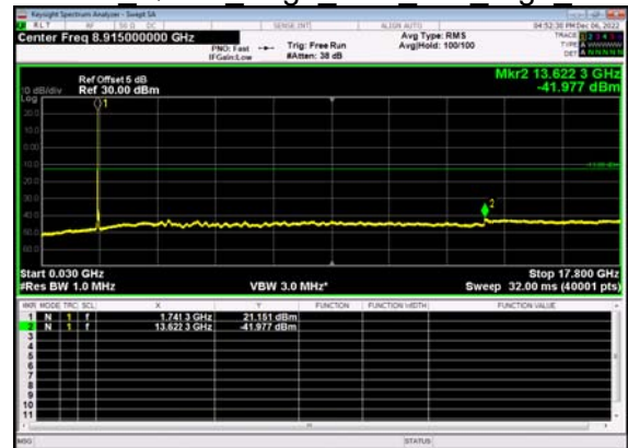
N66(40M)_DFT-s- OFDM QPSK Edge 1RB Left High CH
