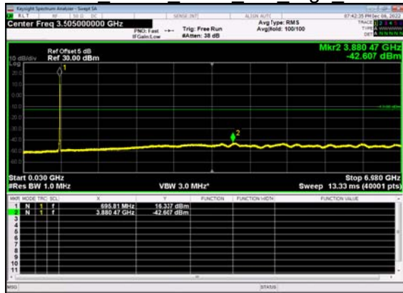
N71(5M)_DFT-s- OFDM QPSK Outer Full High CH
