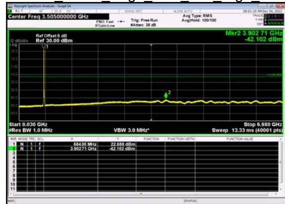
N71(15M)_DFT-s- OFDM BPSK Edge 1RB Left High CH
