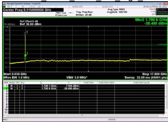
N66(40M)_DFT-s- OFDM BPSK Outer Full High CH
