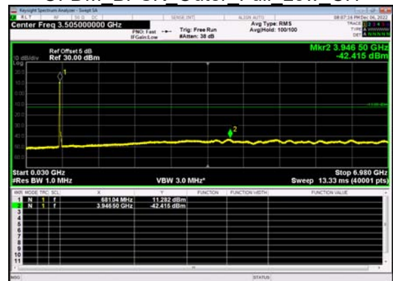
N71(20M)_DFT-s- OFDM BPSK Outer Full Low CH
