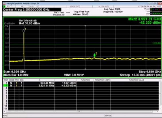
N71(15M)_DFT-s- OFDM QPSK Outer Full Low CH
