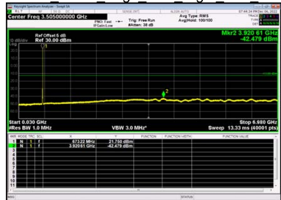
N71(10M)_DFT-s- OFDM BPSK Edge 1RB Right Low CH
