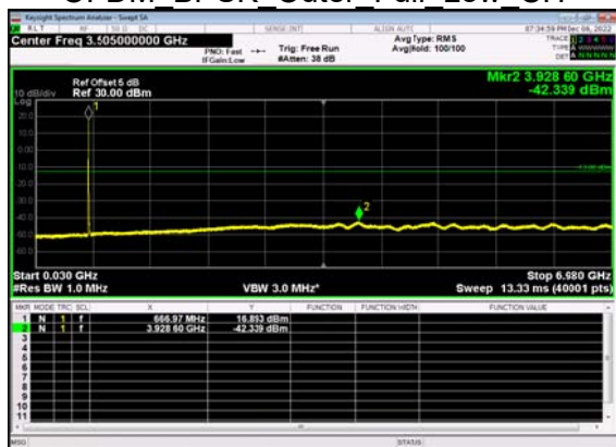
N71(5M)_DFT-s- OFDM BPSK Outer Full Low CH
