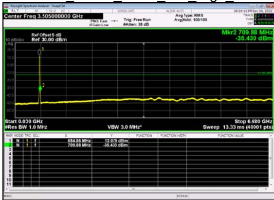
N71(15M)_DFT-s- OFDM QPSK Outer Full High CH
