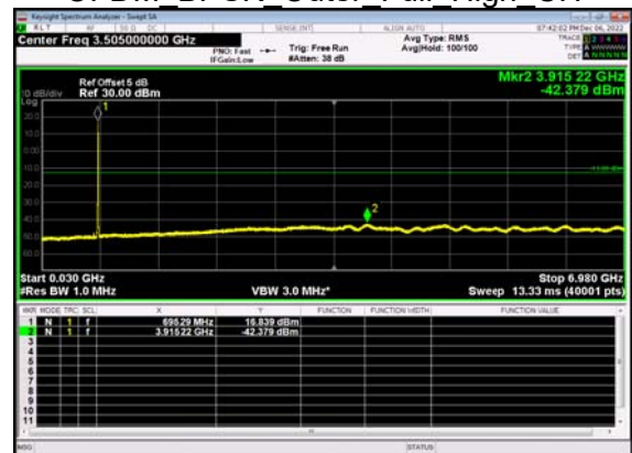
N71(5M)_DFT-s- OFDM BPSK Outer Full High CH
