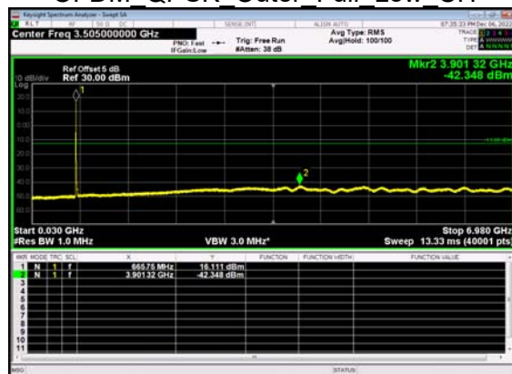
N71(5M)_DFT-s- OFDM QPSK Outer Full Low CH
