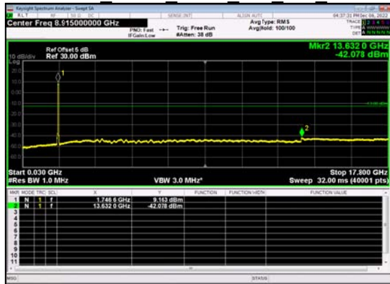
N66(30M)_DFT-s- OFDM BPSK Outer Full Mid CH
