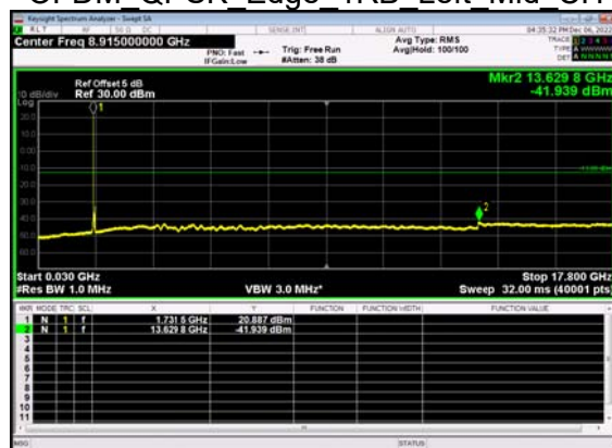
N66(30M)_DFT-s- OFDM QPSK Edge 1RB Left Mid CH
