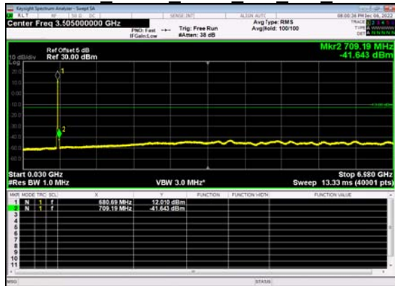
N71(15M)_DFT-s- OFDM QPSK Outer Full Mid CH
