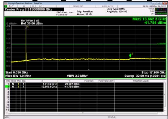
N66(30M)_DFT-s- OFDM QPSK Edge 1RB Left Low CH
