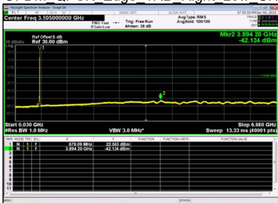
N71(15M)_DFT-s- OFDM QPSK Edge 1RB Right Low CH
