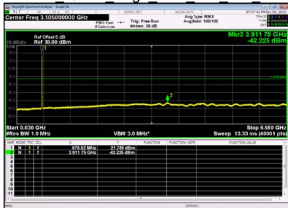
N71(10M)_DFT-s- OFDM QPSK Edge 1RB Left Mid CH
