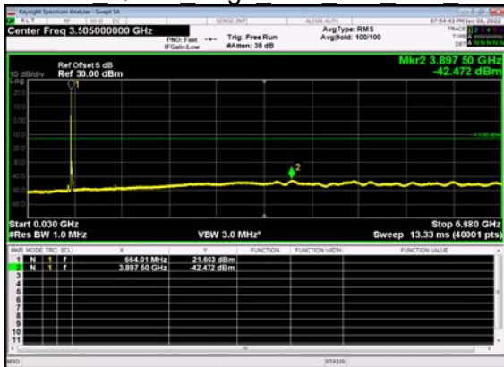
N71(15M)_DFT-s- OFDM QPSK Edge 1RB Left Low CH
