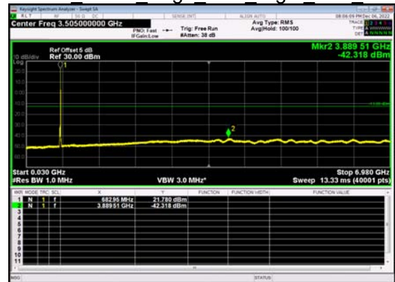
N71(20M)_DFT-s- OFDM BPSK Edge 1RB Right Low CH
