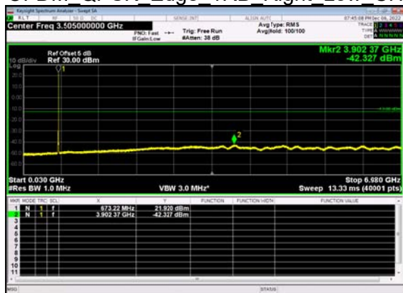
N71(10M)_DFT-s- OFDM QPSK Edge 1RB Right Low CH
