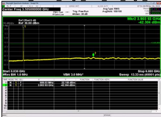
N71(10M)_DFT-s- OFDM QPSK Edge 1RB Left High CH
