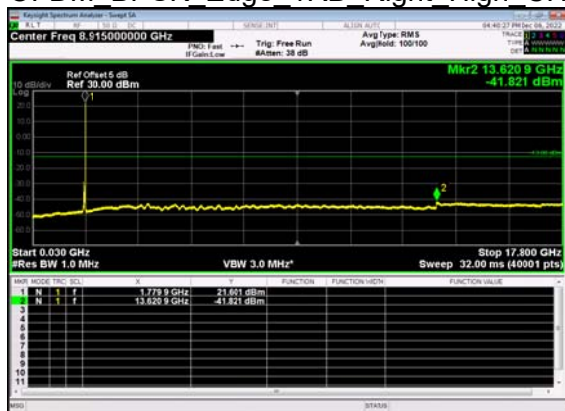
N66(30M)_DFT-s- OFDM BPSK Edge 1RB Right High CH
