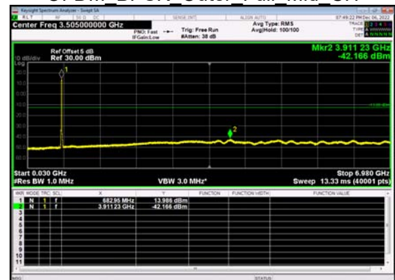
N71(10M)_DFT-s- OFDM BPSK Outer Full Mid CH
