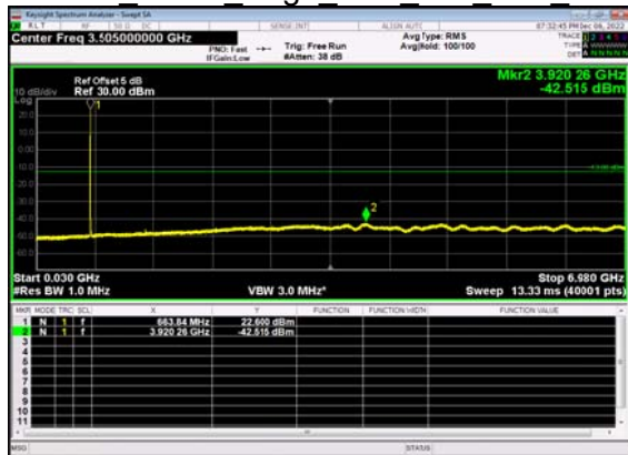
N71(5M)_DFT-s- OFDM BPSK Edge 1RB Left Low CH
