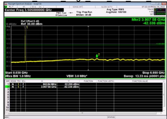
N71(5M)_DFT-s- OFDM QPSK Edge 1RB Left Low CH
