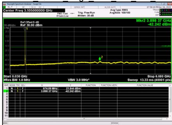
N71(15M)_DFT-s- OFDM QPSK Edge 1RB Left Mid CH
