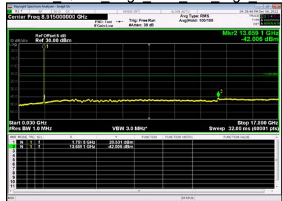
N66(30M)_DFT-s- OFDM QPSK Edge 1RB Left High CH
