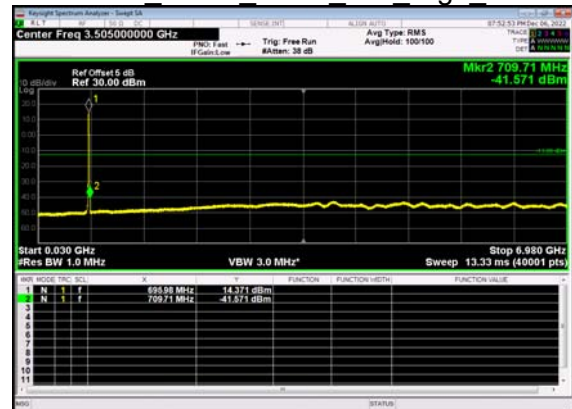
N71(10M)_DFT-s- OFDM BPSK Outer Full High CH
