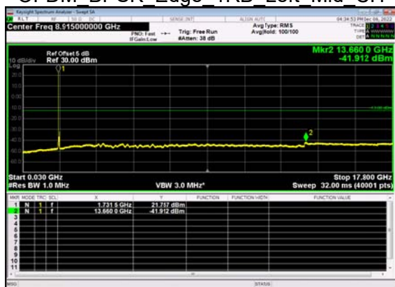
N66(30M)_DFT-s- OFDM BPSK Edge 1RB Left Mid CH
