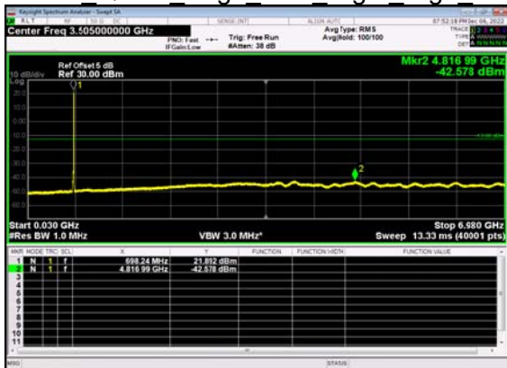
N71(10M)_DFT-s- OFDM QPSK Edge 1RB Right High CH
