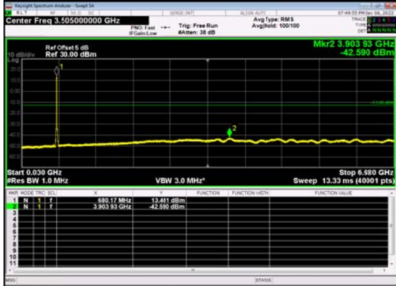
N71(10M)_DFT-s- OFDM QPSK Outer Full Mid CH
