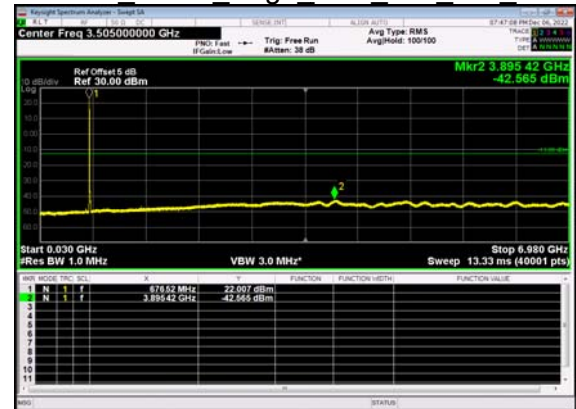
N71(10M)_DFT-s- OFDM BPSK Edge 1RB Left Mid CH
