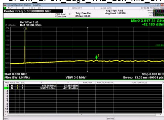
N71(5M)_DFT-s- OFDM QPSK Edge 1RB Left Mid CH
