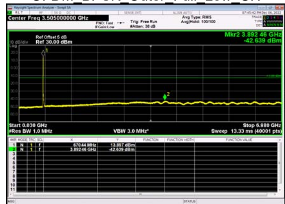
N71(10M)_DFT-s- OFDM BPSK Outer Full Low CH
