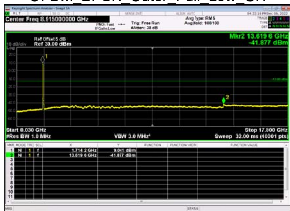
N66(30M)_DFT-s- OFDM BPSK Outer Full Low CH
