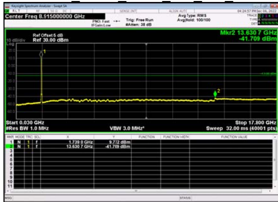
N66(25M)_DFT-s- OFDM BPSK Outer Full Mid CH
