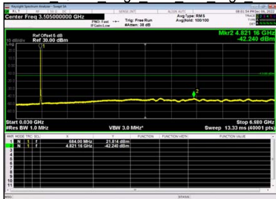
N71(15M)_DFT-s- OFDM QPSK Edge 1RB Left High CH
