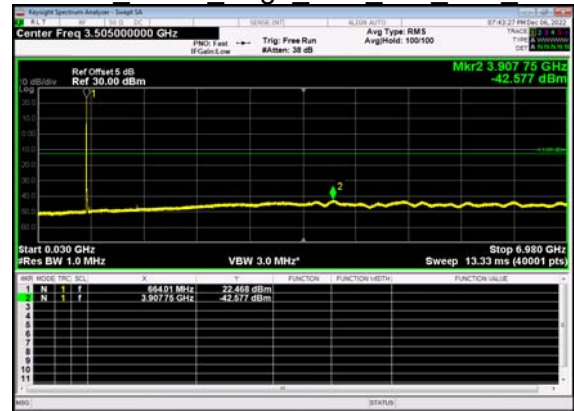
N71(10M)_DFT-s- OFDM BPSK Edge 1RB Left Low CH
