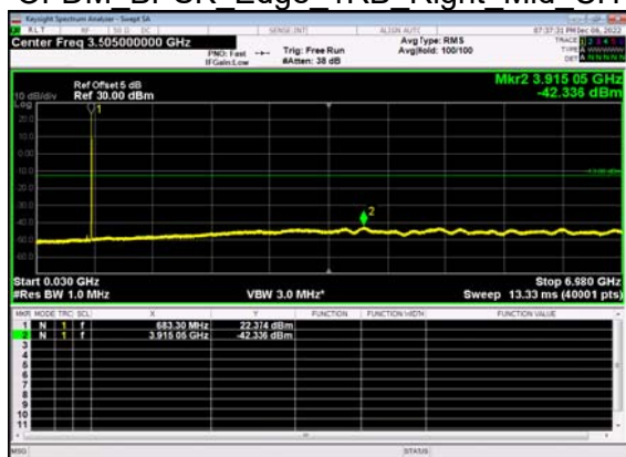
N71(5M)_DFT-s- OFDM BPSK Edge 1RB Right Mid CH
