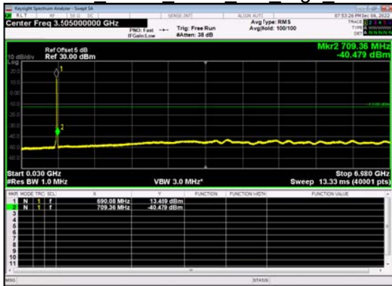
N71(10M)_DFT-s- OFDM QPSK Outer Full High CH
