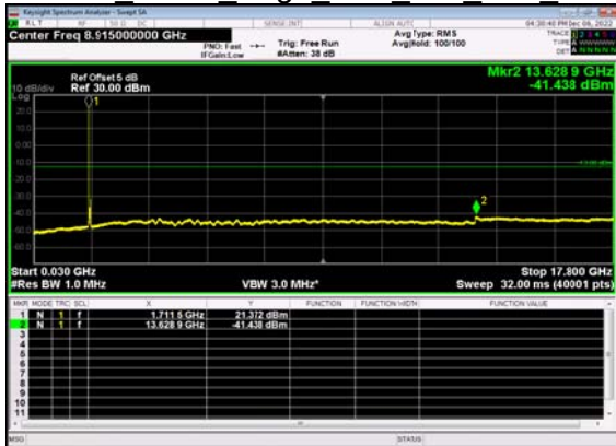
N66(30M)_DFT-s- OFDM BPSK Edge 1RB Left Low CH
