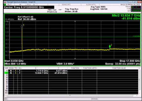
N66(25M)_DFT-s- OFDM QPSK Outer Full Low CH
