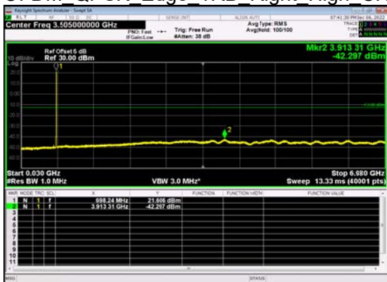
N71(5M)_DFT-s- OFDM QPSK Edge 1RB Right High CH
