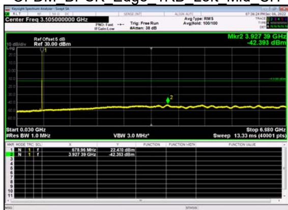
N71(5M)_DFT-s- OFDM BPSK Edge 1RB Left Mid CH
