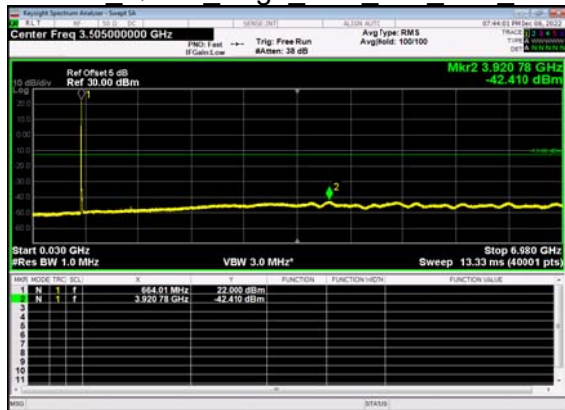
N71(10M)_DFT-s- OFDM QPSK Edge 1RB Left Low CH
