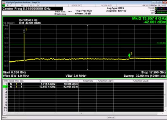
N66(25M)_DFT-s- OFDM BPSK Outer Full Low CH
