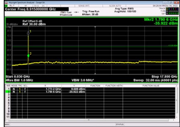
N66(25M)_DFT-s- OFDM QPSK Outer Full High CH
