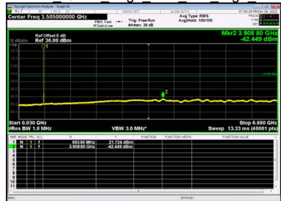
N71(5M)_DFT-s- OFDM QPSK Edge 1RB Left High CH
