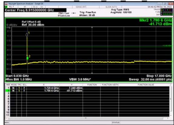
N66(40M)_DFT-s- OFDM QPSK Outer Full Low CH
