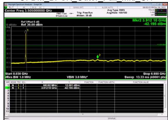
N71(15M)_DFT-s- OFDM BPSK Outer Full Mid CH
