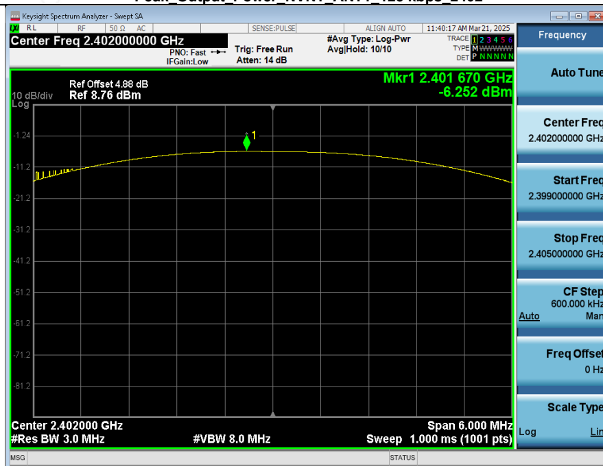
Peak_Output_Power_NVNT_ANT1_125 kbps_2402
