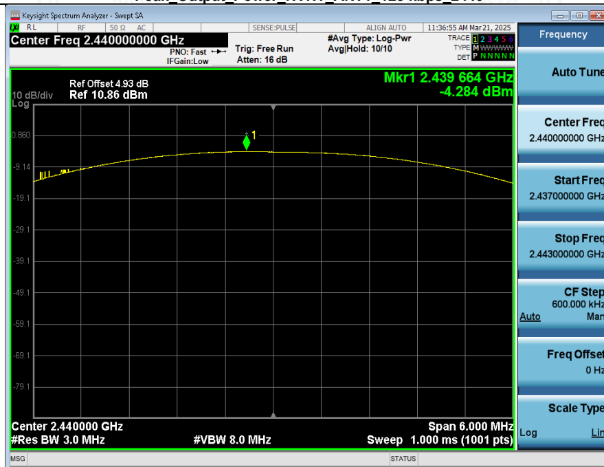
Peak_Output_Power_NVNT_ANT1_125 kbps_2440
