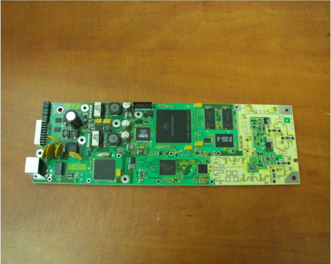
Outdoor Radio Unit PCB Top Side
