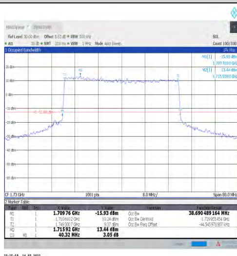
1-N66-15-40-L-8-CP-64QAM-Outer_Full-216@0-Ant 1-38.69-40.320-≤40-PASS
