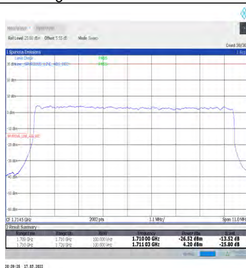
1-N66-15-10-L-3-DFT-PI2BPSK-Outer_Full-50@0-Ant1-seegraph-PASS-see graph
