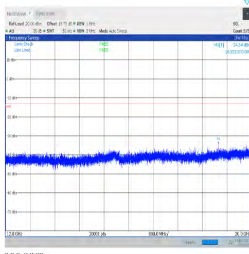
1-N66-15-40-M-1-DFT-PI2BPSK-Inner_1RB_Left-1@ 1-12000-20000-Ant1--34.54--13-PASS
