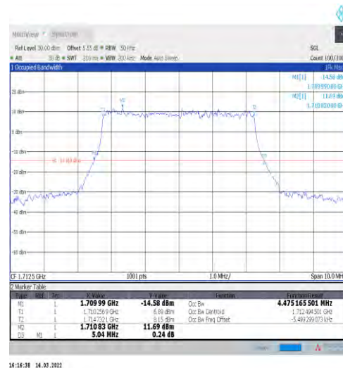
1-N66-15-5-L-4-DFT-64QAM-Outer_Full-25@0-Ant1-4 4.475-5.040-≤5-PASS
