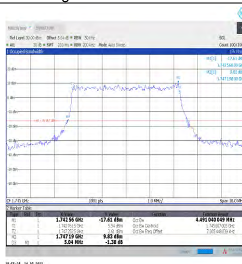
1-N66-15-5-M-5-DFT-256QAM-Outer_Full-25@0-Ant 1-4.491-5.040-≤5-PASS
