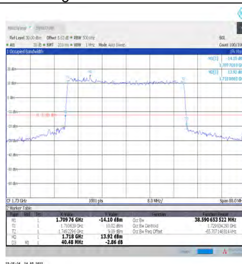
1-N66-15-40-L-7-CP-16QAM-Outer_Full-216@0-Ant 1-38.591-40.480-≤40-PASS
