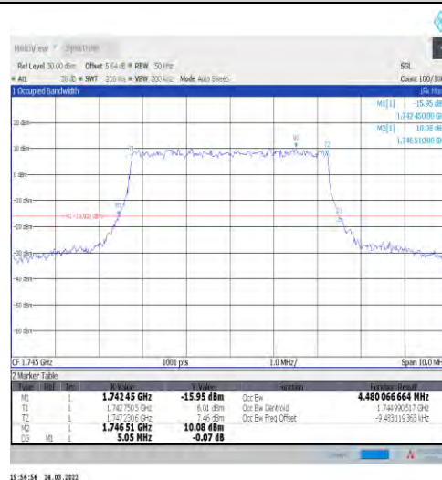
1-N66-15-5-M-7-CP-16QAM-Outer_Full-25@0-Ant1- 4.48-5.050-≤5-PASS
