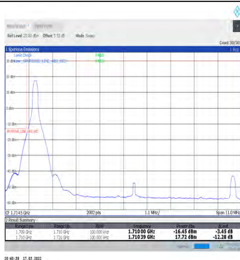
1-N66-15-10-L-4-CP-QPSK-Edge_1RB_Left-1@0-Ant1-seegraph-PASS-see graph
