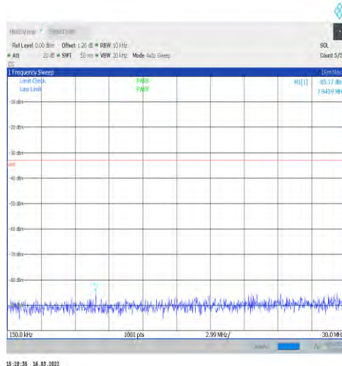
1-N66-15-40-M-1-DFT-PI2BPSK-Inner_1RB_Left-1@ 1-0.15-30-Ant1--85.17--33-PASS
