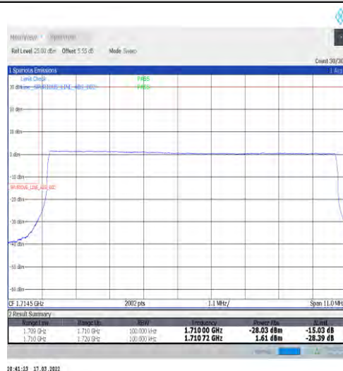
1-N66-15-10-L-6-CP-QPSK-Outer_Full-52@0-Ant1-seegraph-PASS-see graph
