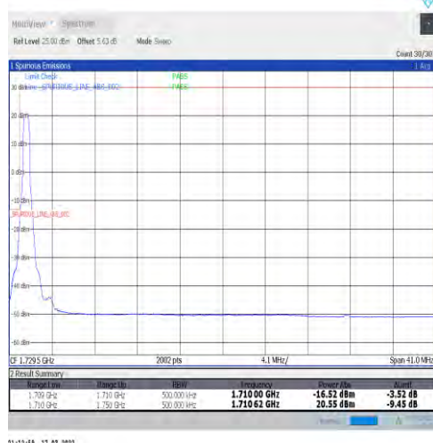
1-N66-15-40-L-4-CP-QPSK-Edge_1RB_Left-1@0-Ant1-seegraph-PASS-see graph
