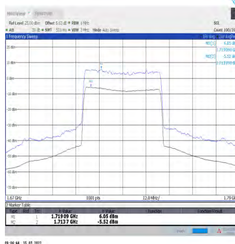
1-N66-15-40-L-2-CP-256QAM-Outer_Full-216@0-A nt1-11.57-100%-0.00-11.57-PASS-≤13
