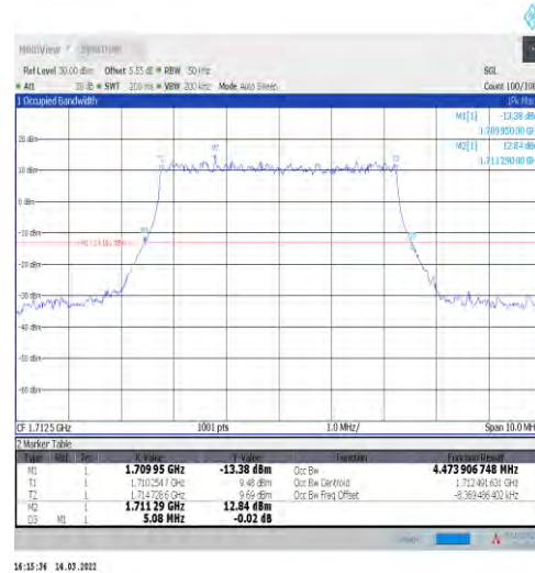
1-N66-15-5-L-2-DFT-PI2BPSK-Outer_Full-25@0-Ant1-4 1-4.474-5.080-≤5-PASS
