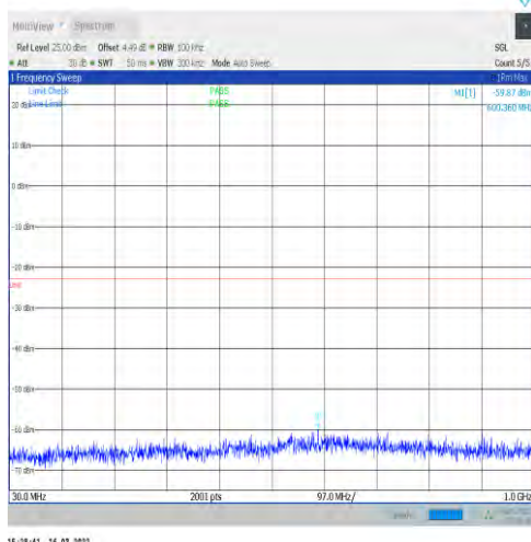
1-N66-15-40-M-1-DFT-PI2BPSK-Inner_1RB_Left-1 @1-30-1000-Ant1--59.87--23-PASS
