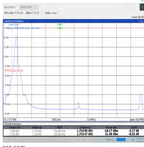
1-N66-15-15-L-1-DFT-PI2BPSK-Edge_1RB_Left-1@0-Ant1-seegraph-PASS-see graph
