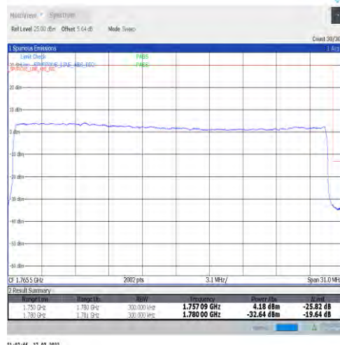
1-N66-15-30-H-3-DFT-PI2BPSK-Outer_Full-160@0-Ant1-seegraph-PASS-see graph
