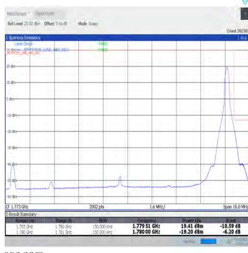
1-N66-15-15-H-5-CP-QPSK-Edge_1RB_Right-1@78-Ant1-seegraph-PASS-see graph
