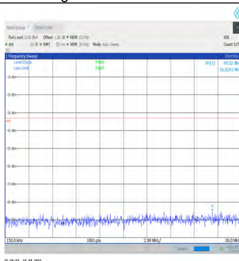
1-N66-15-40-H-1-DFT-PI2BPSK-Inner_1RB_Left-1@ 1-0.15-30-Ant1--85.52--33-PASS
