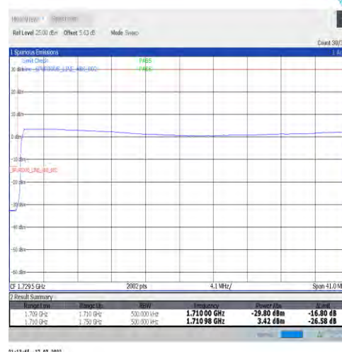
1-N66-15-40-L-6-CP-QPSK-Outer_Full-216@0-Ant1-seegraph-PASS-see graph
