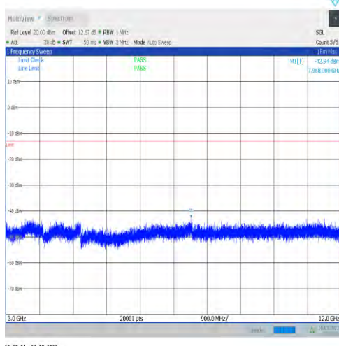
1-N66-15-40-M-1-DFT-PI2BPSK-Inner_1RB_Left-1 @1-3000-12000-Ant1--42.94--13-PASS
