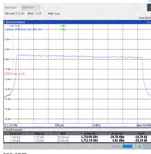
1-N66-15-15-L-3-DFT-PI2BPSK-Outer_Full-75@0-Ant1-seegraph-PASS-see graph
