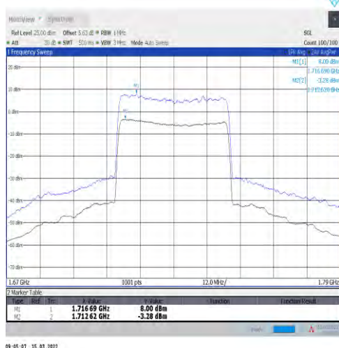
1-N66-15-40-L-1-DFT-256QAM-Outer_Full-216@0-A nt1-11.28-100%-0.00-11.28-PASS-≤13
