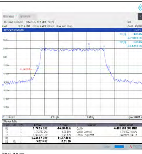
1-N66-15-5-M-4-DFT-64QAM-Outer_Full-25@0-Ant1 -4.484-5.070-≤5-PASS
