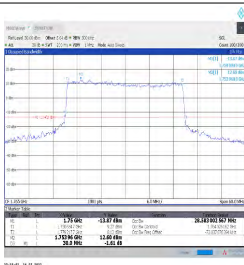
1-N66-15-30-H-7-CP-16QAM-Outer_Full-160@0-Ant 1-28.583-30.000-≤30-PASS
