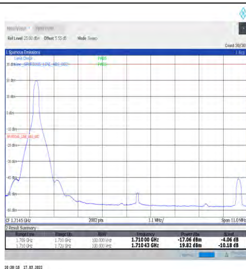
1-N66-15-10-L-1-DFT-PI2BPSK-Edge_1RB_Left-1@0-Ant1-seegraph-PASS-see graph
