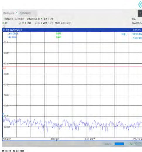
1-N66-15-40-M-1-DFT-PI2BPSK-Inner_1RB_Left-1 @ 1-0.009-0.15-Ant1--90.98--43-PASS
