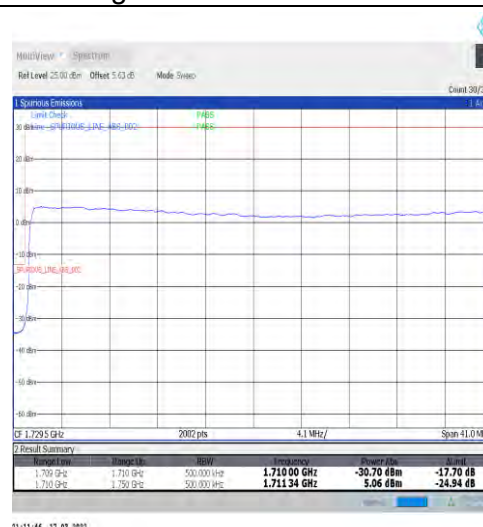
1-N66-15-40-L-3-DFT-PI2BPSK-Outer_Full-216@0-Ant1-seegraph-PASS-see graph
