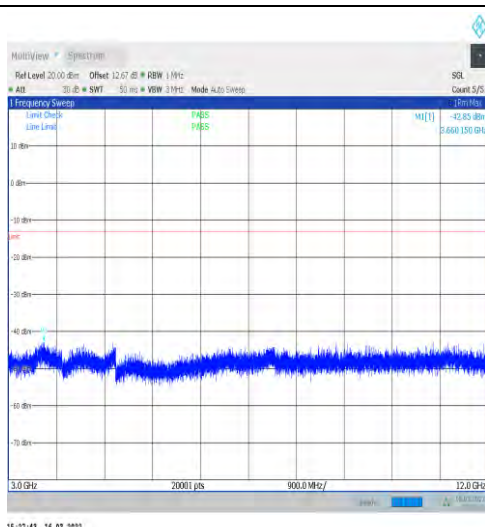
1-N66-15-40-L-1-DFT-PI2BPSK-Inner_1RB_Left-1@ 1-3000-12000-Ant1--42.85--13-PASS
