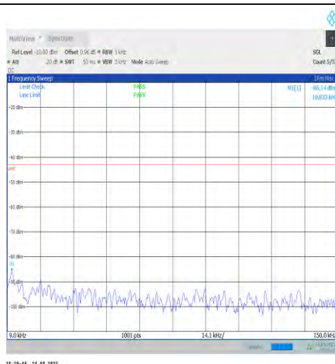
1-N66-15-40-H-1-DFT-PI2BPSK-Inner_1RB_Left-1 @1-0.009-0.15-Ant1--86.14--43-PASS
