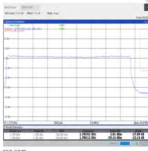
1-N66-15-15-H-3-DFT-PI2BPSK-Outer_Full-75@0-Ant1-seegraph-PASS-see graph
