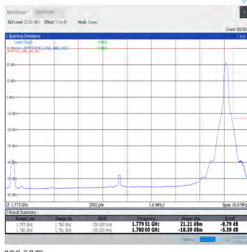
1-N66-15-15-H-2-DFT-PI2BPSK-Edge_1RB_Right-1@78-Ant1-seegraph-PASS-see graph
