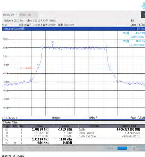
1-N66-15-5-L-3-DFT-16QAM-Outer_Full-25@0-Ant1-4 4.456-4.960-≤5-PASS
