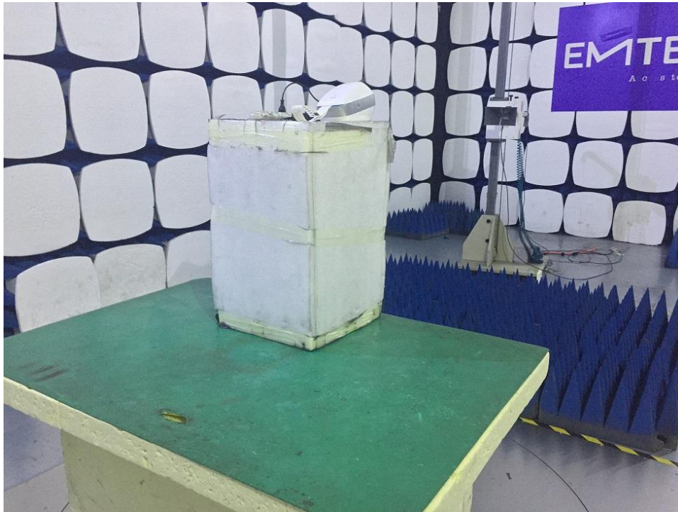
Photograph 4: Setup for Spurious emissions, Above 18GHz
