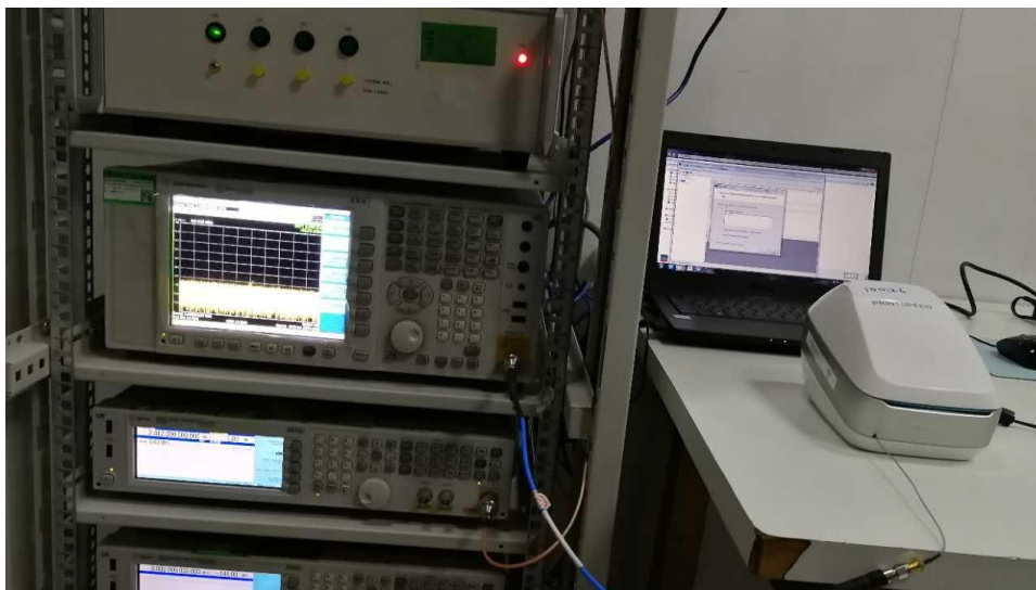
Photograph 2: Setup for Spurious emissions, 30MHz-1GHz
