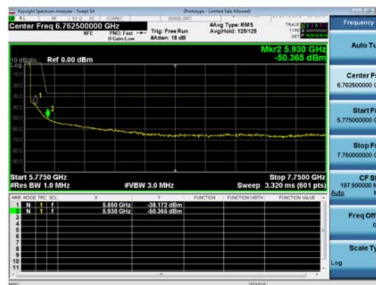
Antenna D
