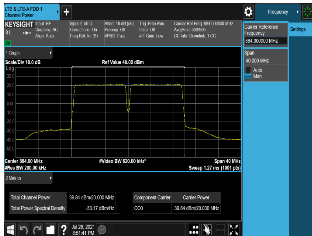
Plot 7-158. Conducted Average Output Power Plot (LTE_B5_10M+10M_2C_256QAM – High Channel, Port 0)
