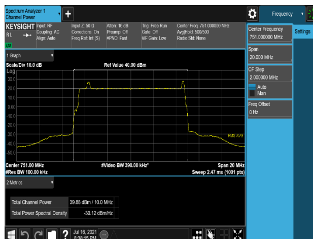
Plot 7-219. Conducted Average Output Power Plot (LTE B13 10M+High NB-IoT(GB)+Low NB-IoT(LB) 2C - Port 1)
