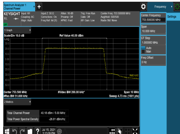
Plot 7-177. Conducted Average Output Power Plot (LTE_B13_5M_1C_64QAM - High Channel, Port 3)
