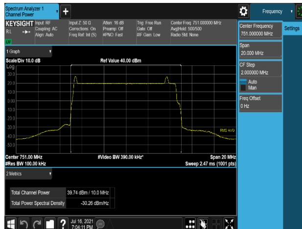
Plot 7-217. Conducted Average Output Power Plot (LTE B13 10M+Low NB-lot(GB)+High NB-lot(IB) 2C - Port 3)
