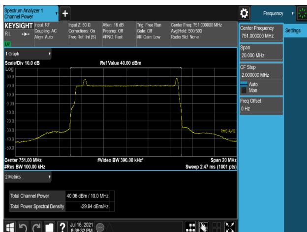
Plot 7-220. Conducted Average Output Power Plot (LTE B13 10M+High NB-IoT(GB)+Low NB-IoT(IB) 2C - Port 2)
