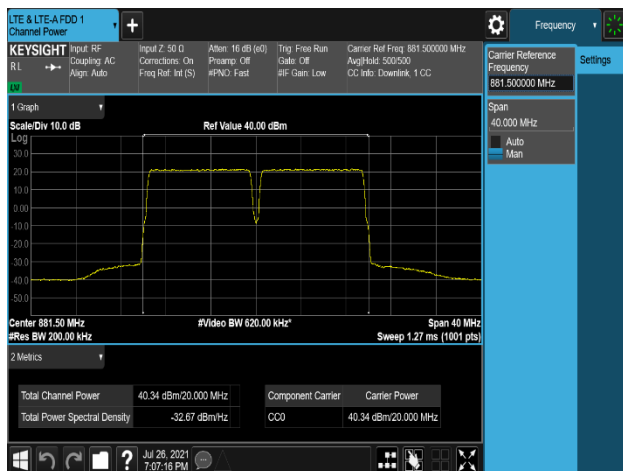
Plot 7-156. Conducted Average Output Power Plot (LTE_B5_10M+10M_2C_64QAM – Mid Channel, Port 2)
