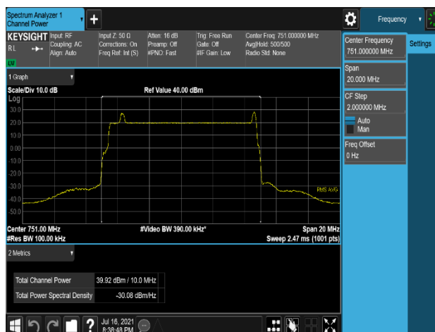
Plot 7-221. Conducted Average Output Power Plot (LTE B13 10M+High NB-Iot(GB)+Low NB-Iot(LB) 2C - Port 3)
