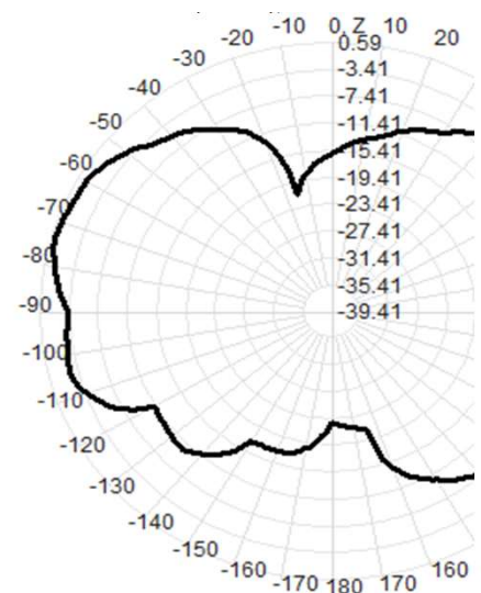
5290.0MHz Total(E2-YZ),Max=0.22dBi
