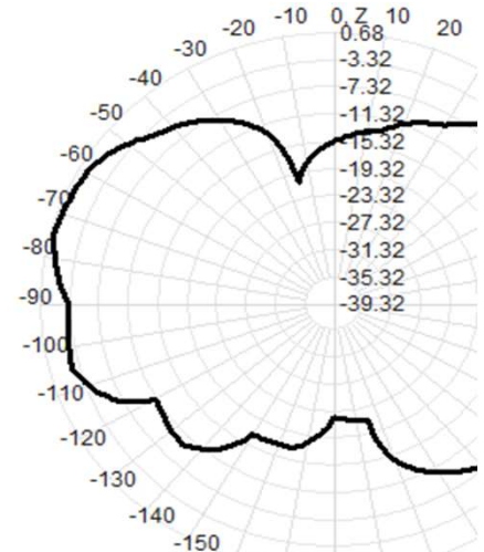
5290.0MHz Total(E2-YZ),Max=0.22dBi
