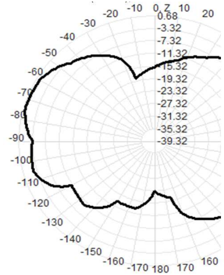
5280.0MHz Total(E2-YZ),Max=0.45dBi
