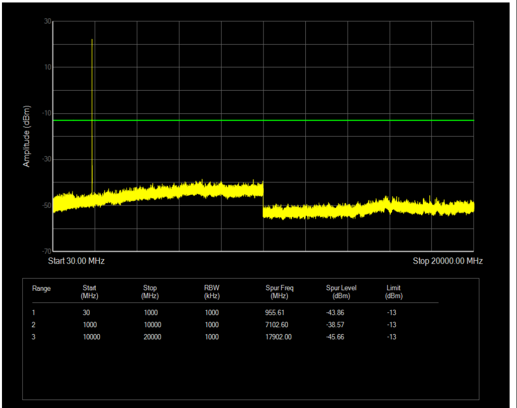
n2 SCS=15kHz DFT_BPSK BW=5MHz Channel=376000 RB=1@24
