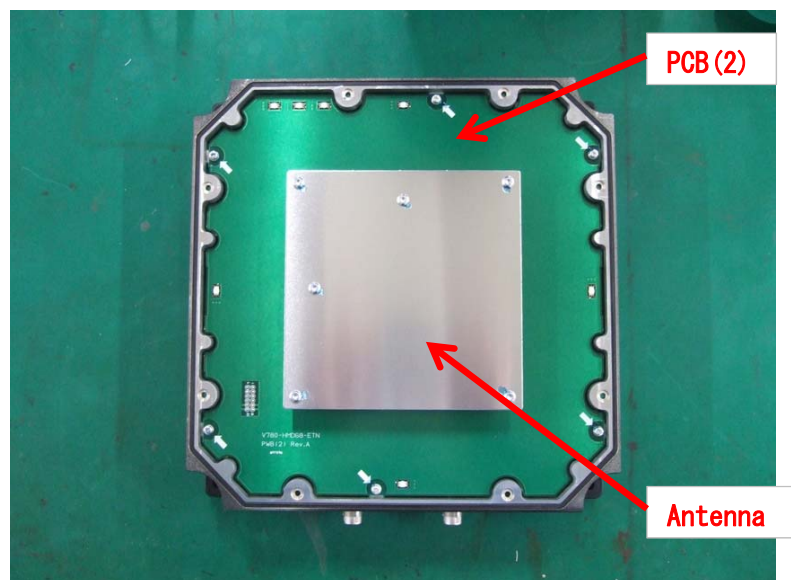
Fig. 20 PCB assembly No. 3
