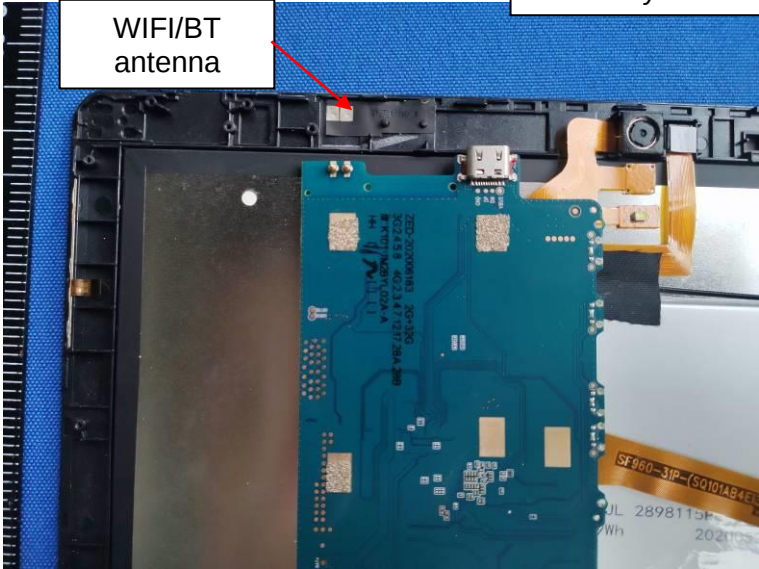
LTE Diversity antenna
