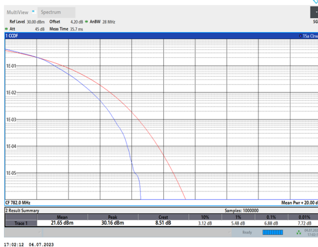
Band13-10MHz-16QAM-23230-27RB#0
