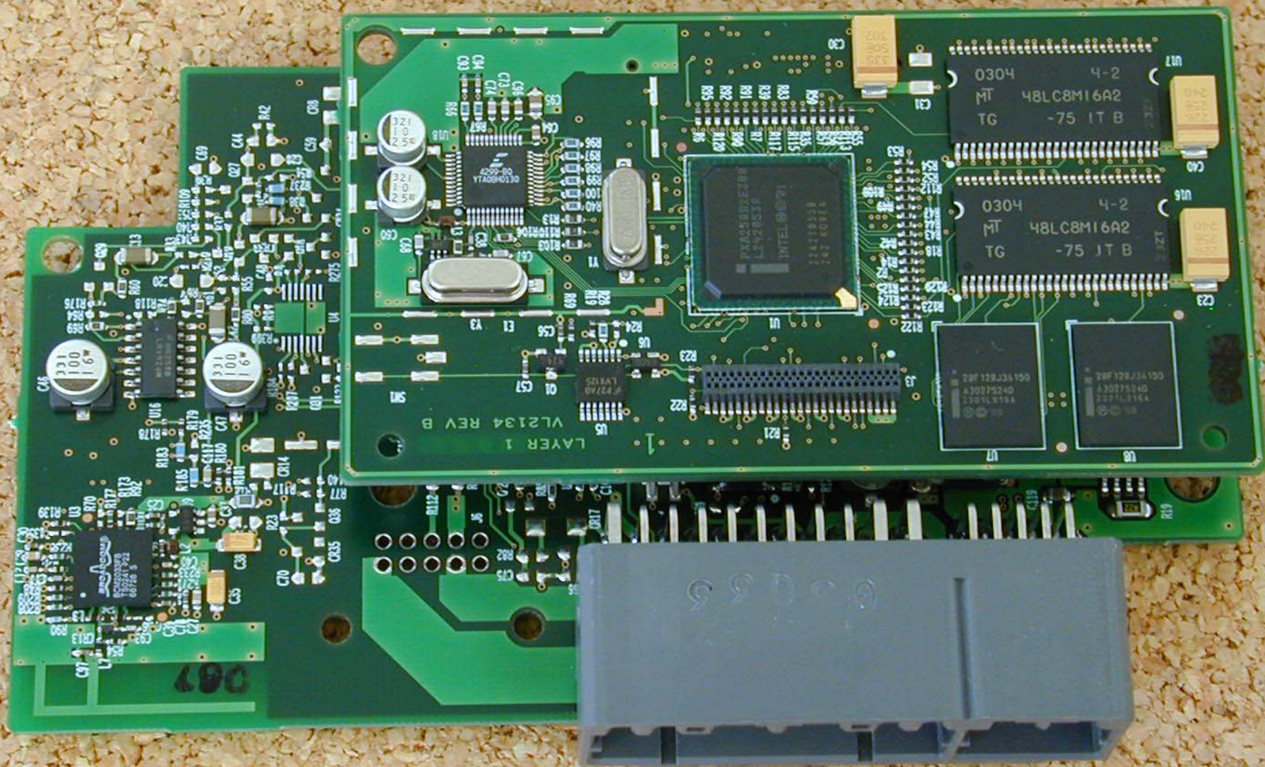
Module 56091004AC PCB (top)
