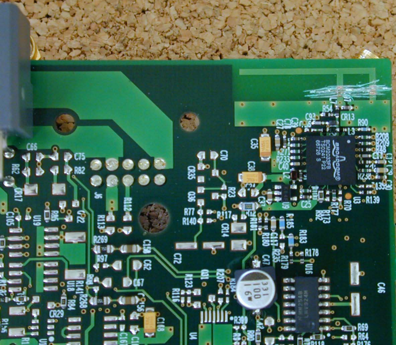
DUT with SMA Connector Attached (top)
