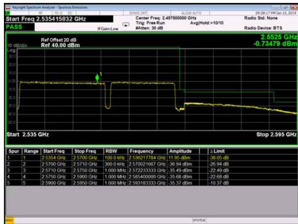
LowRange_FDD07_20+20MHz_1RB0 and 1RB99 QPSK
