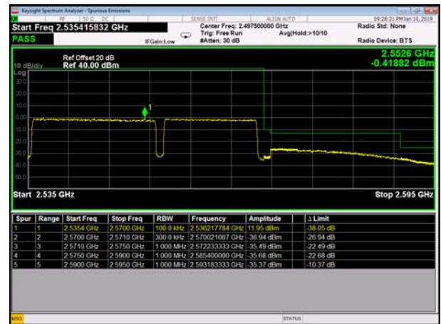
LowRange_FDD07_20+20MHz_1RB0 and 1RB99 Q16
