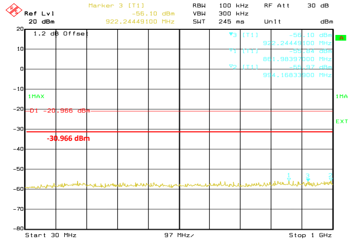
Date: 21.DEC.2016 10:03:16 Conducted Emissions. 802.11n, Frequency 2412 MHz Emission Level, 30 MHz -> 1 GHz
