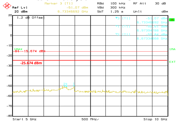
Conducted Emissions. 802.11b, Frequency 2412 MHz Emission Level, 5 GHz -> 10 GHz
