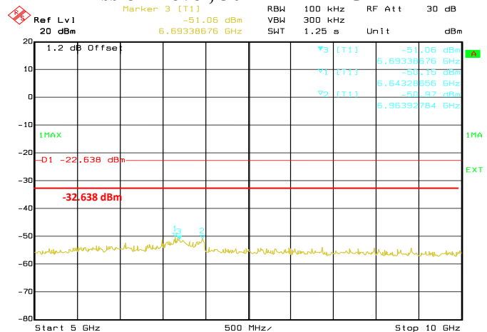
Date: 21.DEC.2016 09:45:25 Conducted Emissions. 802.11g, Frequency 2412 MHz Emission Level, 5 GHz -> 10 GHz
