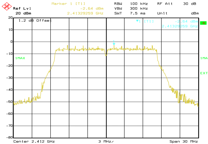
Date: 21.DEC.2016 09:43:46 Conducted Emissions. 802.11g, Frequency 2412 MHz Reference Level
