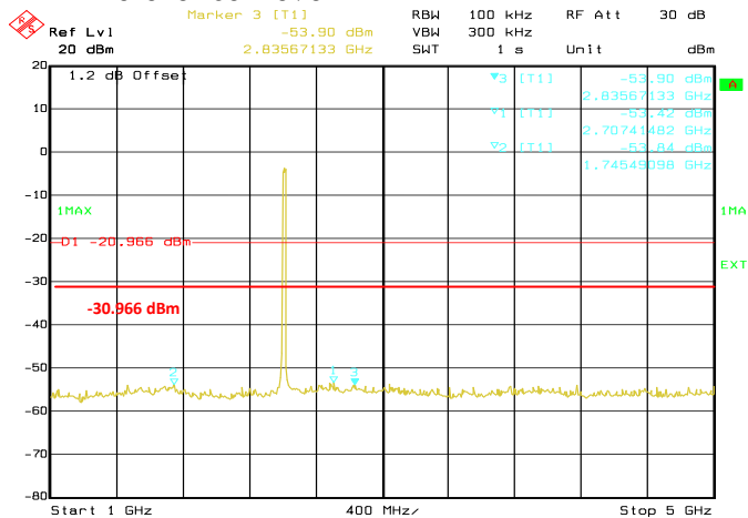
Date: 21.DEC.2016 10:03:49 Conducted Emissions. 802.11n, Frequency 2412 MHz Emission Level, 1 GHz -> 5 GHz
