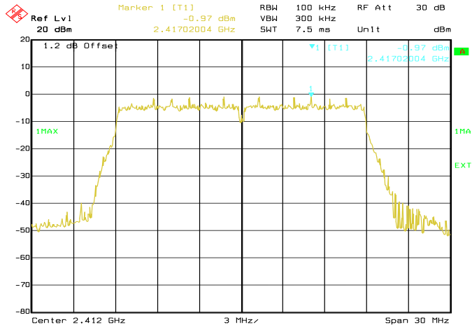
Date: 21.DEC.2016 10:02:43 Conducted Emissions. 802.11n, Frequency 2412 MHz Reference Level
