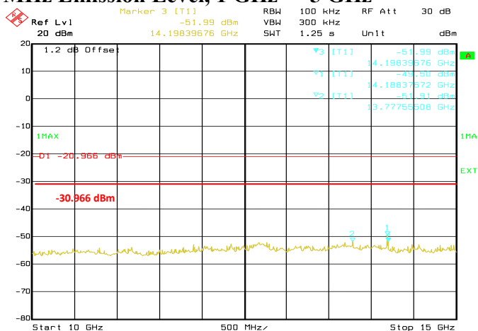
Date: 21.DEC.2016 10:04:54 Conducted Emissions. 802.11n, Frequency 2412 MHz Emission Level, 10 GHz -> 15 GHz
