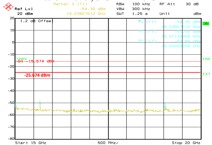
Conducted Emissions. 802.11b, Frequency 2412 MHz Emission Level, 15 GHz -> 20 GHz
