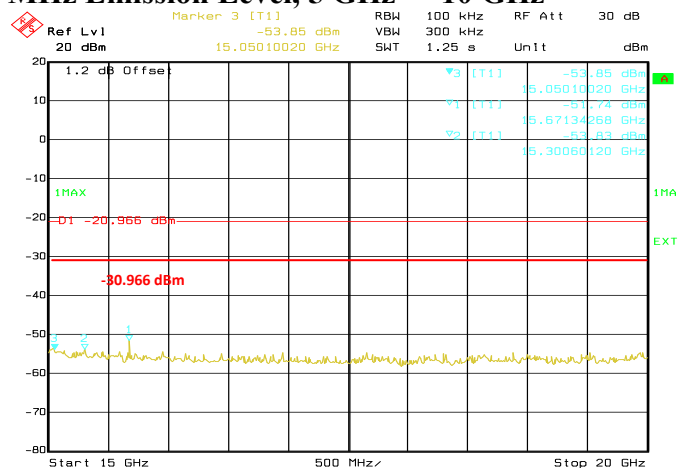
Date: 21.DEC.2016 10:05:27 Conducted Emissions. 802.11n, Frequency 2412 MHz Emission Level, 15 GHz -> 20 GHz
