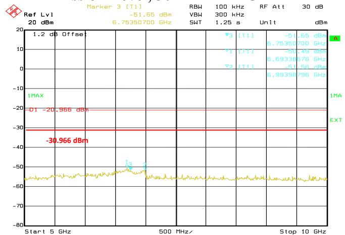
Date: 21.DEC.2016 10:04:21 Conducted Emissions. 802.11n, Frequency 2412 MHz Emission Level, 5 GHz -> 10 GHz
