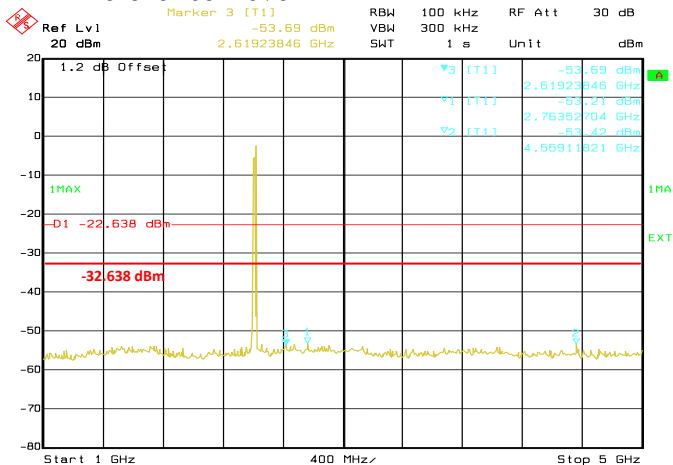
Date: 21.DEC.2016 09:44:52 Conducted Emissions. 802.11g, Frequency 2412 MHz Emission Level, 1 GHz -> 5 GHz
