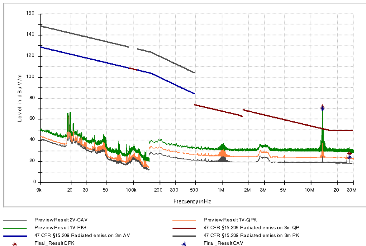
Figure 13: Chart of emissions test below 30 MHz, EUT position Y, without tag, antenna in line at 3 m
