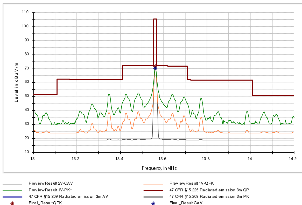
Figure 12: Chart of emission within the band 13.110 MHz to 14.010 MHz, EUT in position Y, without tag, antenna in line at 3 m distance
