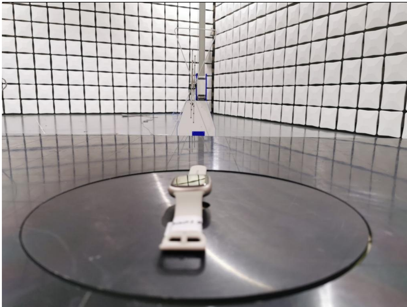
RE (30MHz~1GHz)
