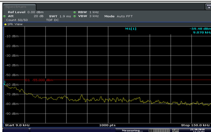
Band38-20MHz-QPSK-38000-100RB#0-Range1:0.009~0.15MHz
