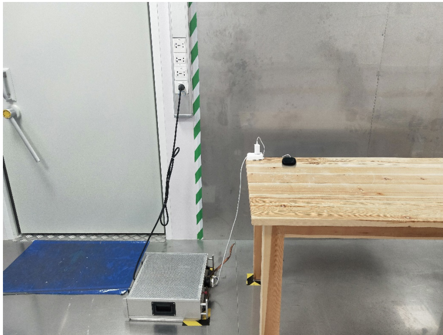
FCC ID: 2AJQ7LIGHTNING Photo of Conducted Emission Measurement
