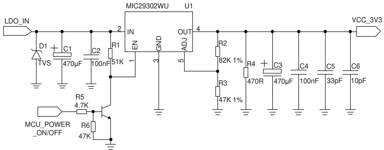
Figure 2: Reference Circuit of Power Supply
