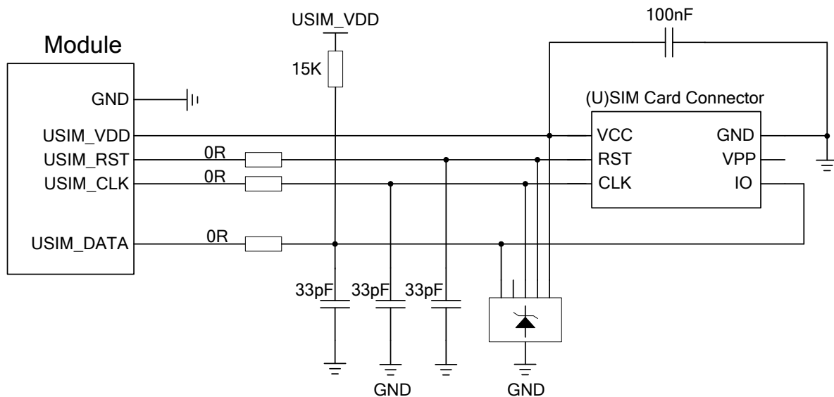
Figure 4: Reference Circuit of (U)SIM Interface with a 6-pin (U)SIM Card Connector
