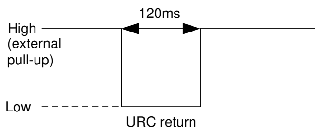
Figure 13: WAKE# Behavior
