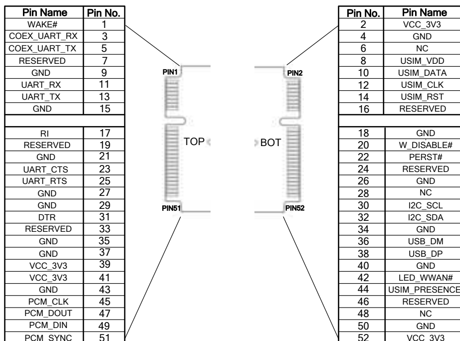
Figure 1: Pin Assignment
