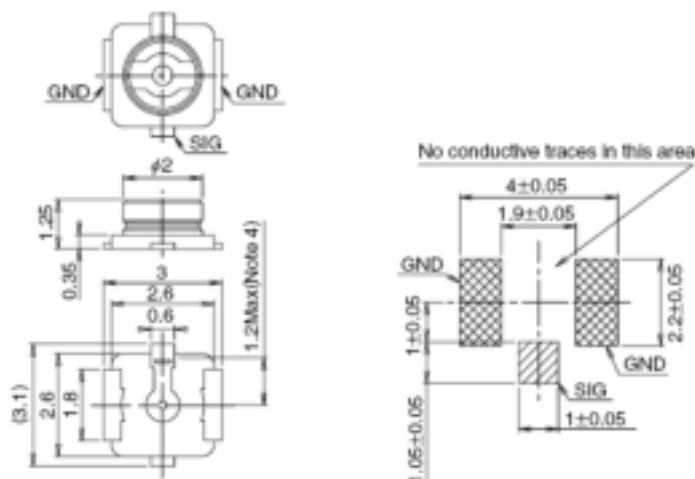
Figure 14: Dimensions of the Receptacle RF Connectors (Unit: mm)
