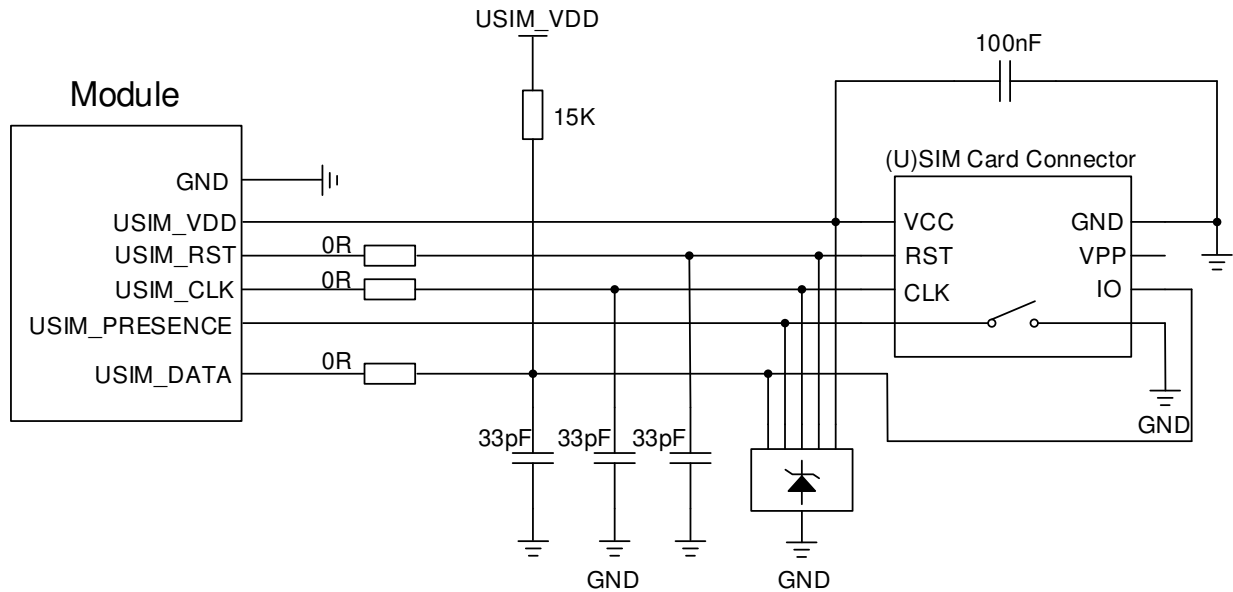
Figure 3: Reference Circuit of (U)SIM Interface with an 8-pin (U)SIM Card Connector
