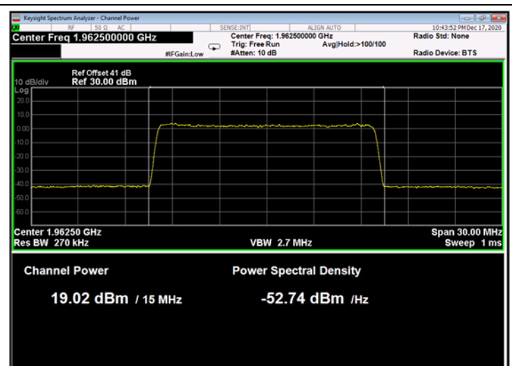
Figure 160: 256QAM 15MHz B.W.; 1962.5MHz, 30kHz
