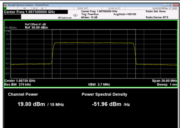
Figure 162: 256QAM 15MHz B.W.; 1987.5MHz, 15kHz
