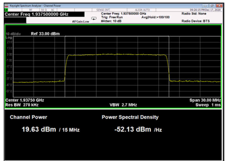
Figure 90: 64QAM 15MHz B.W.; 1937.5MHz, 15kHz
