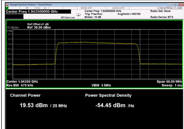
Figure 175: 256QAM 25MHz B.W.; 1942.5MHz, 30kHz
