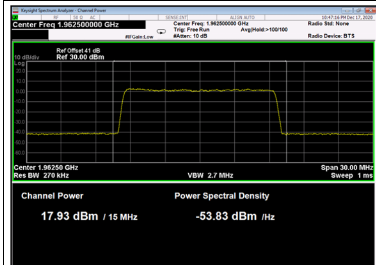
Figure 161: 256QAM 15MHz B.W.; 1962.5MHz, 60kHz
