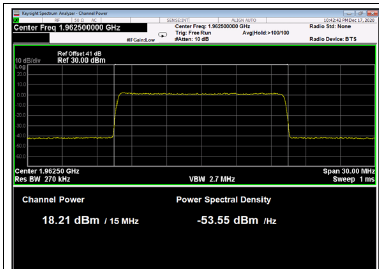
Figure 159: 256QAM 15MHz B.W.; 1962.5MHz, 15kHz
