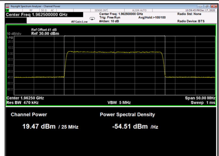
Figure 178: 256QAM 25MHz B.W.; 1962.5MHz, 30kHz
