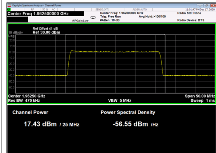
Figure 179: 256QAM 25MHz B.W.; 1962.5MHz, 60kHz
