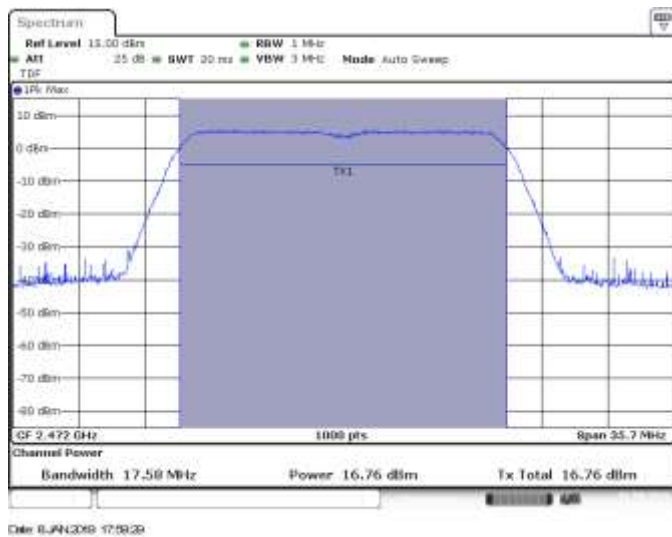
MIMO B, CH13, 802.11n20, HT8
