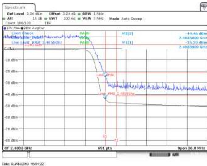
MIMO B, CH11, 802.11he40, HE0, BE High (Restricted)
