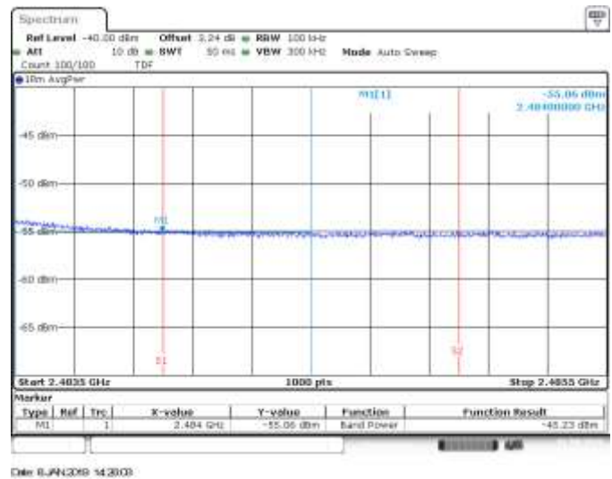
SISO B, CH11, 802.11he40, HE0, BE High RMS within 2MHz (Restricted)
