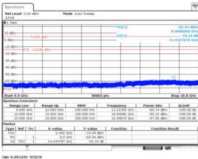
CH7, 802.11n20, HT8, MIMO B, Range 9GHz to 18GHz - Delta Marker Measurement
