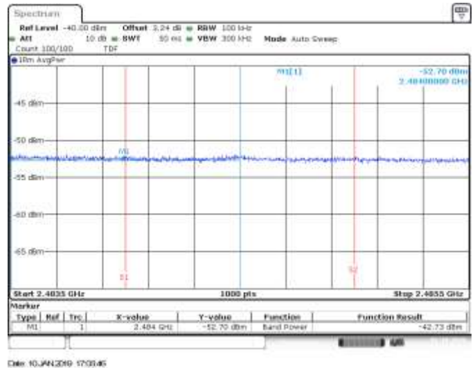
SISO A, CH9, 802.11he40, HE0, BE High RMS within 2MHz (Restricted)
