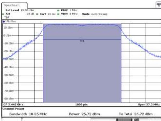
MIMO A, CH7, 802.11n20, HT8
