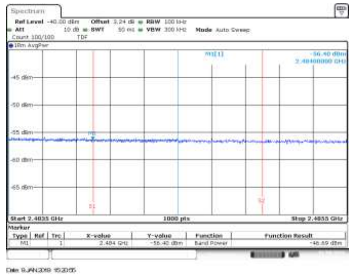
MIMO B, CH9, 802.11he40, HE0, BE High RMS within 2MHz (Restricted)
