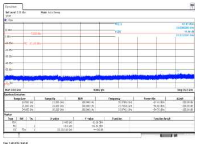
CH7, 802.11n20, HT0, SISO B, Range 18GHz to 26.5GHz - Delta Marker Measurement
