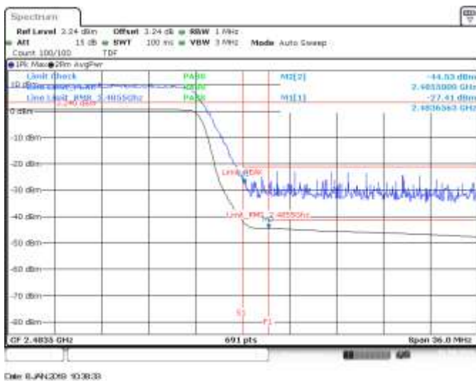
SISO B, CH11, 802.11n40, HT0, BE High (Restricted)
