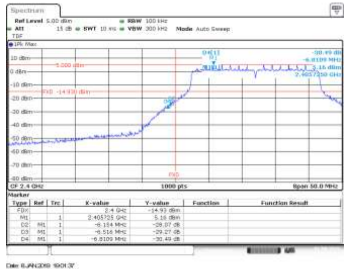
MIMO B, CH1, 802.11he20, HE0, BE Low (Non Restricted)
