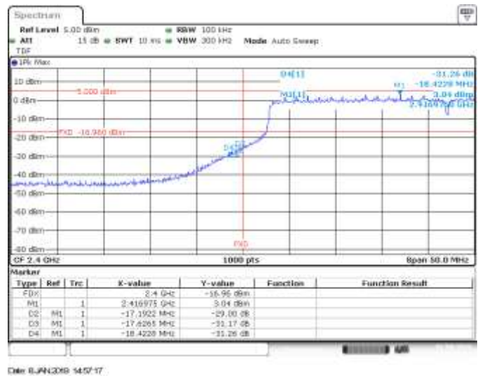
SISO B, CH3, 802.11he40, HE0, BE Low (Non Restricted)
