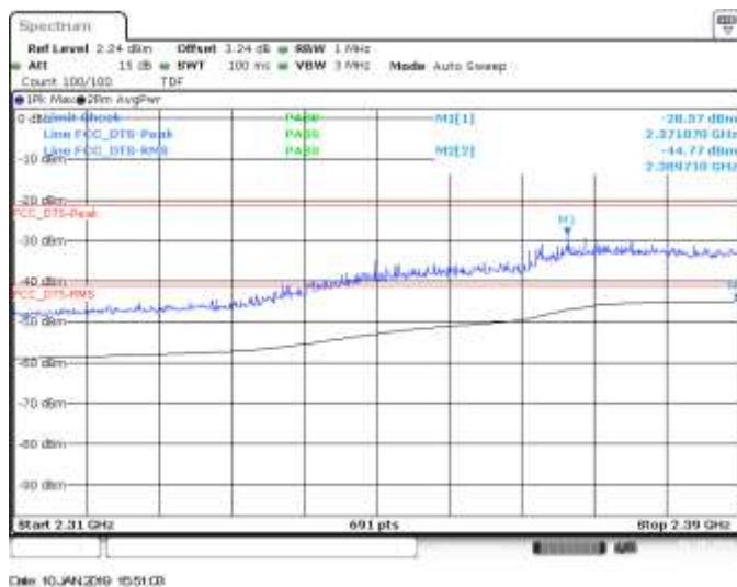
MIMO A, CH3, 802.11he40, HE0, BE Low
