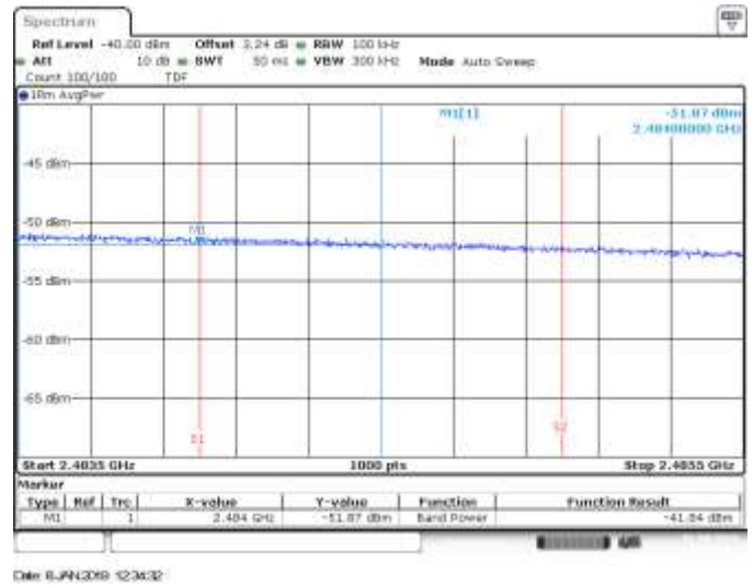
SISO B, CH11, 802.11he20, HE0, BE High RMS within 2MHz (Restricted)
