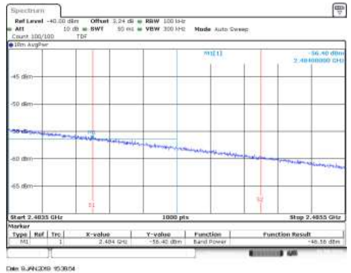
MIMO B, CH10, 802.11he40, HE0, BE High RMS within 2MHz (Restricted)
