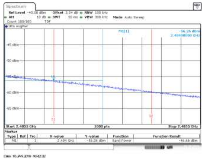
MIMO A, CH10, 802.11he40, HE0, BE High RMS within 2MHz (Restricted)
