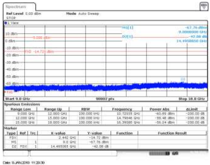
CH7, 802.11he20, HE0, MIMO A, Range 9GHz to 18GHz - Delta Marker Measurement
