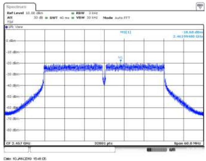
MIMO A, CH10, 802.11n40, HT8
