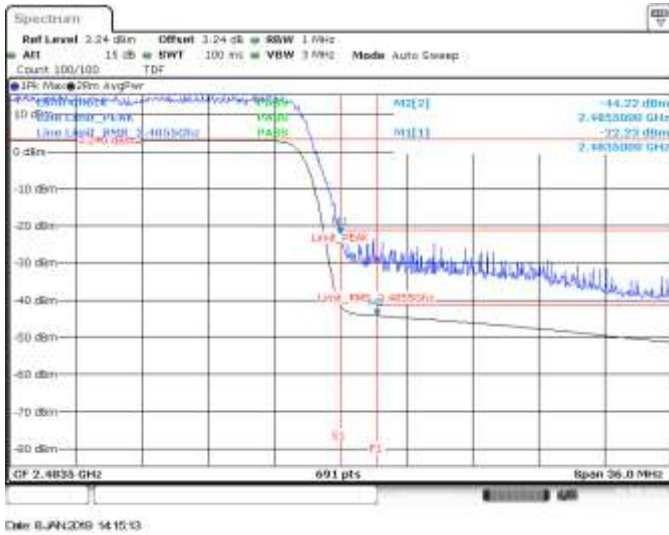
SISO B, CH13, 802.11he20, HE0, BE High (Restricted)
