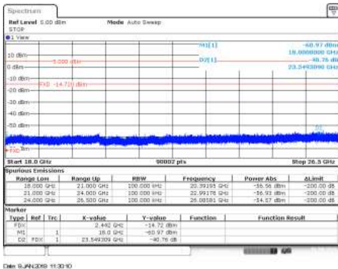
CH7, 802.11he20, HE0, MIMO A, Range 18GHz to 26.5GHz - Delta Marker Measurement
