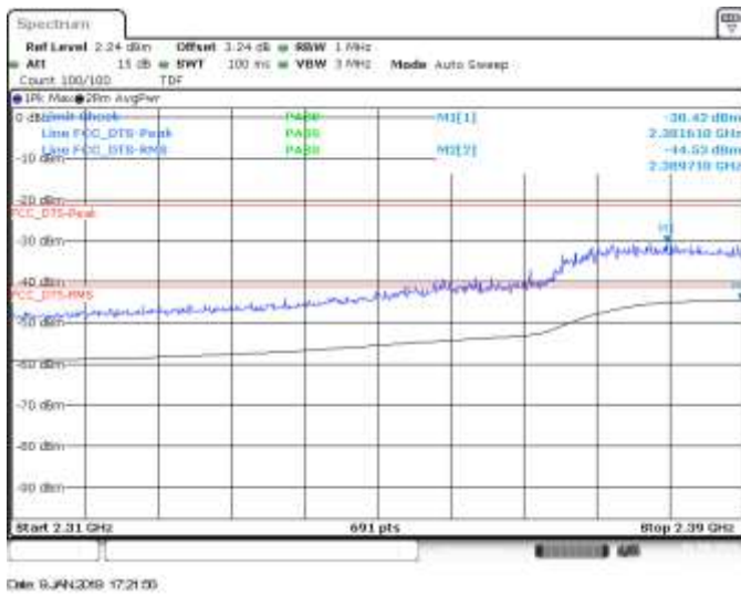
MIMO A, CH3, 802.11n40, HT8, BE Low
