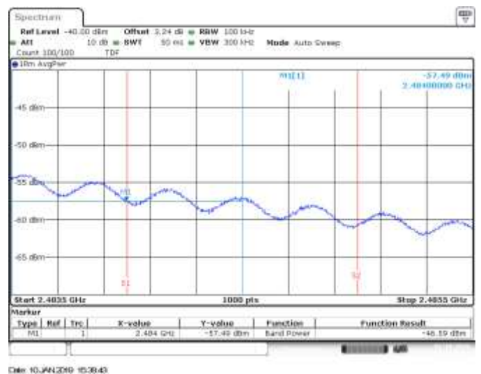
MIMO A, CH10, 802.11n40, HT8, BE High RMS within 2MHz (Restricted)
