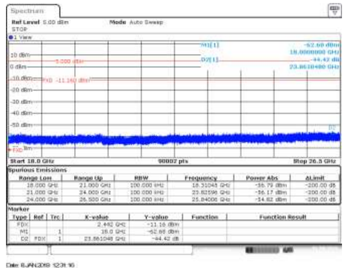
CH7, 802.11he20, HE0, SISO B, Range 18GHz to 26.5GHz - Delta Marker Measurement
