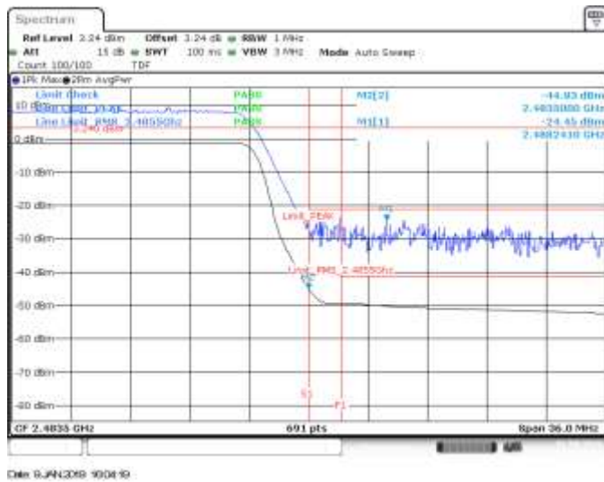
MIMO B, CH11, 802.11n40, HT8, BE High (Restricted)
