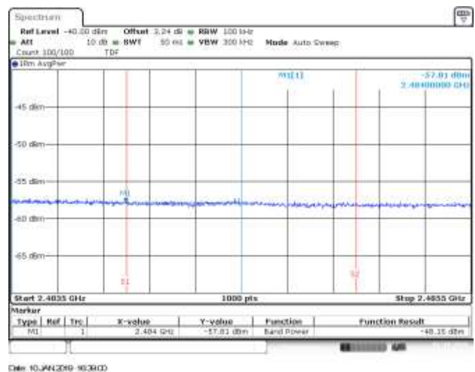
MIMO A, CH9, 802.11he40, HE0, BE High RMS within 2MHz (Restricted)
