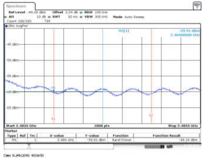
MIMO B, CH11, 802.11n40, HT8, BE High RMS within 2MHz (Restricted)
