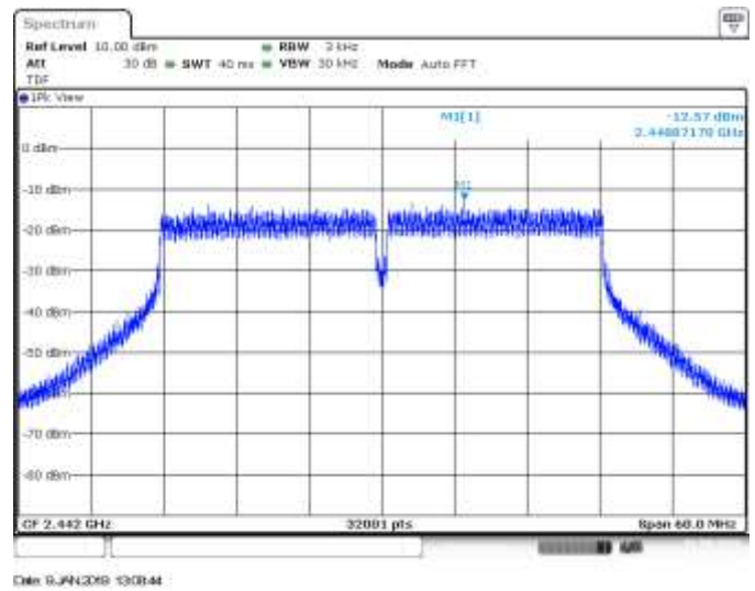
MIMO B, CH7, 802.11n40, HT8
