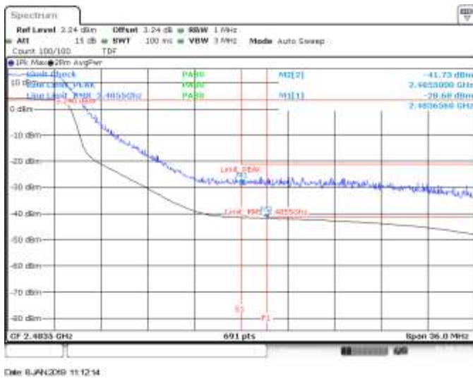
SISO B, CH9, 802.11n40, HT0, BE High (Restricted)
