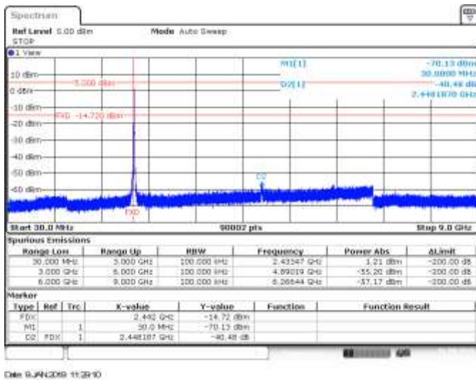
CH7, 802.11he20, HE0, MIMO A, Range 30MHz to 9GHz - Delta Marker Measurement
