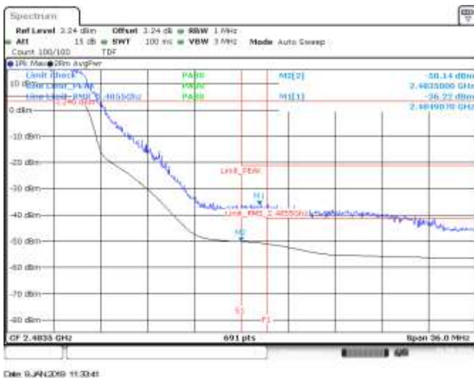
MIMO A, CH11, 802.11he20, HE0, BE High (Restricted)
