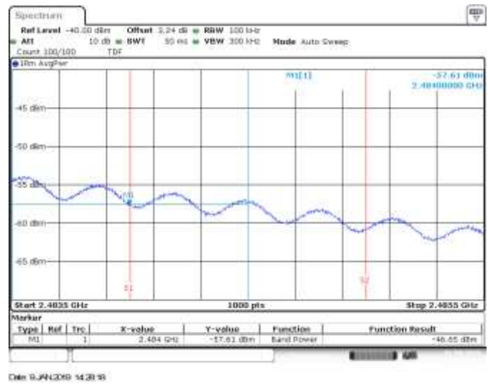
MIMO B, CH10, 802.11n40, HT8, BE High RMS within 2MHz (Restricted)
