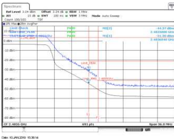
MIMO A, CH10, 802.11n40, HT8, BE High (Restricted)
