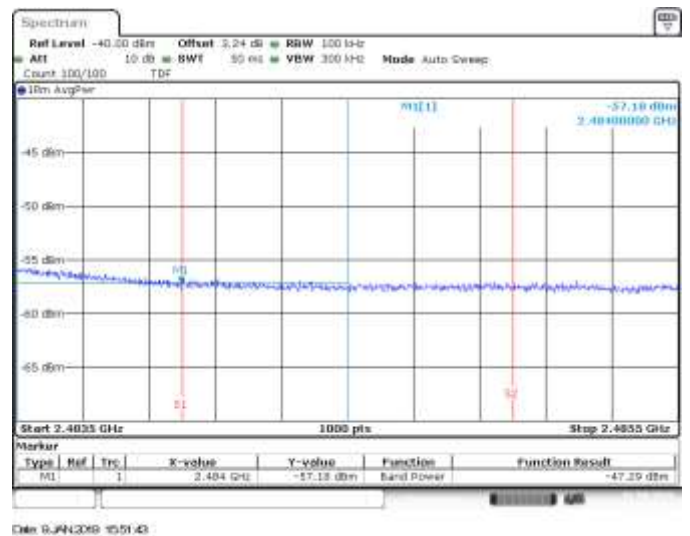
MIMO B, CH11, 802.11he40, HE0, BE High RMS within 2MHz (Restricted)
