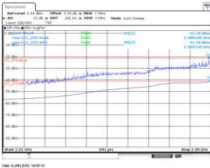
SISO B, CH3, 802.11he40, HE0, BE Low
