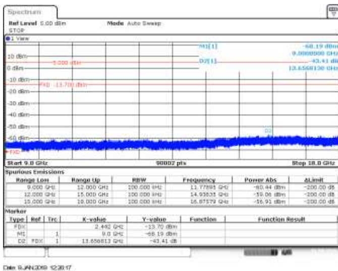
CH7, 802.11he20, HE0, MIMO B, Range 9GHz to 18GHz - Delta Marker Measurement
