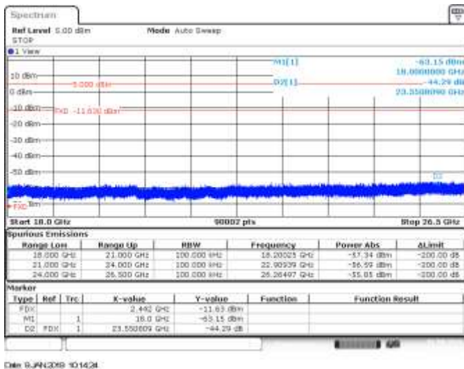
CH7, 802.11n20, HT8, MIMO A, Range 18GHz to 26.5GHz - Delta Marker Measurement
