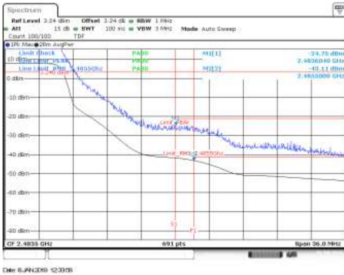
SISO B, CH11, 802.11he20, HE0, BE High (Restricted)
