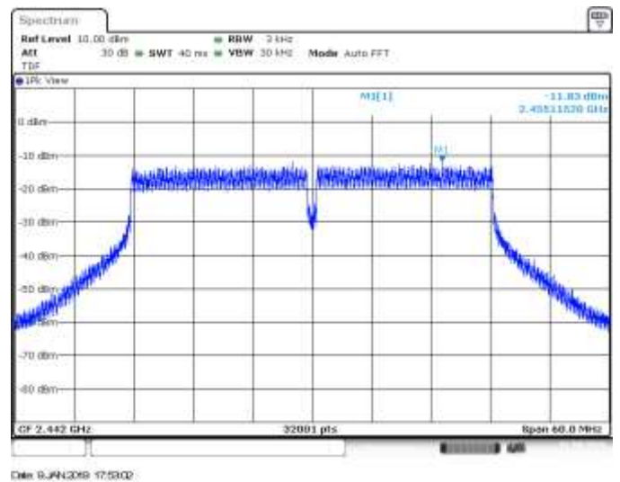
MIMO A, CH7, 802.11n40, HT8
