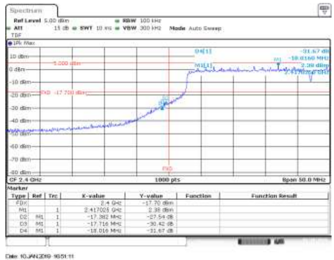
SISO A, CH3, 802.11he40, HE0, BE Low (Non Restricted)
