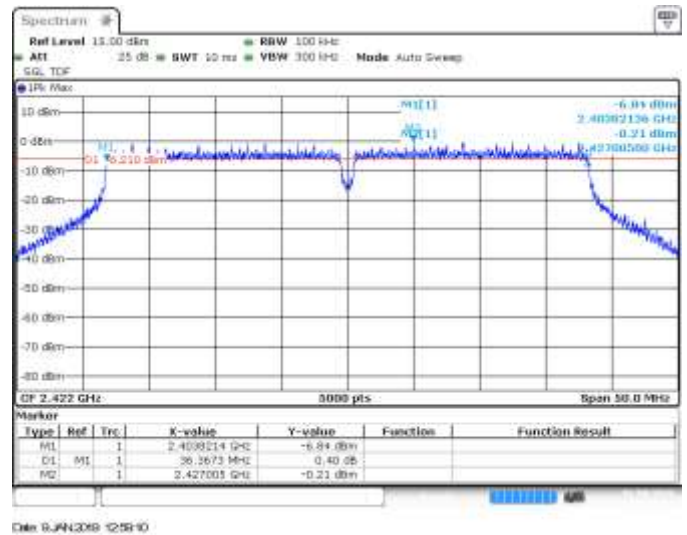
MIMO B, CH3, 802.11n40, HT8, 6dB
