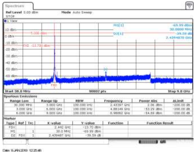
CH7, 802.11he20, HE0, MIMO B, Range 30MHz to 9GHz - Delta Marker Measurement
