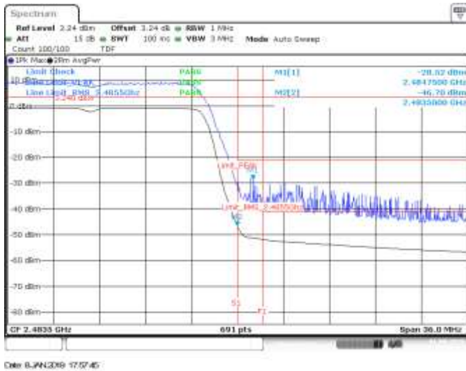
MIMO B, CH13, 802.11n20, HT8, BE High (Restricted)
