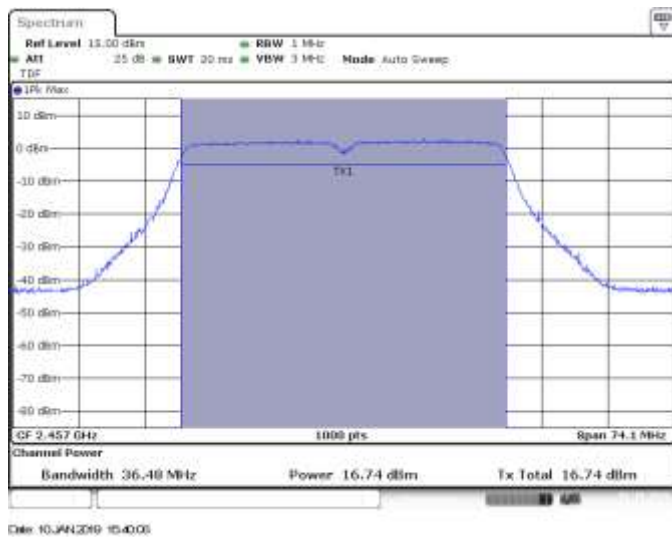
MIMO A, CH10, 802.11n40, HT8
