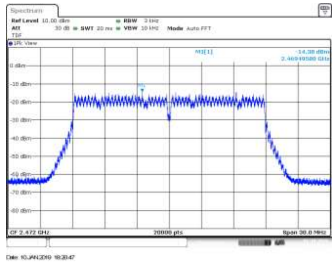
MIMO A, CH13, 802.11n20, HT8
