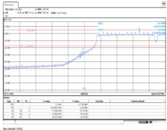
SISO A, CH3, 802.11n40, HT0, BE Low (Non Restricted)
