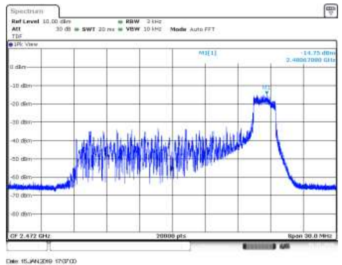
MIMO A, CH13, 802.11he20, RU26_8, HE0
