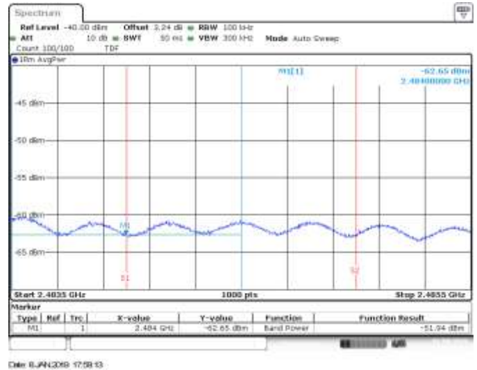
MIMO B, CH13, 802.11n20, HT8, BE High RMS within 2MHz (Restricted)
