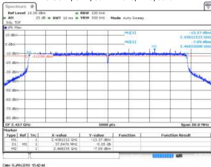
MIMO B, CH10, 802.11he40, HE0, 6dB
