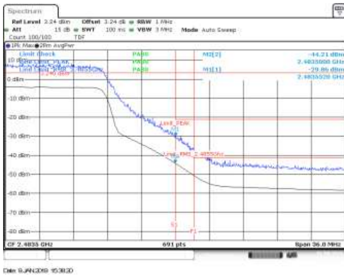
MIMO B, CH10, 802.11he40, HE0, BE High (Restricted)
