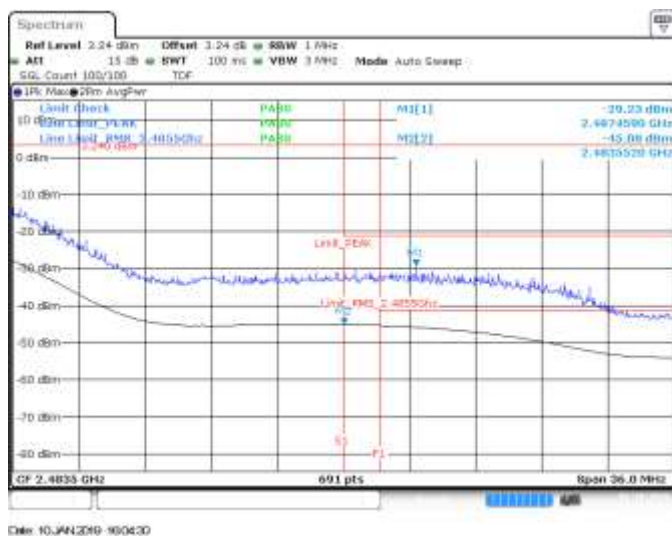
MIMO A, CH9, 802.11he40, HE0, BE High (Restricted)
