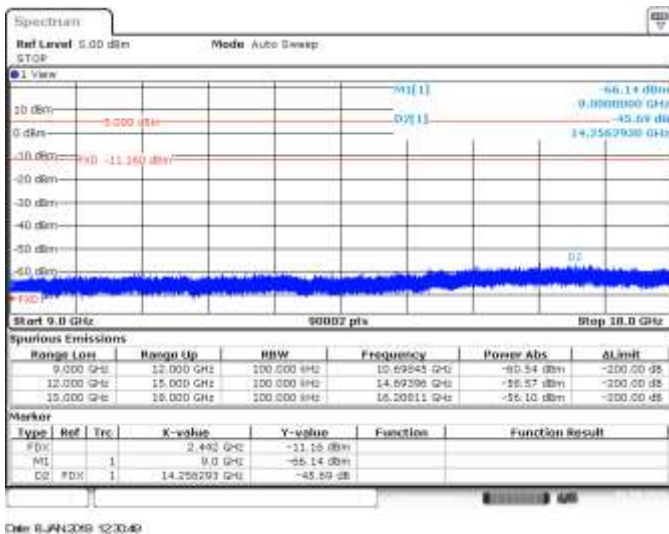
CH7, 802.11he20, HE0, SISO B, Range 9GHz to 18GHz - Delta Marker Measurement
