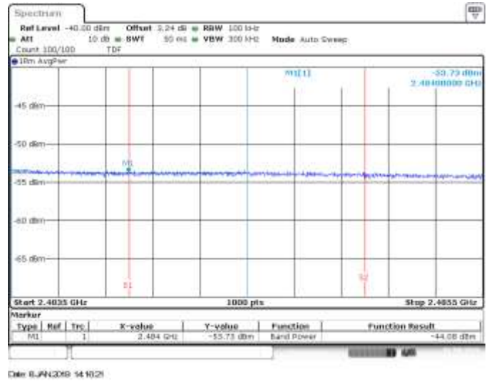
SISO B, CH13, 802.11he20, HE0, BE High RMS within 2MHz (Restricted)
