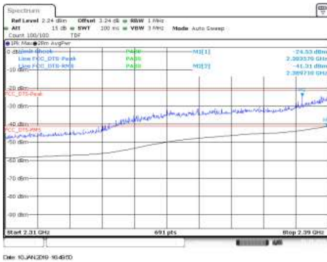
SISO A, CH3, 802.11he40, HE0, BE Low
