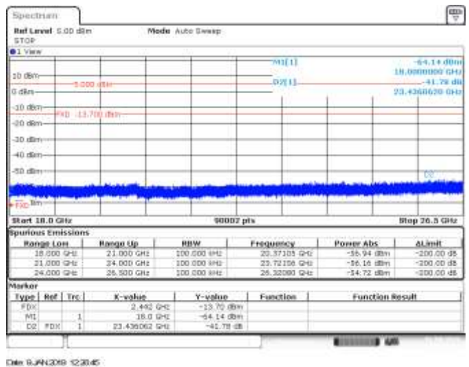
CH7, 802.11he20, HE0, MIMO B, Range 18GHz to 26.5GHz - Delta Marker Measurement
