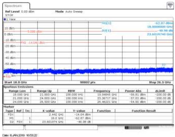
CH7, 802.11n20, HT8, MIMO B, Range 18GHz to 26.5GHz - Delta Marker Measurement
