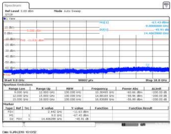
CH7, 802.11n20, HT8, MIMO A, Range 9GHz to 18GHz - Delta Marker Measurement
