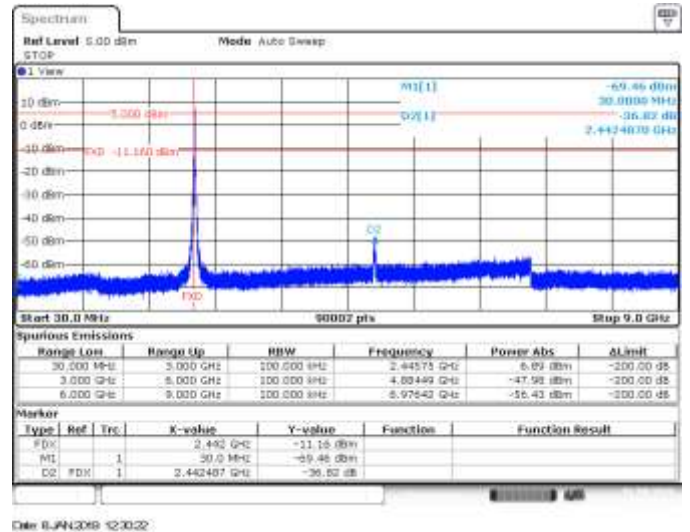
CH7, 802.11he20, HE0, SISO B, Range 30MHz to 9GHz - Delta Marker Measurement
