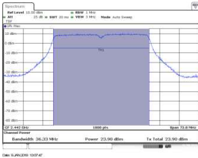
MIMO B, CH7, 802.11n40, HT8
