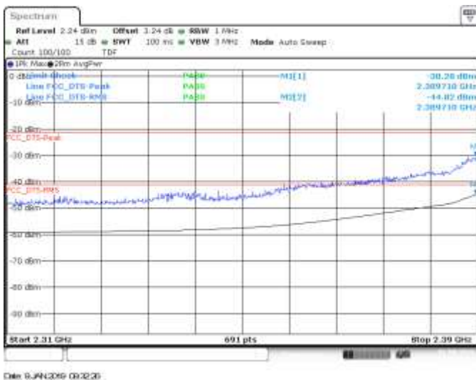
MIMO A, CH1, 802.11n20, HT8, BE Low
