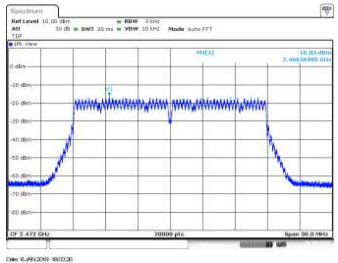
MIMO B, CH13, 802.11n20, HT8
