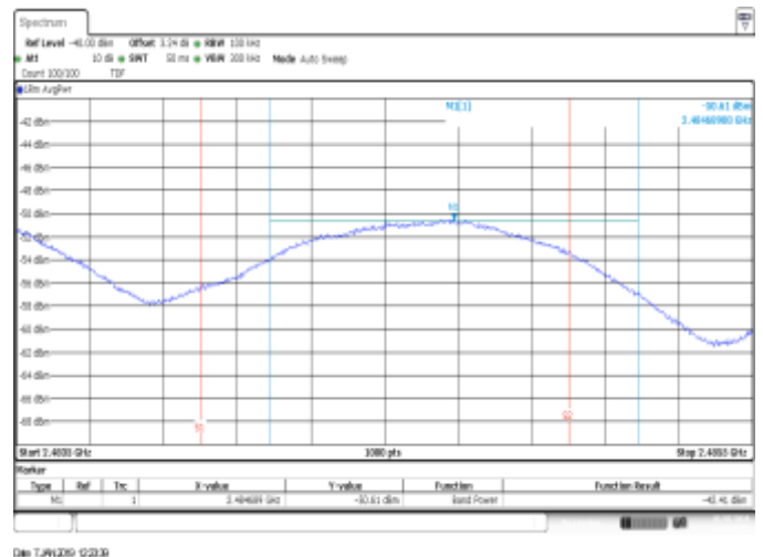
SISO B, CH11, 802.11b, 1Mbps, BE High RMS within 2MHz (Restricted)
