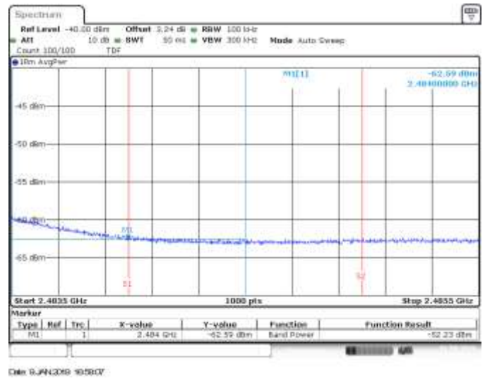
MIMO A, CH11, 802.11he40, HE0, BE High RMS within 2MHz (Restricted)
