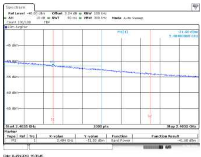
SISO B, CH10, 802.11he40, HE0, BE High RMS within 2MHz (Restricted)
