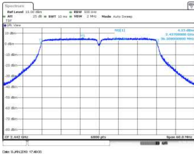
MIMO A, CH7, 802.11n40, HT8, 99%
