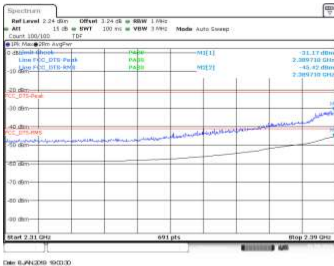
MIMO B, CH1, 802.11he20, HE0, BE Low
