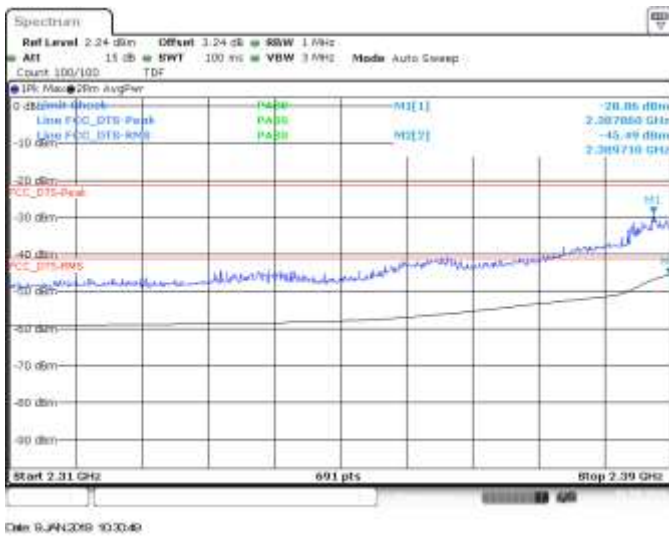
MIMO A, CH1, 802.11he20, HE0, BE Low
