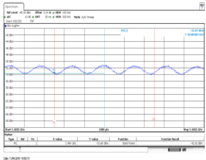
SISO A, CH9, 802.11n40, HT0, BE High RMS within 2MHz (Restricted)
