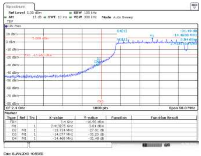
SISO B, CH3, 802.11n40, HT0, BE Low (Non Restricted)
