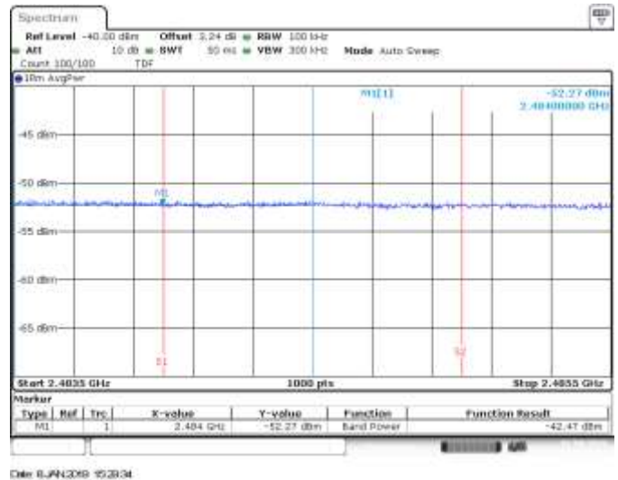
SISO B, CH9, 802.11he40, HE0, BE High RMS within 2MHz (Restricted)
