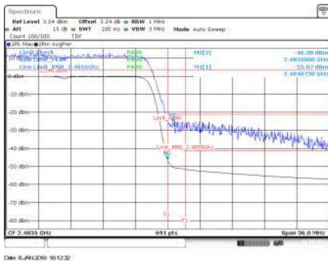
MIMO B, CH13, 802.11he20, HE0, BE High (Restricted)
