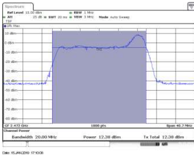
MIMO A, CH13, 802.11he20, RU26_8, HE0
