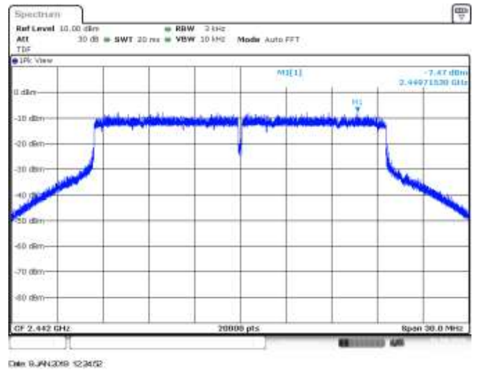
MIMO B, CH7, 802.11he20, HE0
