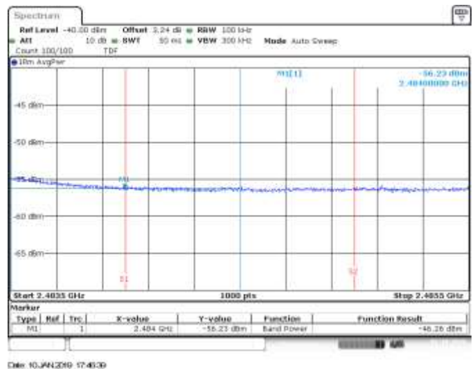
SISO A, CH11, 802.11he40, HE0, BE High RMS within 2MHz (Restricted)
