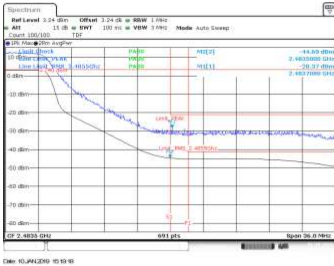
MIMO A, CH9, 802.11n40, HT8, BE High (Restricted)
