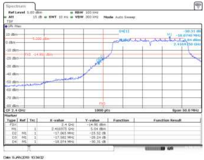
MIMO A, CH1, 802.11he20, HE0, BE Low (Non Restricted)
