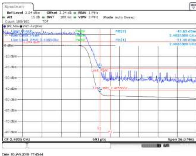
SISO A, CH11, 802.11he40, HE0, BE High (Restricted)
