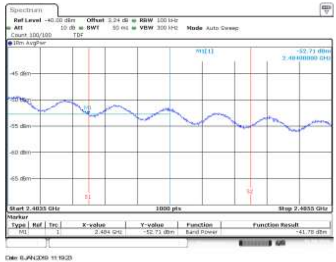
SISO B, CH10, 802.11n40, HT0, BE High RMS within 2MHz (Restricted)
