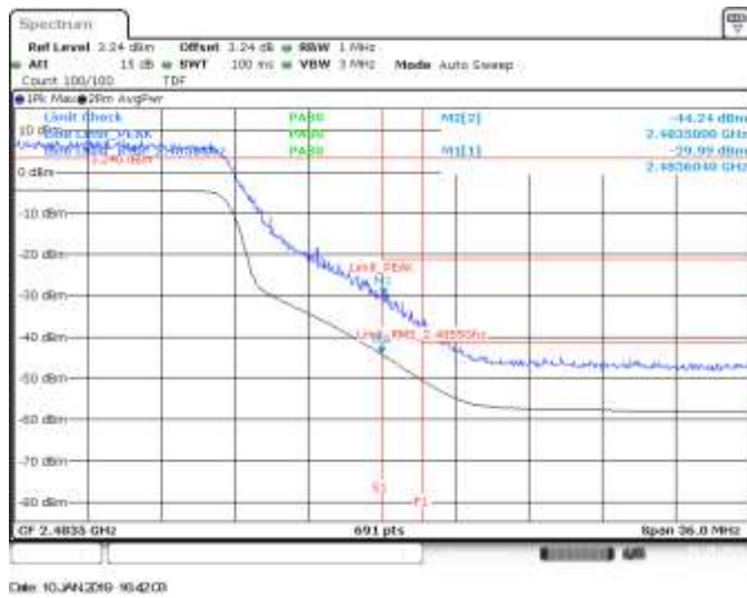
MIMO A, CH10, 802.11he40, HE0, BE High (Restricted)
