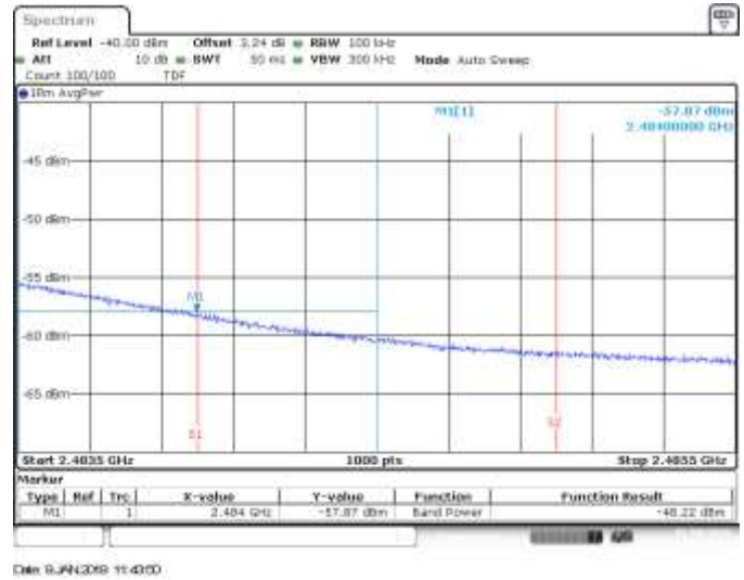
MIMO A, CH12, 802.11he20, HE0, BE High RMS within 2MHz (Restricted)
