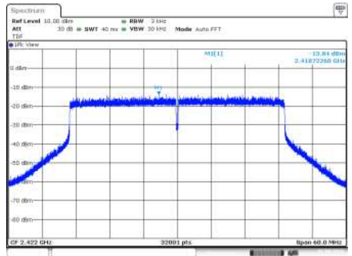
MIMO A, CH3, 802.11he40, RU242_61, HE0
