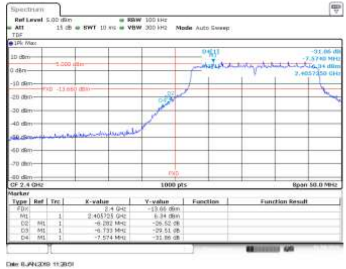
SISO B, CH1, 802.11he20, HE0, BE Low (Non Restricted)
