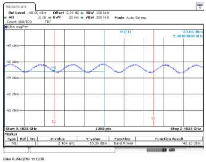
SISO B, CH9, 802.11n40, HT0, BE High RMS within 2MHz (Restricted)
