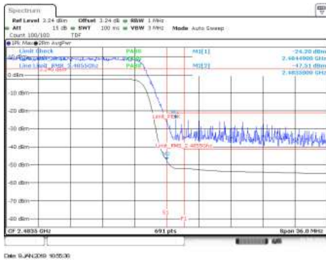
MIMO A, CH11, 802.11he40, HE0, BE High (Restricted)
