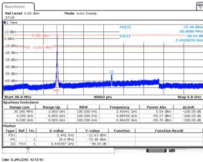
CH7, 802.11n20, HT8, MIMO A, Range 30MHz to 9GHz - Delta Marker Measurement
