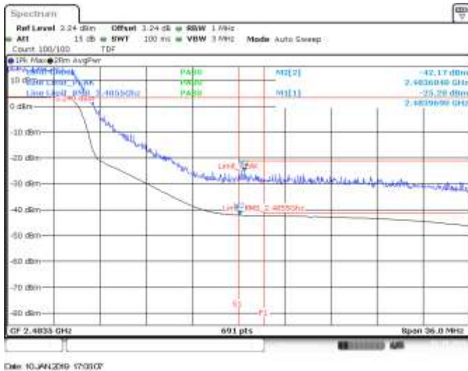
SISO A, CH9, 802.11he40, HE0, BE High (Restricted)
