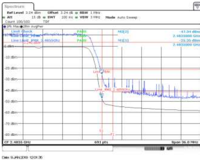
MIMO A, CH13, 802.11he20, HE0, BE High (Restricted)
