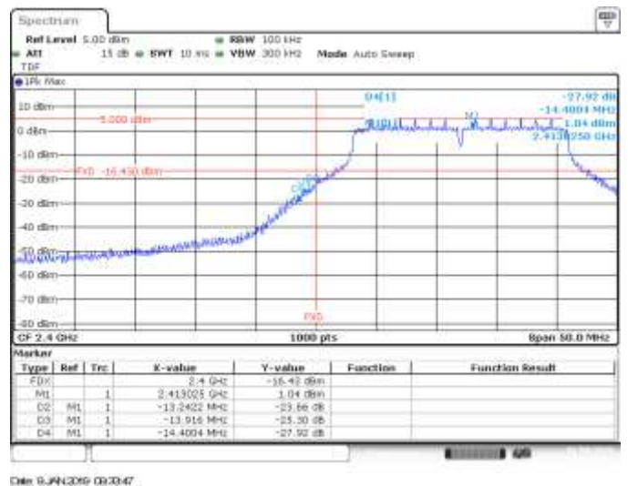
MIMO A, CH1, 802.11n20, HT8, BE Low (Non Restricted)
