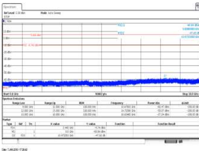
CH7, 802.11g, 6Mbps, SISO B, Range 9GHz to 18GHz - Delta Marker Measurement
