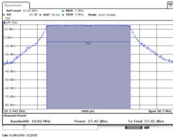
MIMO B, CH7, 802.11he20, HE0
