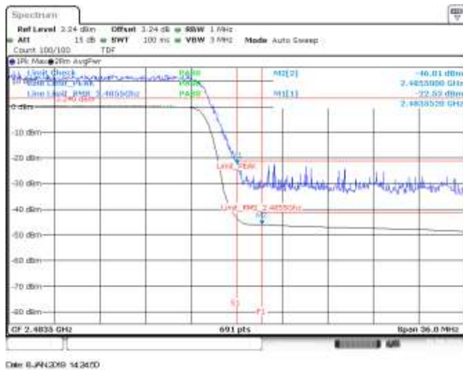
SISO B, CH11, 802.11he40, HE0, BE High (Restricted)
