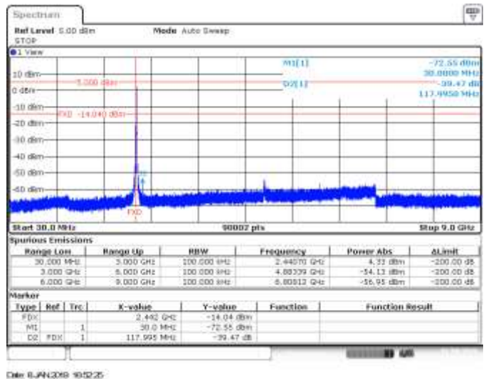
CH7, 802.11n20, HT8, MIMO B, Range 30MHz to 9GHz - Delta Marker Measurement
