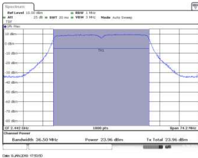
MIMO A, CH7, 802.11n40, HT8
