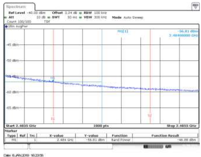
MIMO B, CH12, 802.11he20, HE0, BE High RMS within 2MHz (Restricted)
