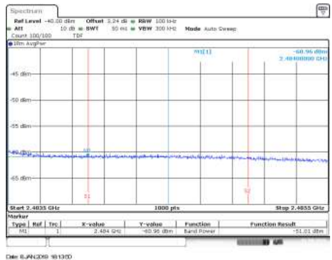
MIMO B, CH13, 802.11he20, HE0, BE High RMS within 2MHz (Restricted)
