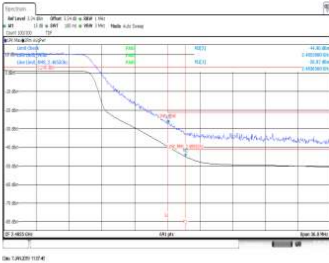
SISO A, CH10, 802.11n40, HT0, BE High (Restricted)
