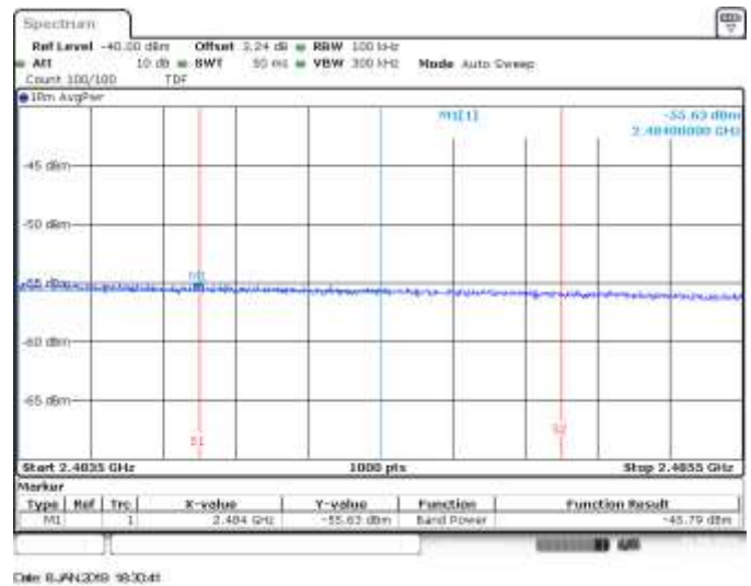
MIMO B, CH11, 802.11he20, HE0, BE High RMS within 2MHz (Restricted)
