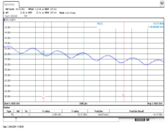
SISO A, CH10, 802.11n40, HT0, BE High RMS within 2MHz (Restricted)
