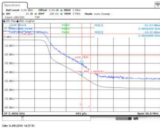
MIMO B, CH10, 802.11n40, HT8, BE High (Restricted)
