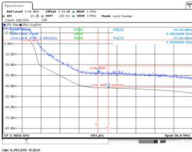
SISO B, CH9, 802.11he40, HE0, BE High (Restricted)
