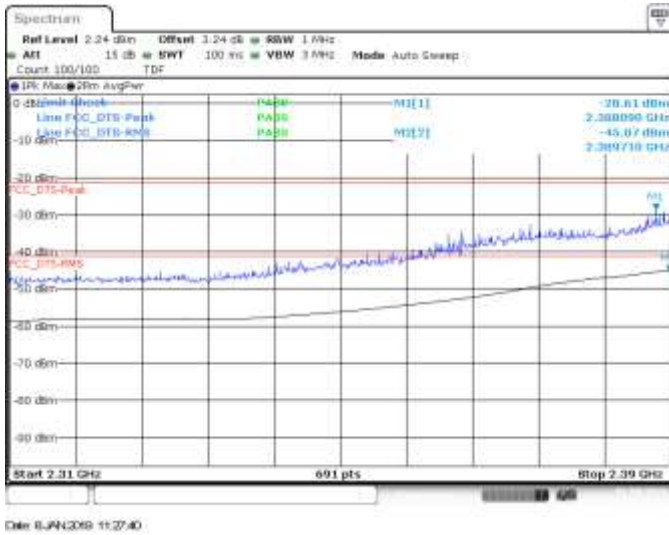
SISO B, CH1, 802.11he20, HE0, BE Low
