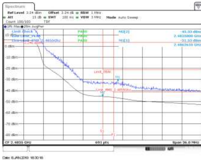
MIMO B, CH11, 802.11he20, HE0, BE High (Restricted)
