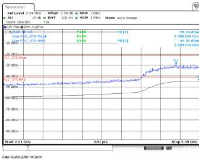
MIMO B, CH3, 802.11he40, HE0, BE Low
