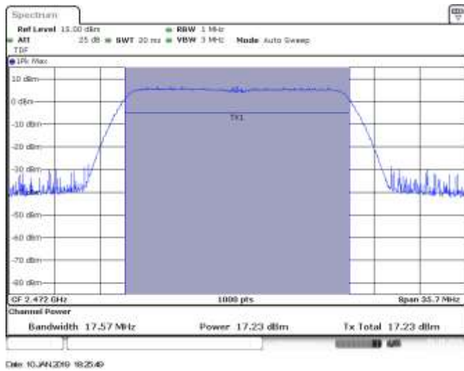
MIMO A, CH13, 802.11n20, HT8
