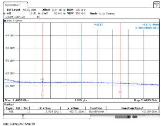
MIMO A, CH13, 802.11he20, HE0, BE High RMS within 2MHz (Restricted)
