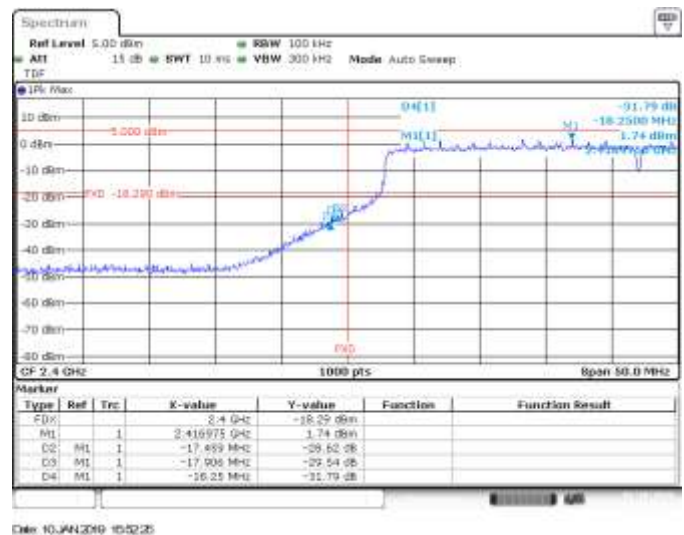
MIMO A, CH3, 802.11he40, HE0, BE Low (Non Restricted)
