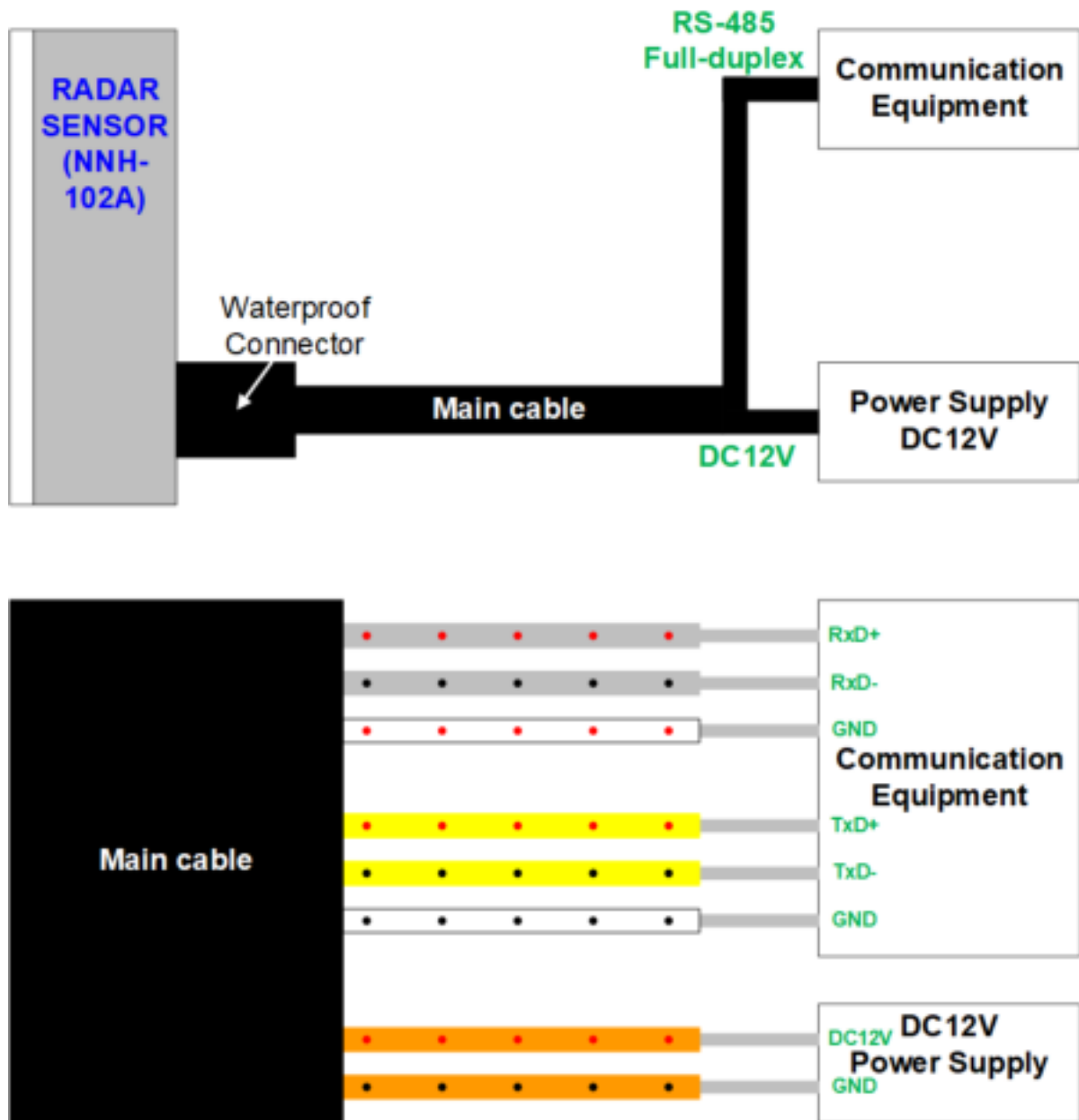
Figure 3: Connection from the JRC-M's RADAR SENSOR to power supply and communication equipment.
