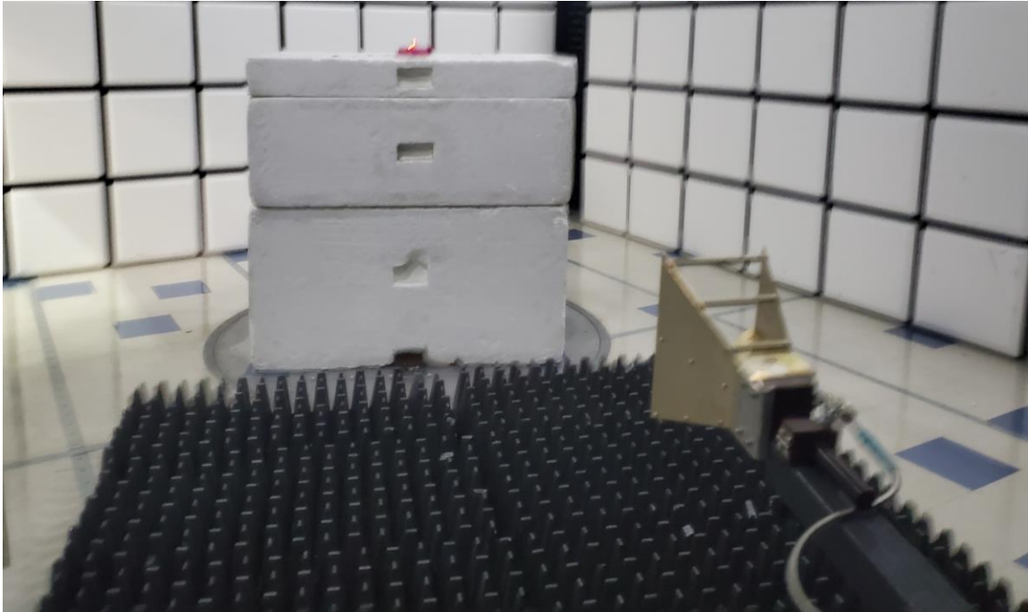
Above 1 GHz
