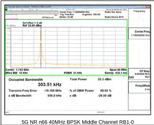
5G NR n66 40MHz BPSK Middle Channel RB1-0
