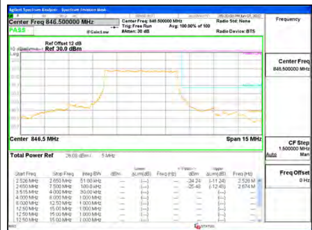
5G NR n5 5MHz BPSK High Channel RB25-0-ID-12482
