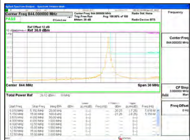
5G NR n5 10MHz BPSK High Channel RB1-51-ID-12482
