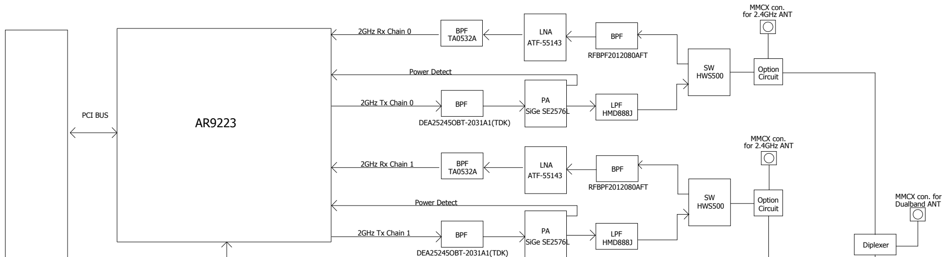
2.4GHz Radio Block Diagram
