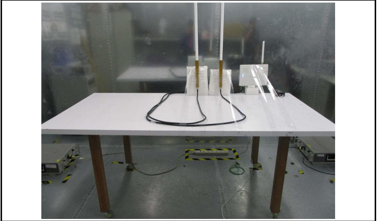
Conducted Emission Test (POE: POE29U-1AT)
