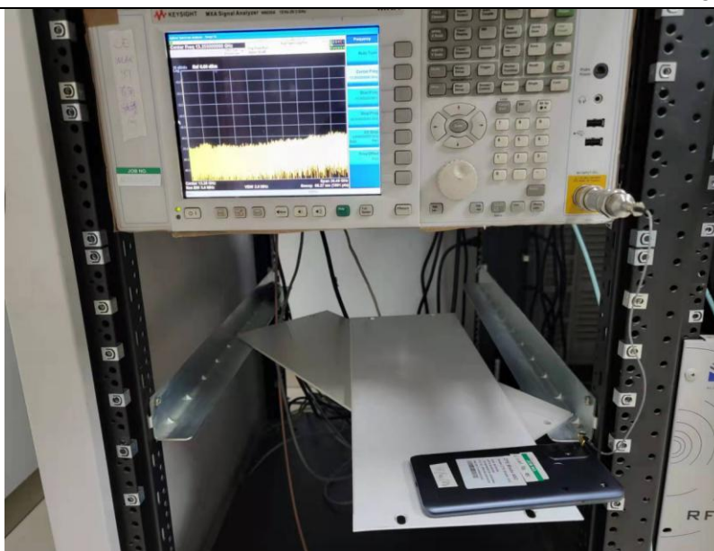
RF Conducted Test setup (BT/WIFI)
