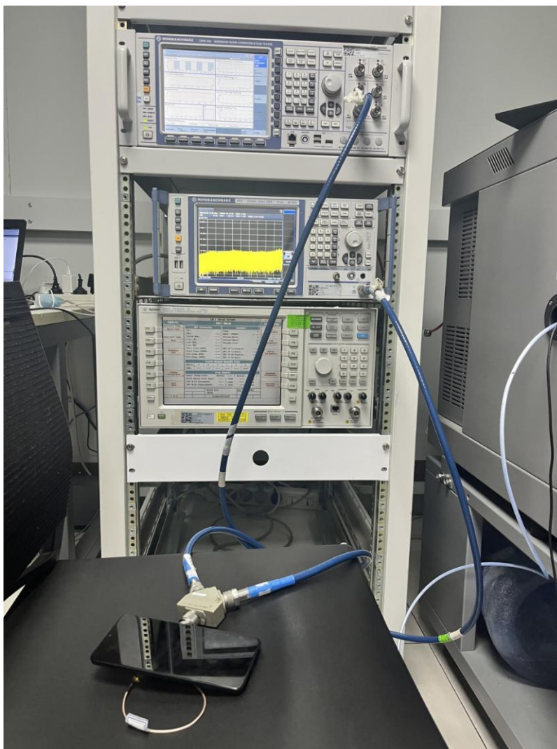
'RF Conducted Test setup (GSM/WCDMA/LTE)
