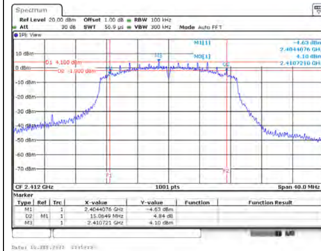
802.11n (20 MHz) / Ant. 1 / 2412 MHz
