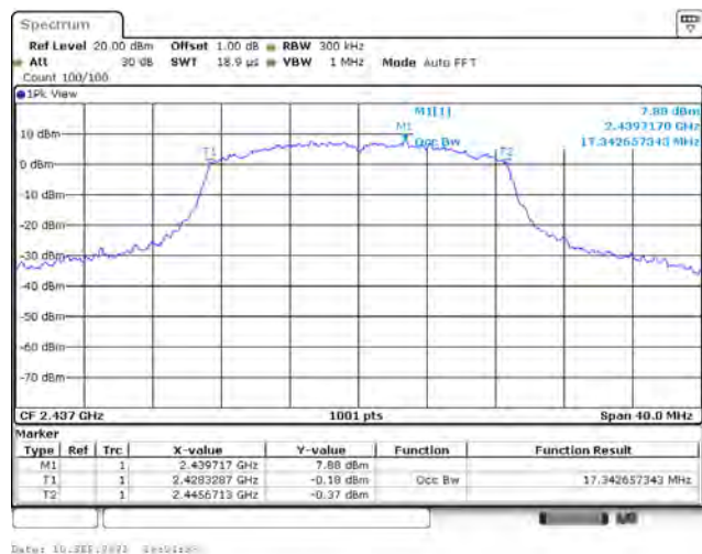
802.11n (20 MHz) / Ant. 0 / 2437 MHz
