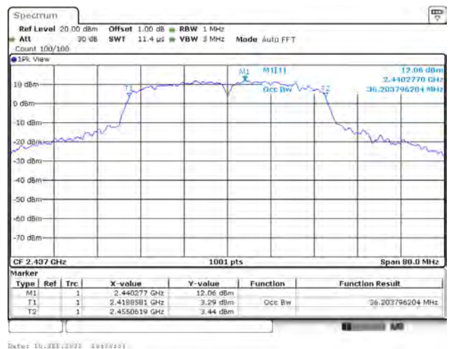
802.11n (40 MHz) / Ant. 0 / 2437 MHz
