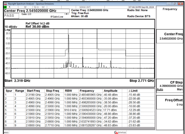
Band41_90MHz_CP_OFDM_SCS30kHz_QPSK_RB1_0_CH509004
