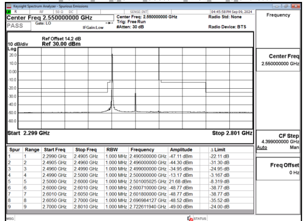
Band41_100MHz_DFT_s_OFDM_SCS30kHz_BPSK_RB1_0_CH510000
