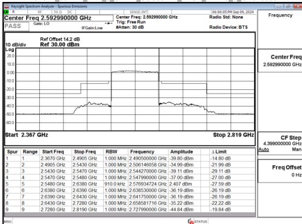
Band41_90MHz_DFT_s_OFDM_SCS30kHz_BPSK_RB243_0_CH518598
