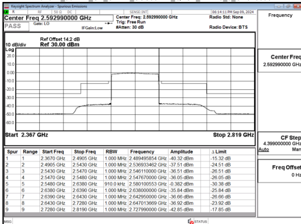
Band41_90MHz_CP_OFDM_SCS30kHz_QPSK_RB245_0_CH518598
