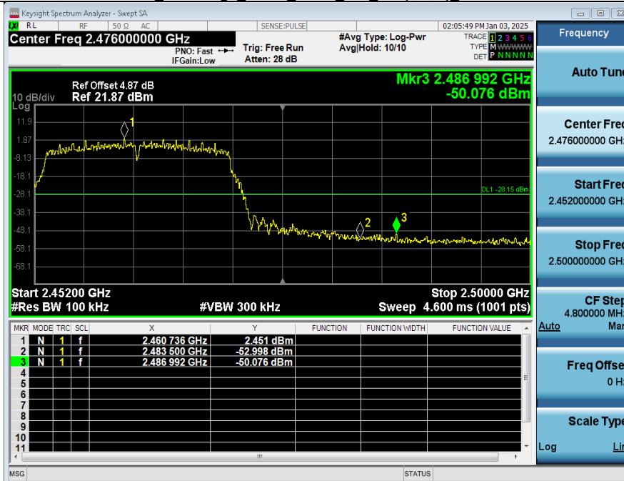
2_Bandedge_NVNT_ANT2_802_11n(HT20)_2462
