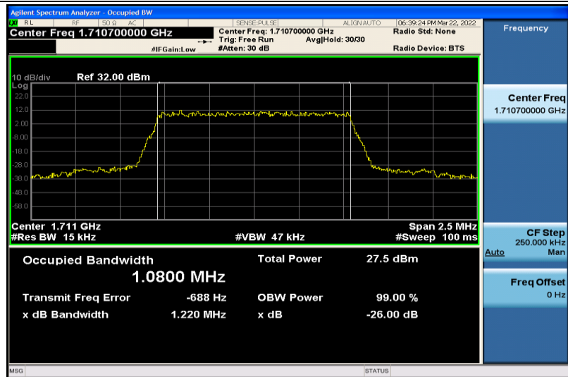
Band4-1.4MHz-QPSK-19957-6RB#0-1.0800
