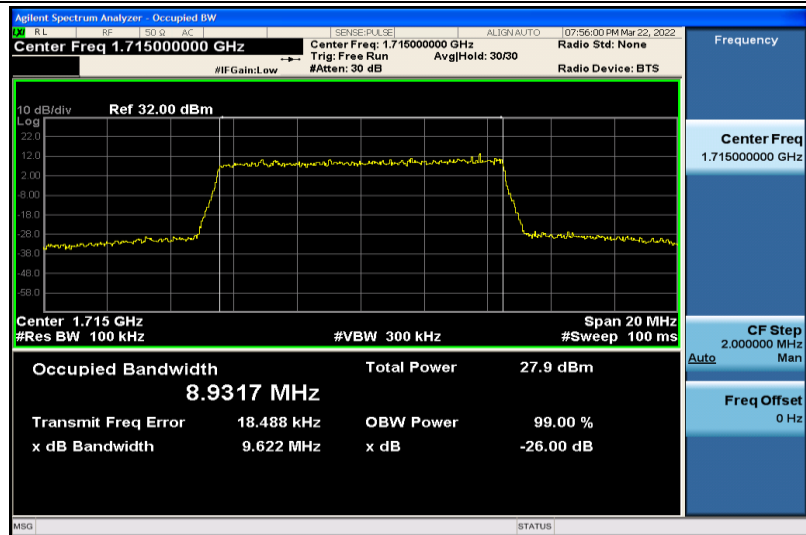
Band4-10MHz-16QAM-20000-50RB#0-8.9317
