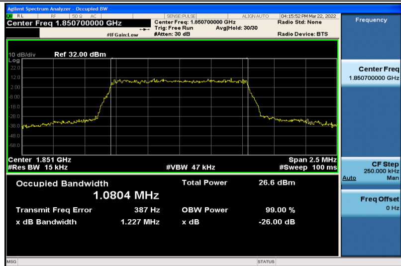
Band2-1.4MHz-16QAM-18607-6RB#0-1.0804
