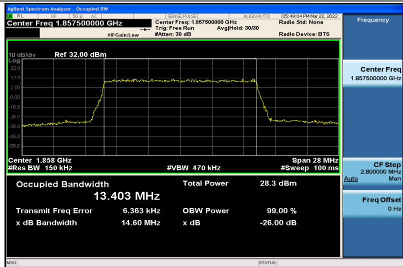
Band2-15MHz-16QAM-18675-75RB#0-13.403
