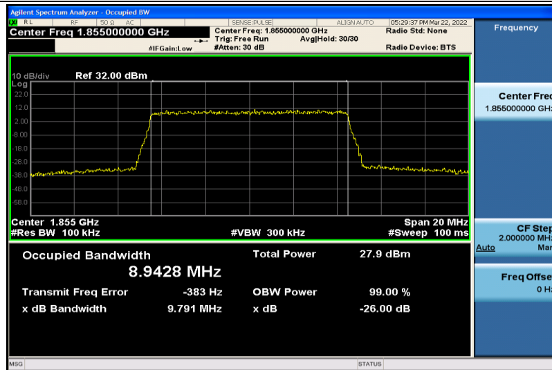
Band2-10MHz-16QAM-18650-50RB#0-8.9428
