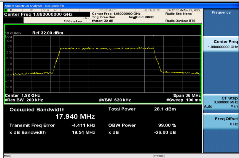
Band2-20MHz-16QAM-18900-100RB#0-17.940
