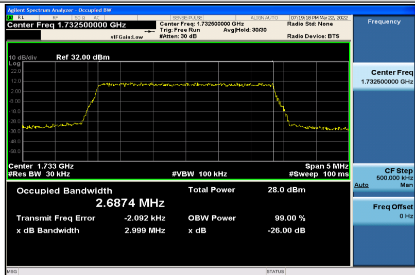
Band4-3MHz-QPSK-20175-15RB#0-2.6874
