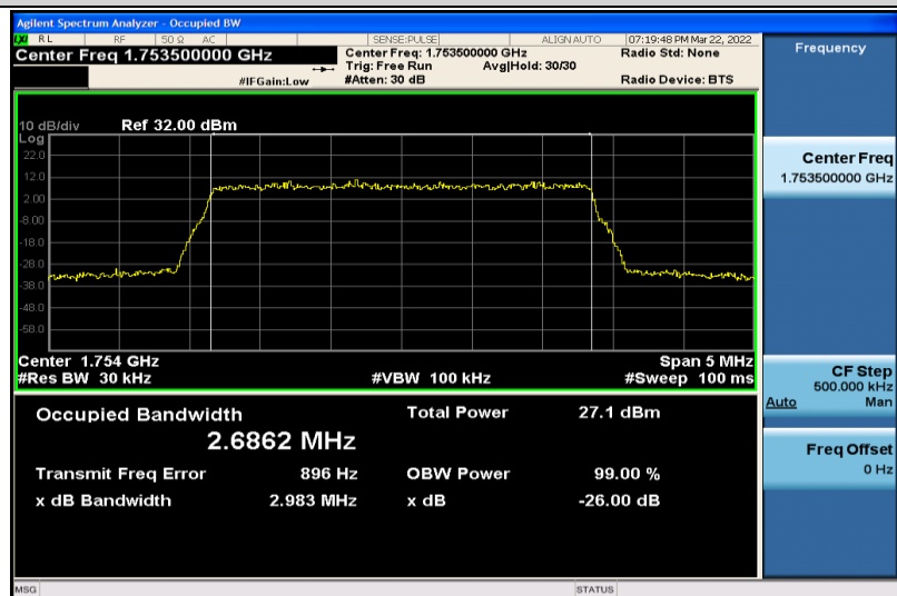
Band4-3MHz-16QAM-20385-15RB#0-2.6862
