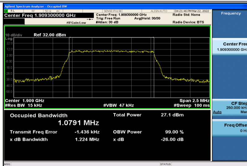
Band2-1.4MHz-QPSK-19193-6RB#0-1.0791
