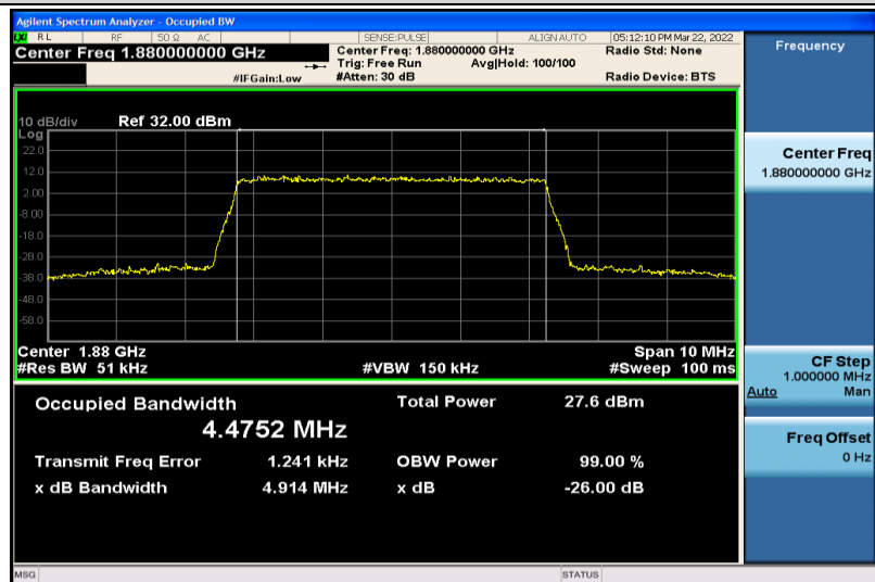
Band2-5MHz-16QAM-18900-25RB#0-4.4752
