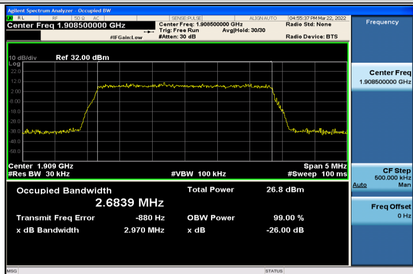
Band2-3MHz-16QAM-19185-15RB#0-2.6839
