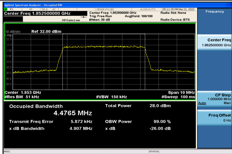
Band2-5MHz-16QAM-18625-25RB#0-4.4765
