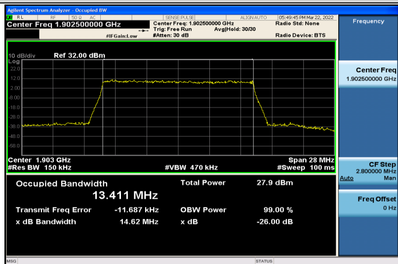
Band2-15MHz-16QAM-19125-75RB#0-13.411
