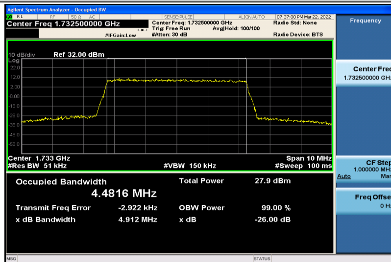
Band4-5MHz-16QAM-20175-25RB#0-4.4816
