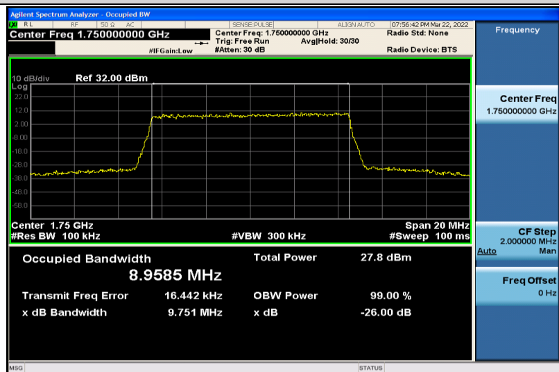
Band4-10MHz-16QAM-20350-50RB#0-8.9585
