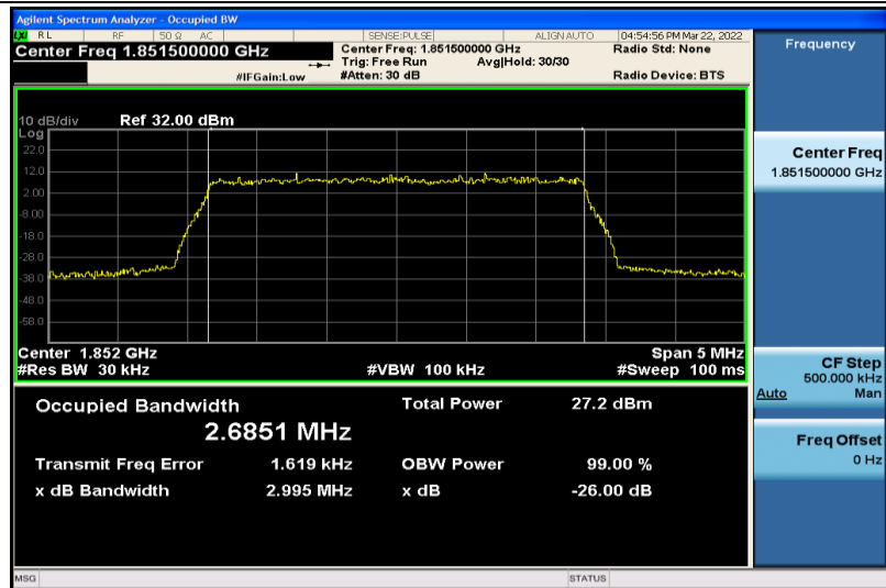
Band2-3MHz-16QAM-18615-15RB#0-2.6851
