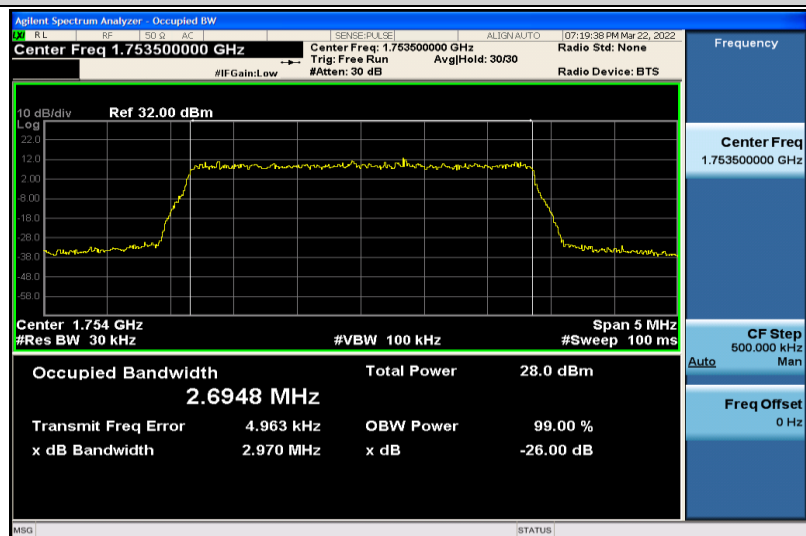
Band4-3MHz-QPSK-20385-15RB#0-2.6948
