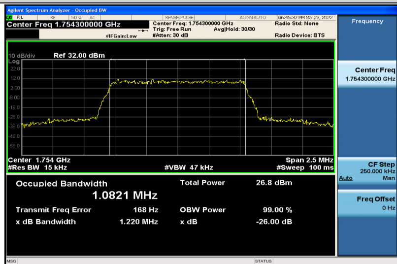
Band4-1.4MHz-16QAM-20393-6RB#0-1.0821
