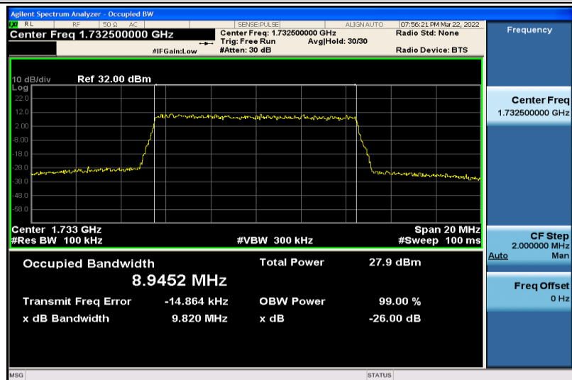
Band4-10MHz-16QAM-20175-50RB#0-8.9452
