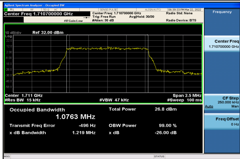
Band4-1.4MHz-16QAM-19957-6RB#0-1.0763
