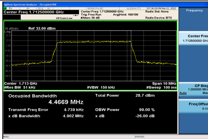
Band4-5MHz-QPSK-19975-25RB#0-4.4669
