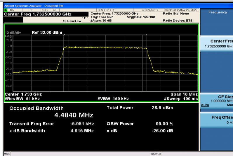
Band4-5MHz-QPSK-20175-25RB#0-4.4840
