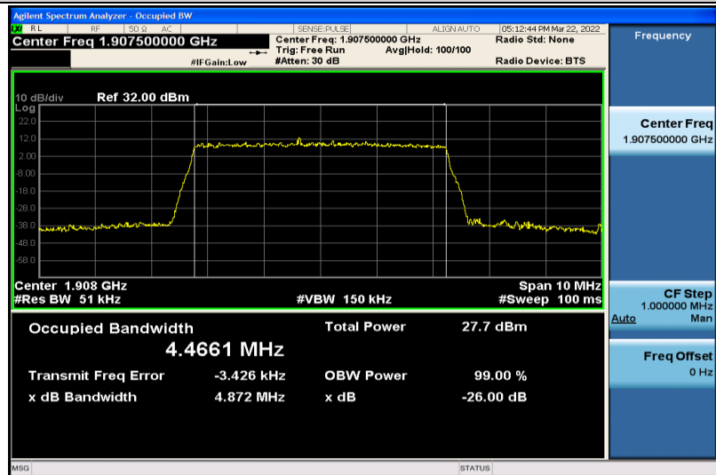
Band2-5MHz-16QAM-19175-25RB#0-4.4661
