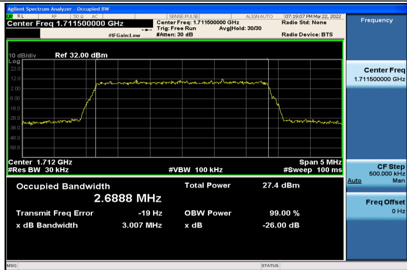
Band4-3MHz-16QAM-19965-15RB#0-2.6888
