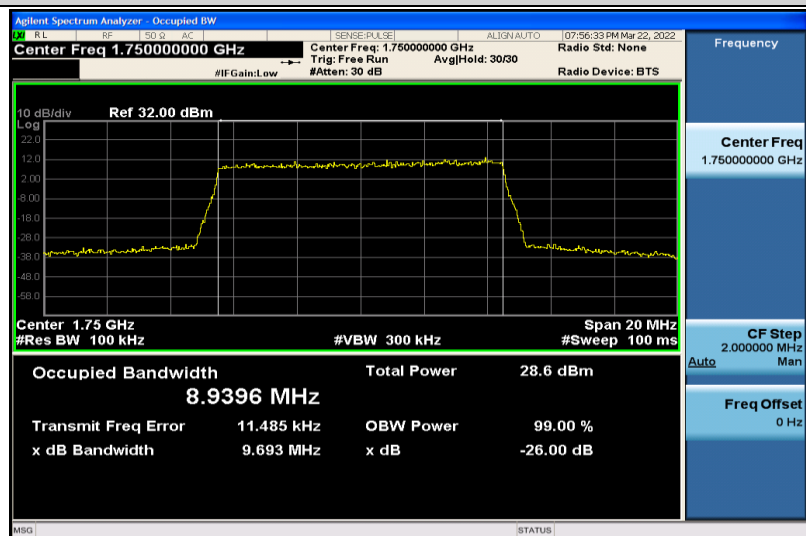
Band4-10MHz-QPSK-20350-50RB#0-8.9396
