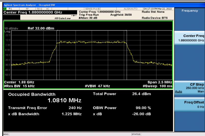
Band2-1.4MHz-16QAM-18900-6RB#0-1.0810
