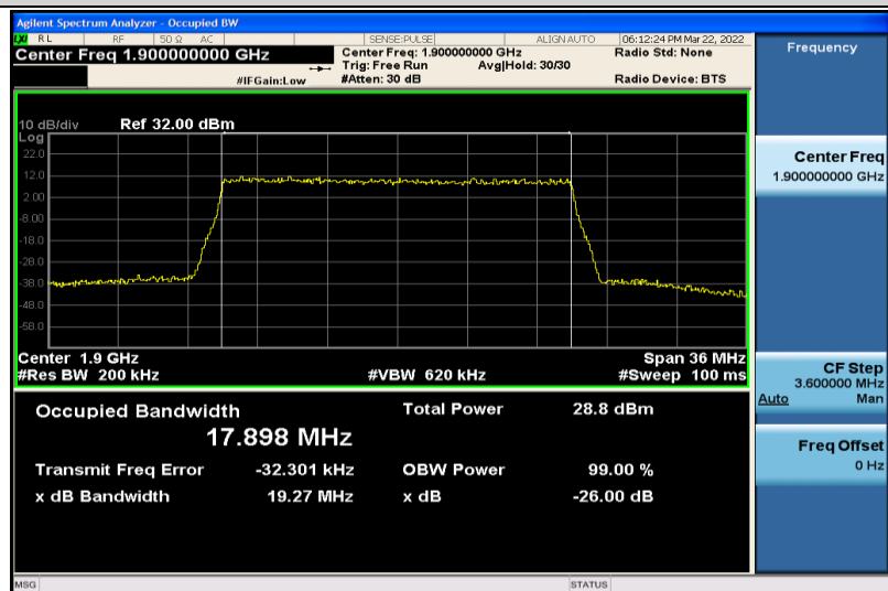
Band2-20MHz-QPSK-19100-100RB#0-17.898
