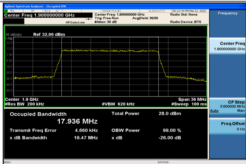
Band2-20MHz-16QAM-19100-100RB#0-17.936
