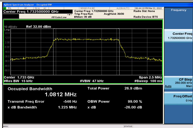
Band4-1.4MHz-16QAM-20175-6RB#0-1.0812
