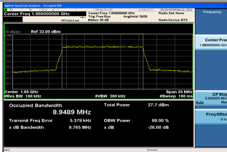
Band2-10MHz-16QAM-18900-50RB#0-8.9489
