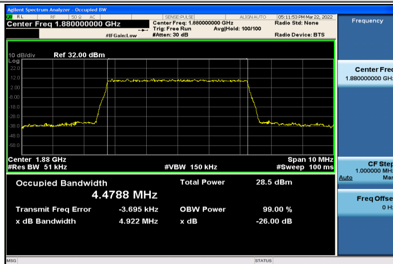
Band2-5MHz-QPSK-18900-25RB#0-4.4788
