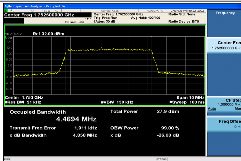
Band4-5MHz-16QAM-20375-25RB#0-4.4694
