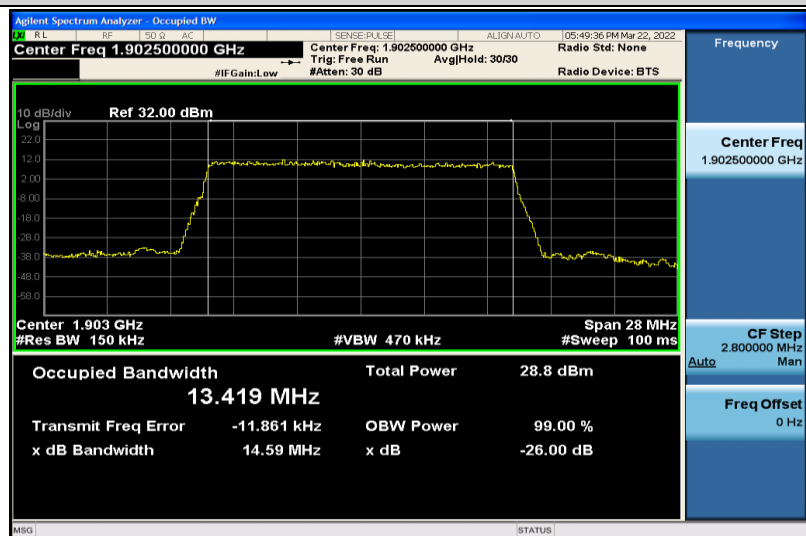
Band2-15MHz-QPSK-19125-75RB#0-13.419
