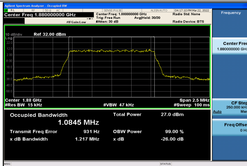
Band2-1.4MHz-QPSK-18900-6RB#0-1.0845
