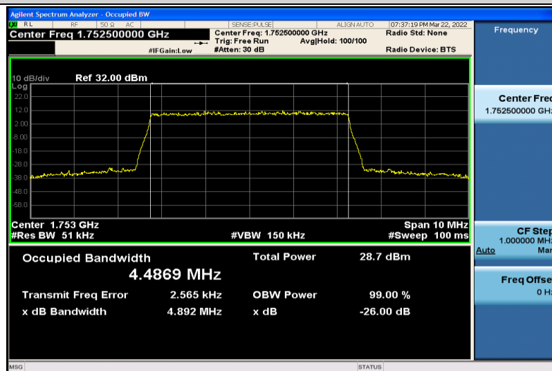
Band4-5MHz-QPSK-20375-25RB#0-4.4869
