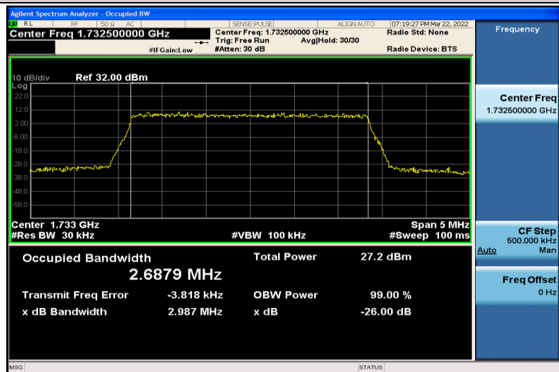
Band4-3MHz-16QAM-20175-15RB#0-2.6879
