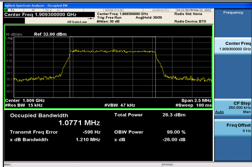
Band2-1.4MHz-16QAM-19193-6RB#0-1.0771
