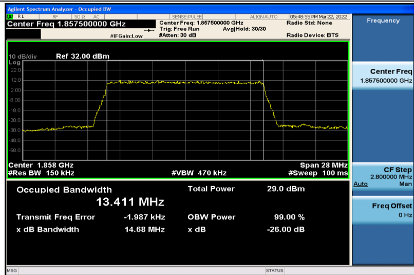
Band2-15MHz-QPSK-18675-75RB#0-13.411
