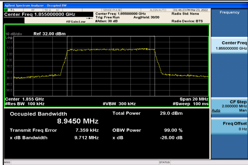
Band2-10MHz-QPSK-18650-50RB#0-8.9450
