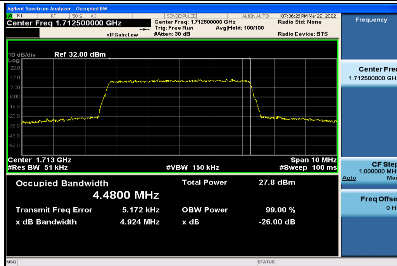
Band4-5MHz-16QAM-19975-25RB#0-4.4800
