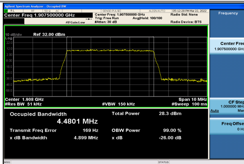
Band2-5MHz-QPSK-19175-25RB#0-4.4801
