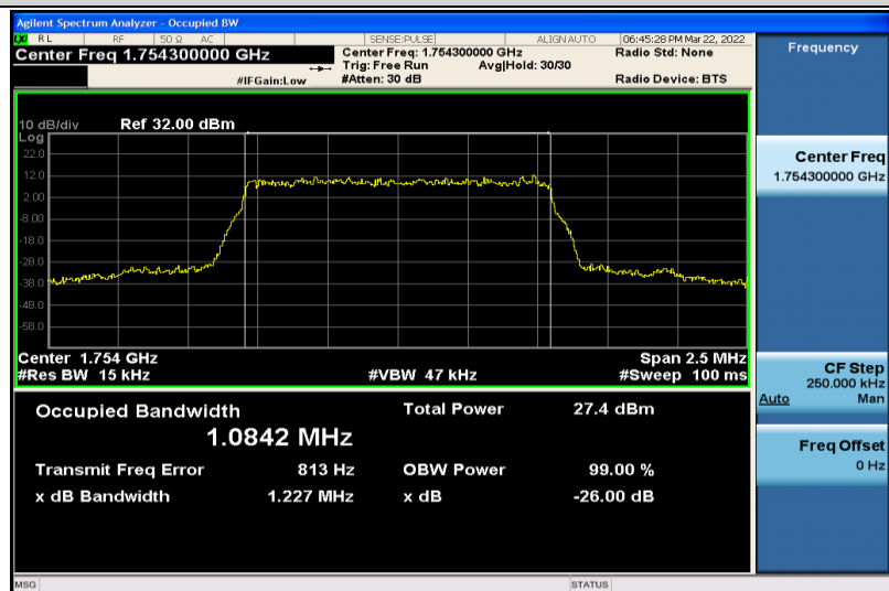
Band4-1.4MHz-QPSK-20393-6RB#0-1.0842
