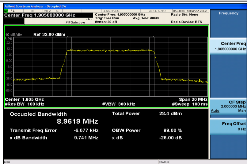
Band2-10MHz-QPSK-19150-50RB#0-8.9619
