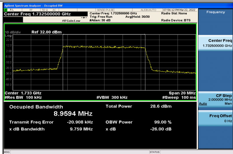
Band4-10MHz-QPSK-20175-50RB#0-8.9594
