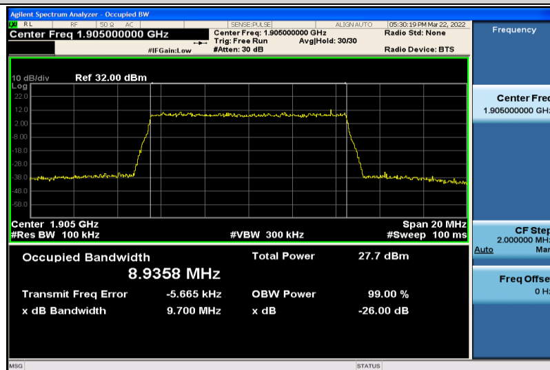
Band2-10MHz-16QAM-19150-50RB#0-8.9358
