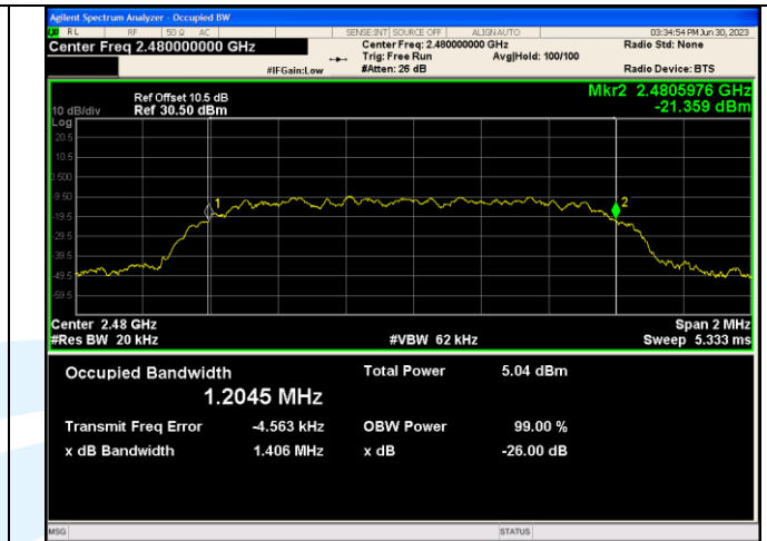
\pi/4 DQPSK_2-DH5_Channel 78
