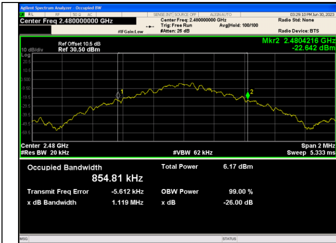
GFSK_DH5_Channel 78
