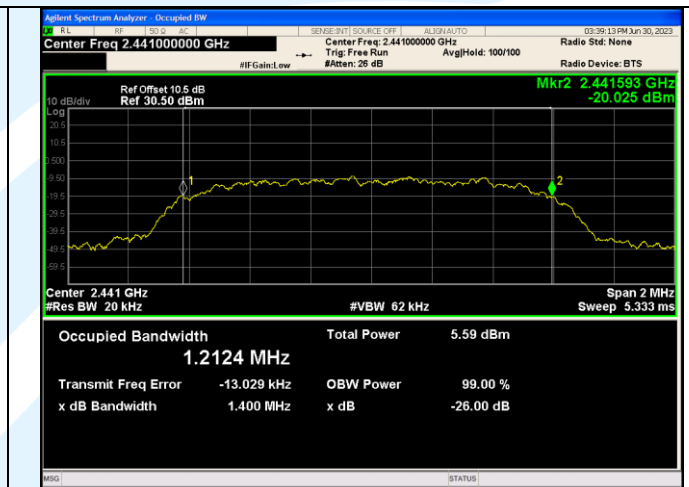
8DPSK_3-DH5_Channel 39
