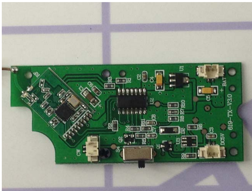
PCB side1
