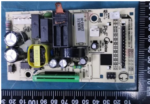
1.The Original Mother board-top view
