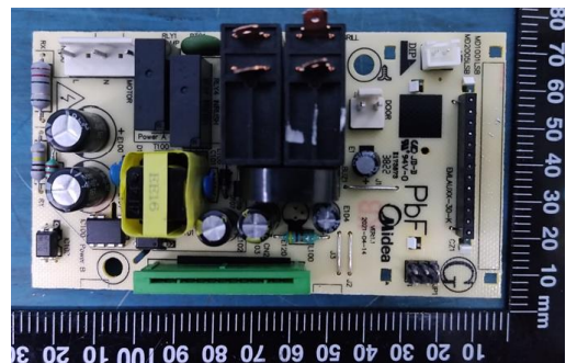
The New Mother board -top view
