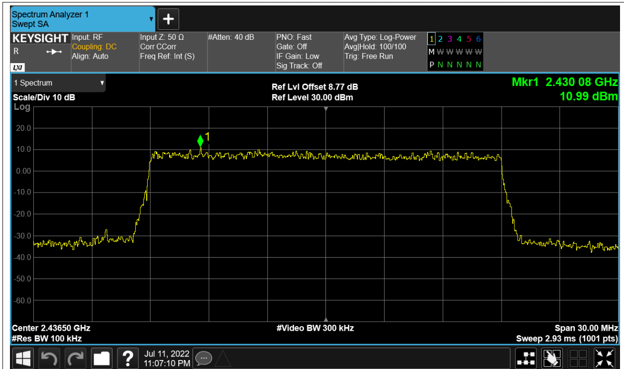
Tx. Spurious NVNT 2.4G-20M-QPSK 2436.5MHz Ant1 Emission
