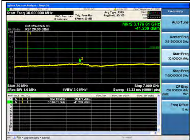
Band71 / 15MHz / High CH / 64QAM
