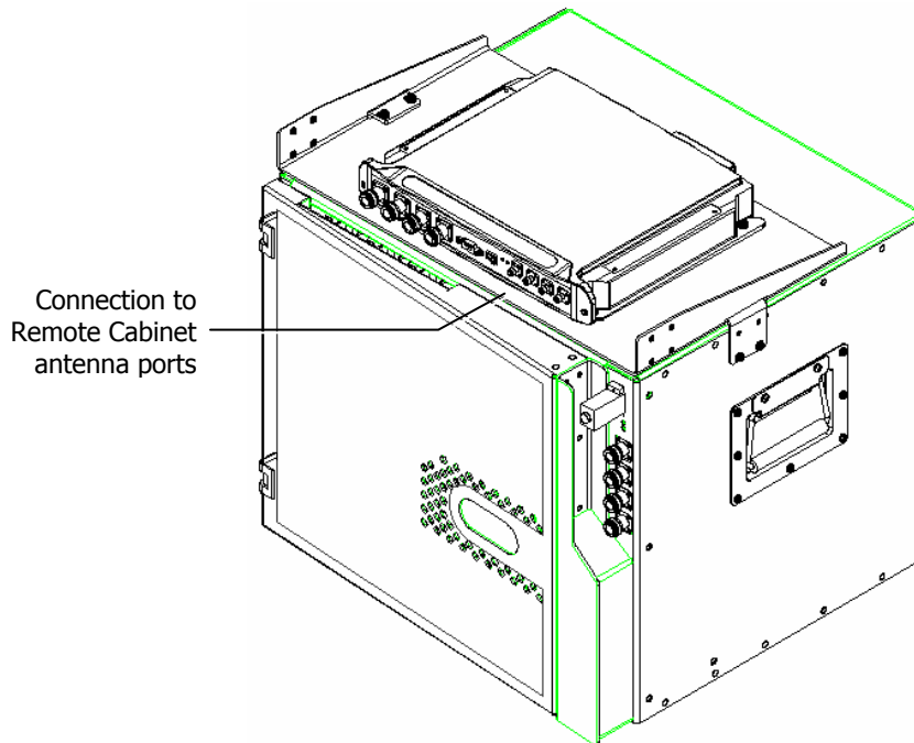
Figure 3-6. Illustration of MA 850A1 Mounted on MA 2000 RC
