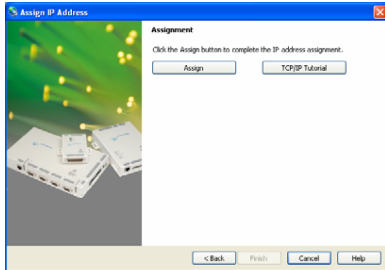
Figure 4-9. Assignment Window
