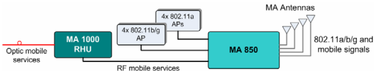
Figure 1-4 MA 850A1 as Add-On to MA 1000 System
