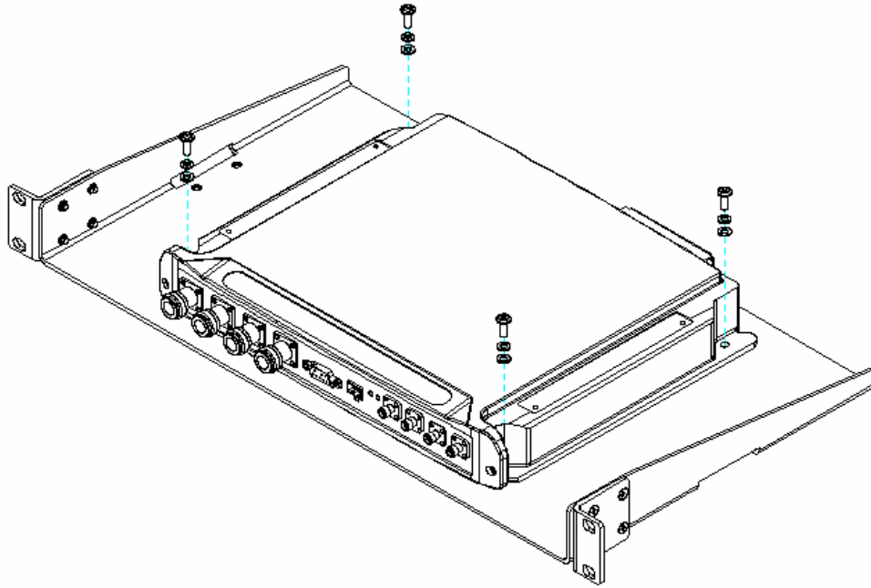
Figure 3-8. MA 850A1 to Bracket Installation
