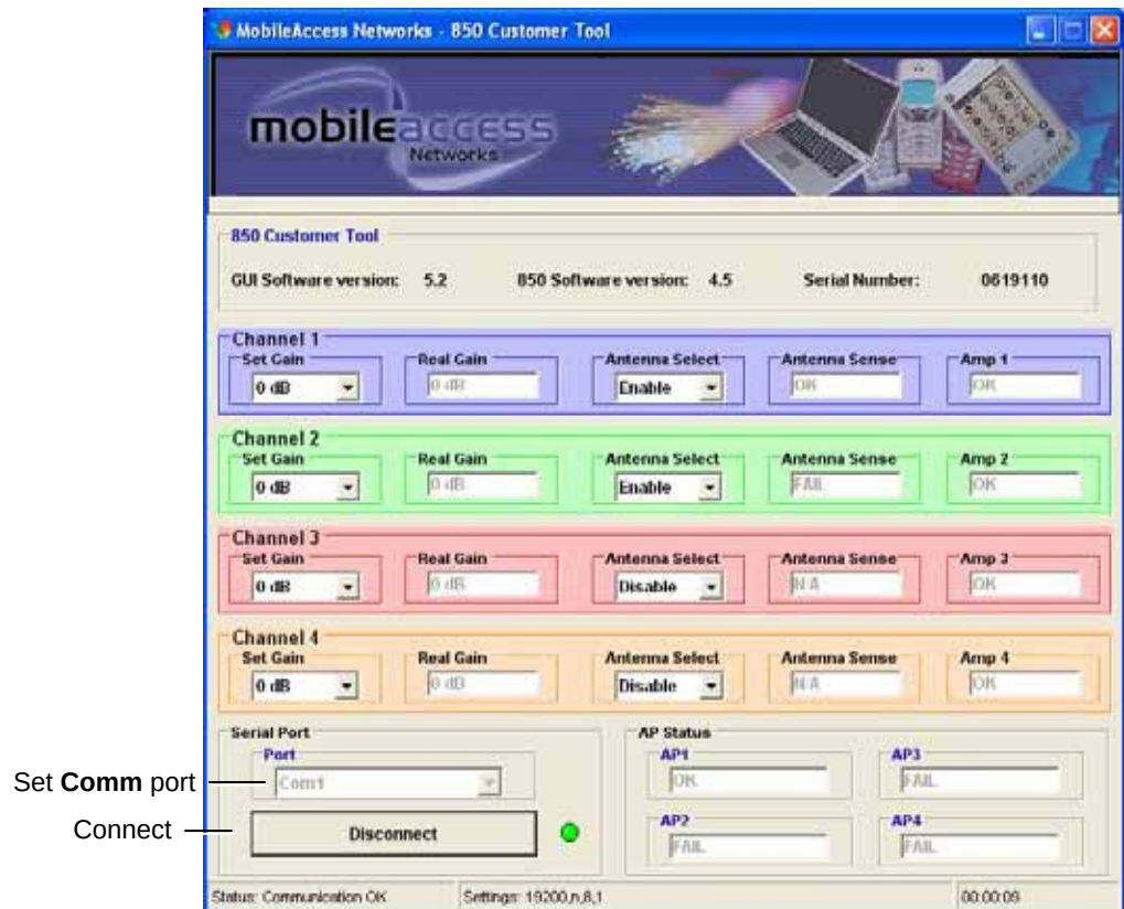
Figure 4-1. Connecting to the MA 850A1
