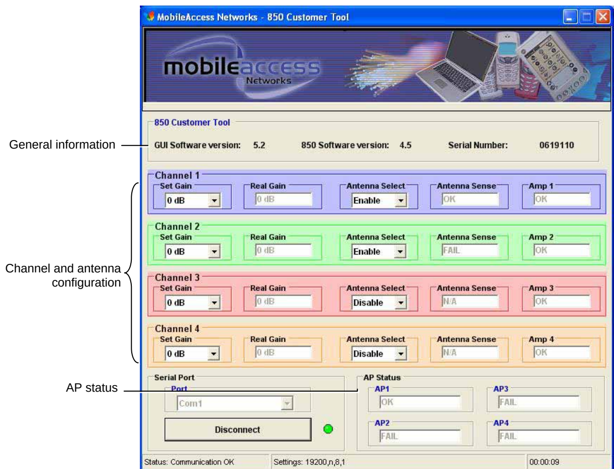
Figure 4-2. MA 850A1 Customer Tool Dialog
