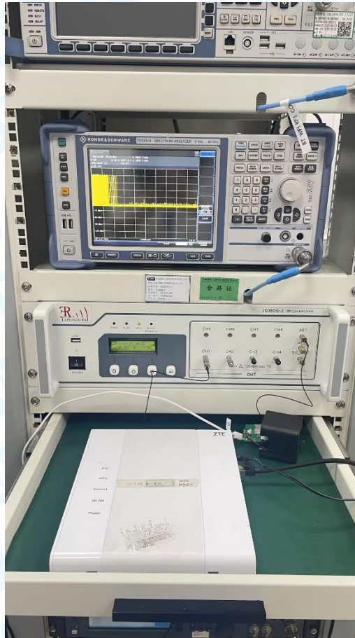
Photo of Setup for DFS Test
