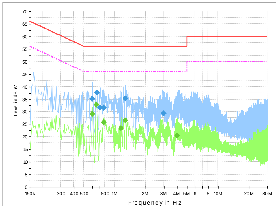
Fig.B.11.2 AC Powerline Conducted Emission-Idle
