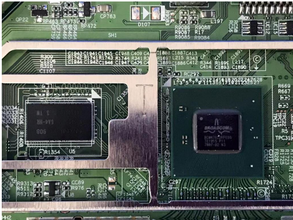
(13) EUT Photo(AP305CX)
