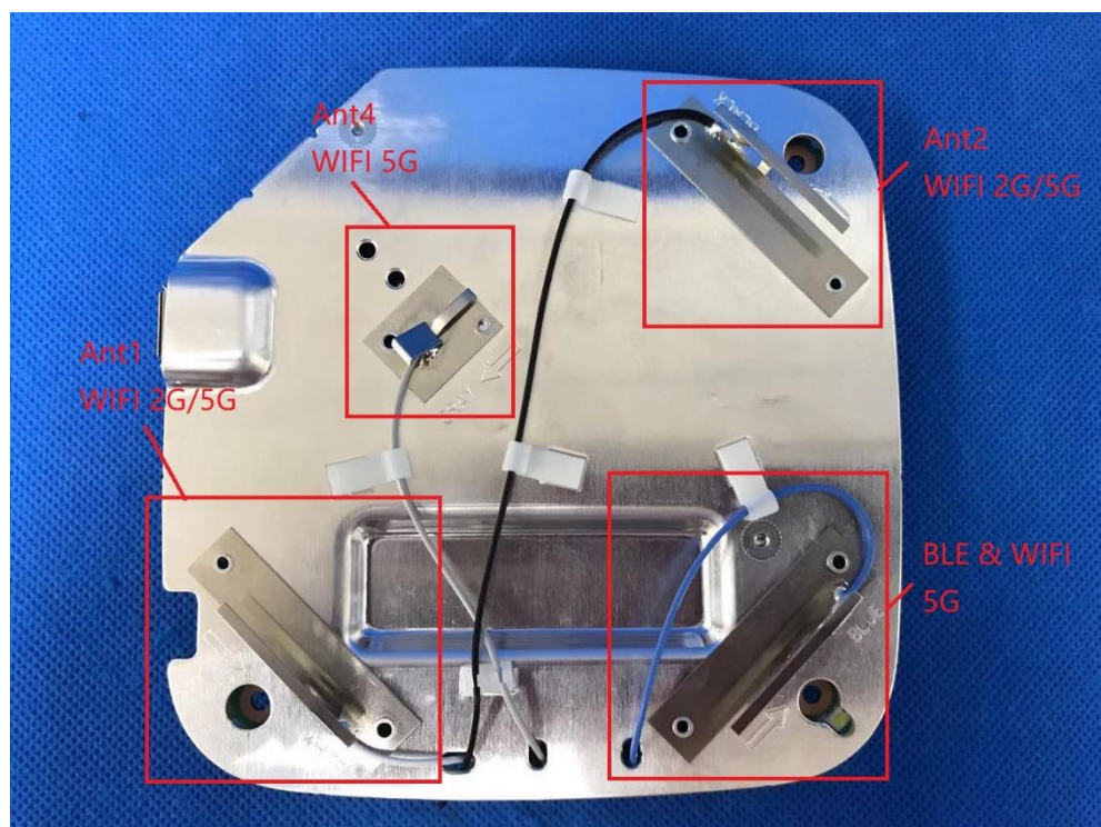
(2) EUT Photo(AP305C)
