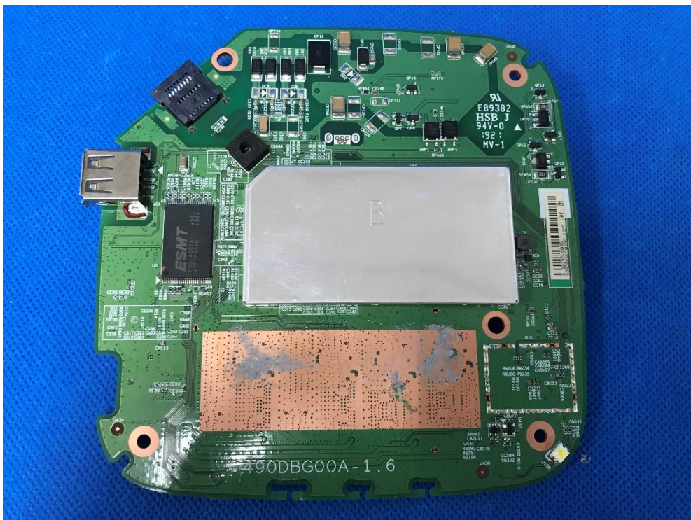
(10) EUT Photo(AP305CX)
