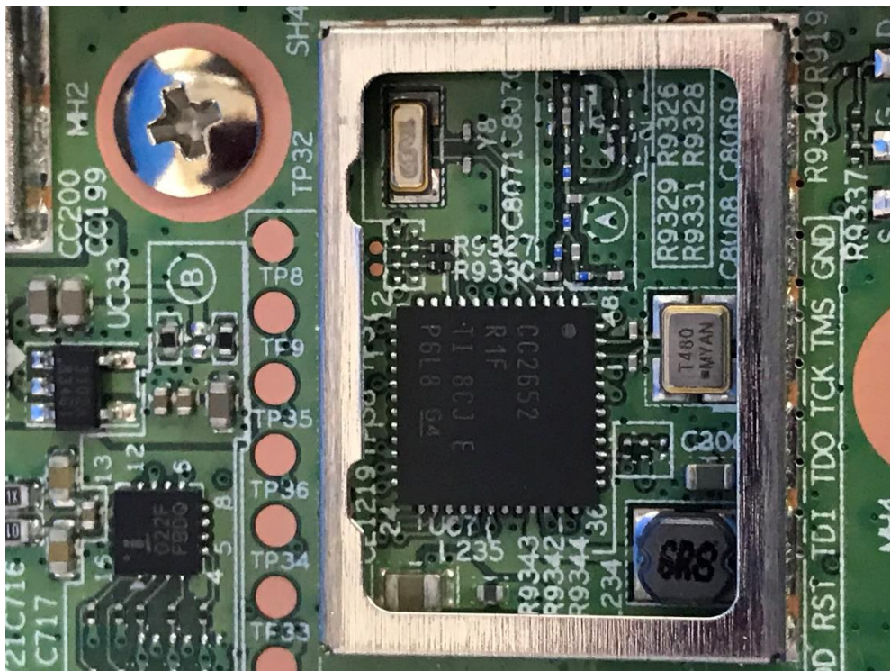
(14) EUT Photo(AP305CX)
