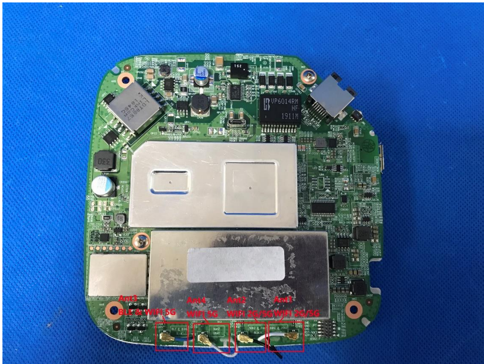
(1) EUT Photo(AP305C)
