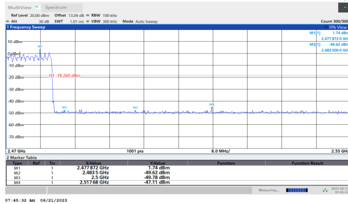
3DH5_Ant1_High_Hop_2480
