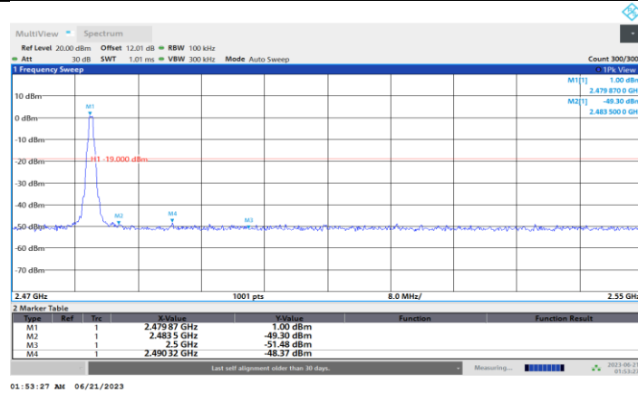
DH5_Ant1_High_2480
