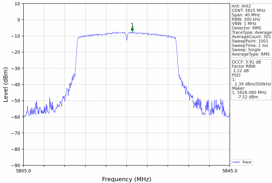
802.11ax(HEW20)_HCH_5825MHz_RU242_Left_MIMO_NTNV
