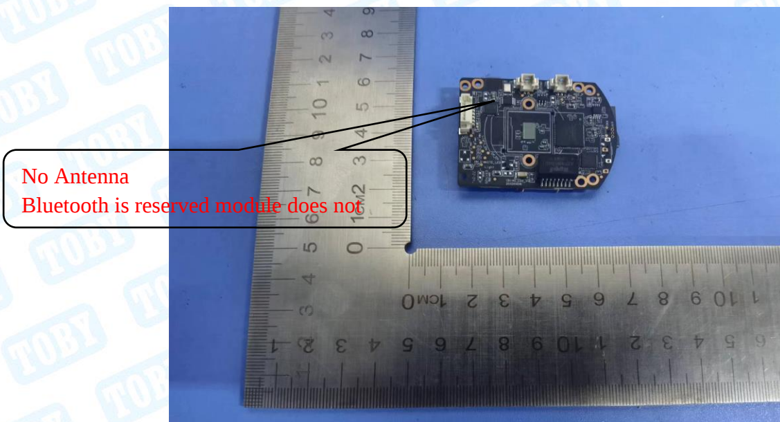
Photo 13 Appearance of PCB
