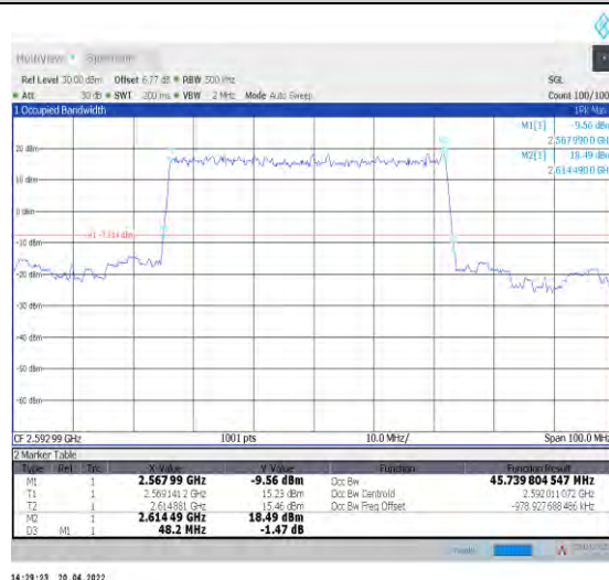
1-N41--30-50-M-2-DFT-PI2BPSK-Outer_Full-128@0 -Ant1-45.74-48.200-≤50-PASS
