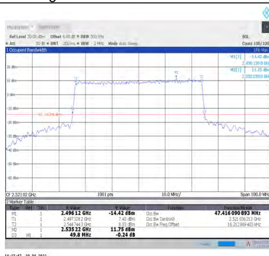
1-N41--30-50-L-9-CP-256QAM-Outer_Full-133@0-A nt1-47.416-49.800-≤50-PASS
