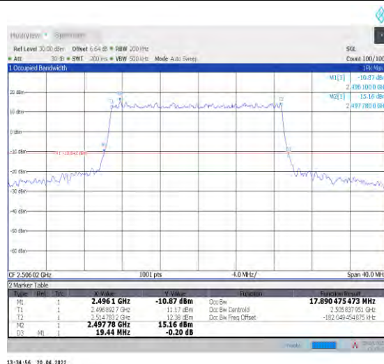
1-N41--30-20-L-4-DFT-64QAM-Outer_Full-50@0-Ant t1-17.89-19.440-≤20-PASS
