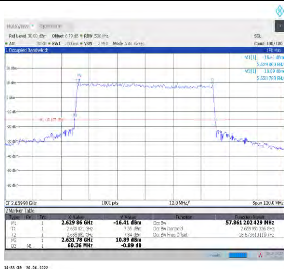
1-N41--30-60-H-9-CP-256QAM-Outer_Full-162@0-A nt1-57.861-60.360-≤60-PASS
