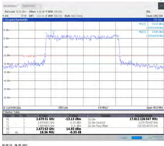
1-N41--30-20-H-3-DFT-16QAM-Outer_Full-50@0-An t1-17.812-18.560-≤20-PASS
