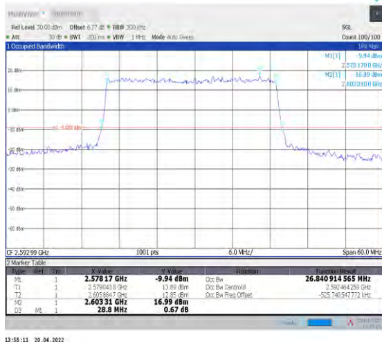
1-N41--30-30-M-1-DFT-QPSK-Outer_Full-75@0-Ant 1-26.841-28.800-≤30-PASS
