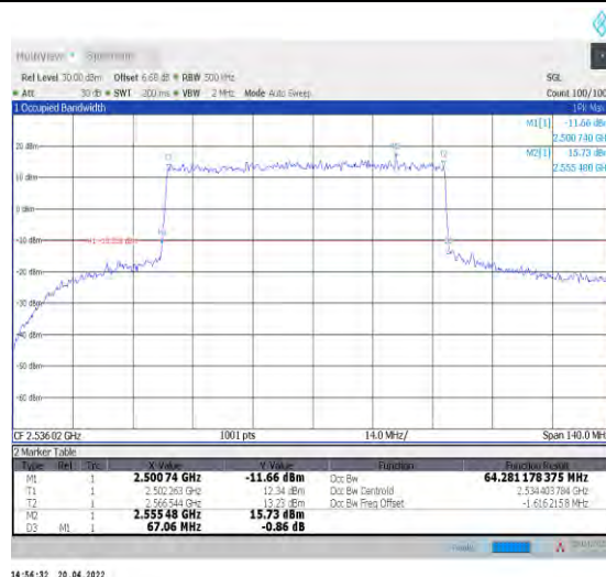
1-N41--30-70-L-1-DFT-QPSK-Outer_Full-180@0-Ant 1-64.281-67.060-≤70-PASS
