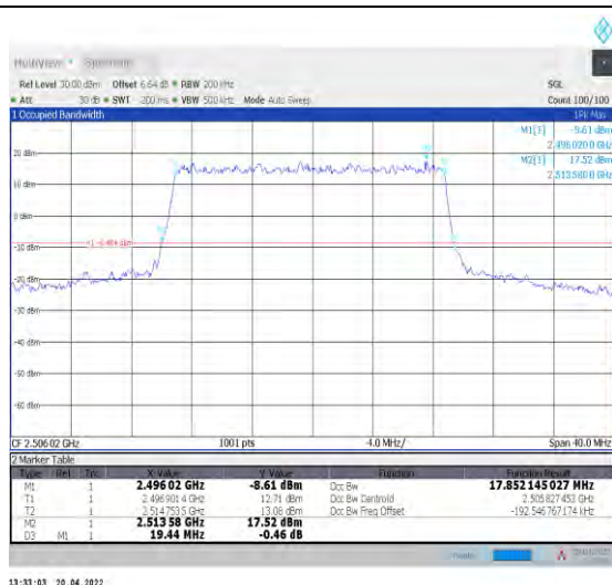
1-N41--30-20-L-1-DFT-QPSK-Outer_Full-50@0-Ant1 -17.852-19.440-≤20-PASS
