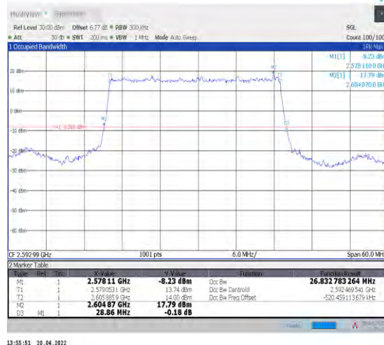
1-N41--30-30-M-2-DFT-PI2BPSK-Outer_Full-75@0-Ant 1-26.833-28.860-≤30-PASS
