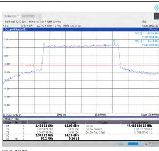
1-N41--30-50-L-8-CP-64QAM-Outer_Full-133@0-Ant 1-47.489-50.200-≤50-PASS
