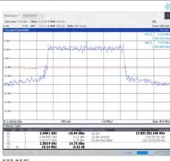
1-N41--30-20-L-3-DFT-16QAM-Outer_Full-50@0-Ant 1-17.851-19.240-≤20-PASS
