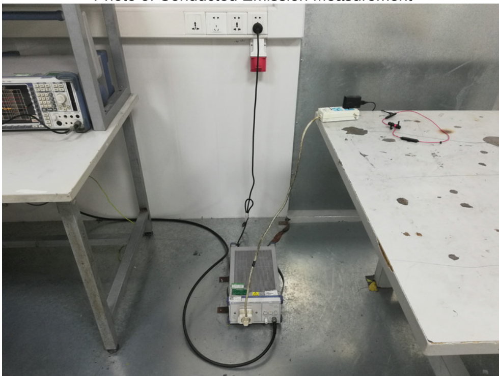
FCC ID: 2AG68-BT578 Photo of Conducted Emission Measurement
