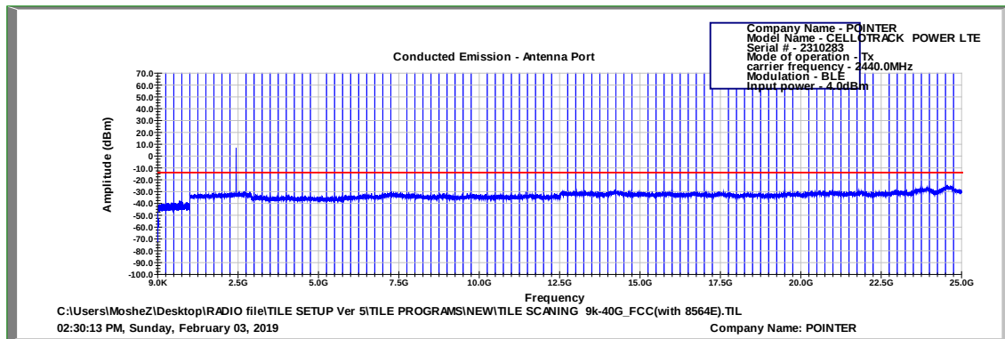
Figure 36 2440.0 MHz, BLE
