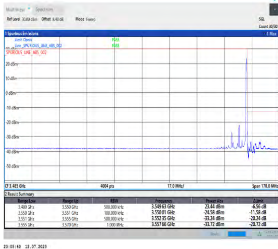
1-N77-3450-3550-PC1.5-30-10-H-2-DFT-PI2BPSK-Edge_1RB_Right-1@23-Ant3-1--PASS-see graph
