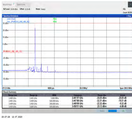
1-N77-3450-3550-PC1.5-30-20-L-1-DFT-PI2BPSK-Edge_1RB_Left-1@0-Ant3-1--PASS-see graph
