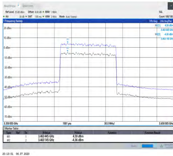
1-N77-3450-3550-PC1.5-30-100-L-1-DFT-256QAM-Outer_Full-270@0-Ant3-8.95-100%-0.00-8.95-PASS -≤13
