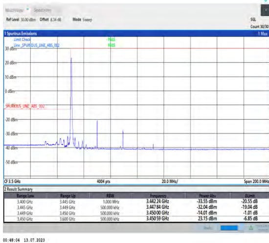
1-N77-3450-3550-PC1.5-30-40-L-4-CP-QPSK-Edge_1RB_Left-1@0-Ant3-1--PASS-see graph
