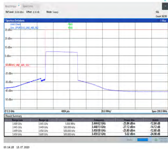
1-N77-3450-3550-PC1.5-30-40-L-6-CP-QPSK-Outer_Full-106@0-Ant3-1--PASS-see graph
