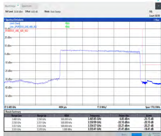
1-N77-3450-3550-PC1.5-30-90-H-3-DFT-PI2BPSK-Outer_Full-240@0-Ant3-1--PASS-see graph
