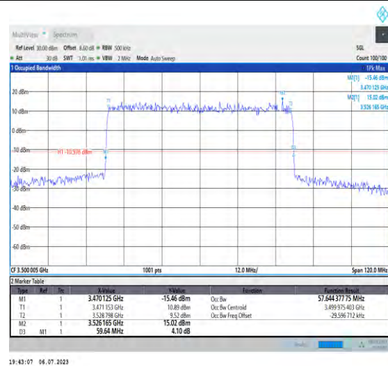
1-N77-3450-3550-PC1.5-30-60-M-1-DFT-QPSK-Out er_Full-162@0-Ant3-57.644-59.640-≤60-PASS
