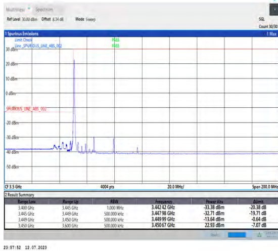
1-N77-3450-3550-PC1.5-30-30-L-1-DFT-PI2BPSK-Edge_1RB_Left-1@0-Ant3-1--PASS-see graph
