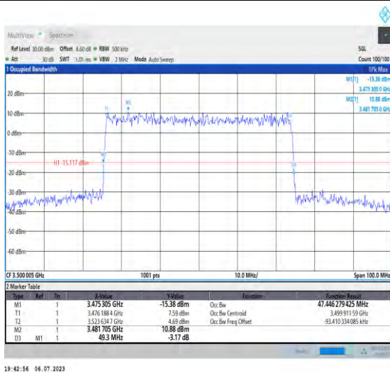
1-N77-3450-3550-PC1.5-30-50-M-9-CP-256QAM-Out er_Full-133@0-Ant3-47.446-49.300-≤50-PASS
