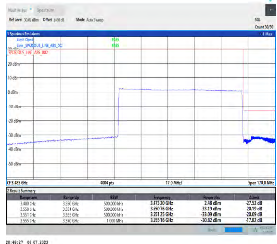
1-N77-3450-3550-PC1.5-30-80-H-6-CP-QPSK-Outet_Full-217@0-Ant3-1--PASS-see graph
