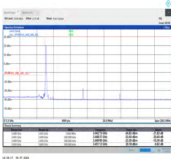
1-N77-3450-3550-PC1.5-30-90-L-4-CP-QPSK-Edge_1RB_Left-1@0-Ant3-1--PASS-see graph
