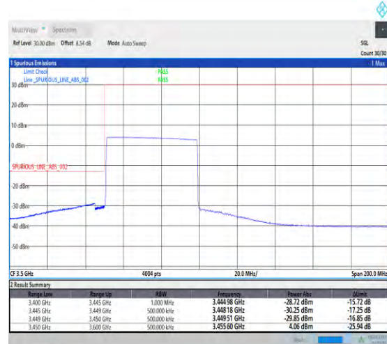
1-N77-3450-3550-PC1.5-30-50-L-3-DFT-PI2BPSK-Outer_Full-128@0-Ant3-1--PASS-see graph
