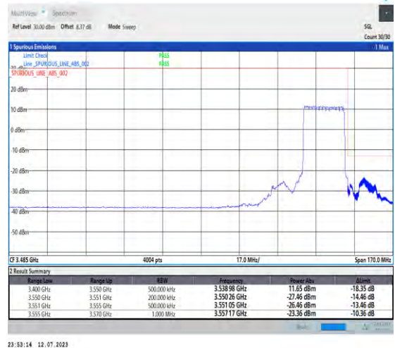
1-N77-3450-3550-PC1.5-30-20-H-3-DFT-PI2BPSK-Outer_Full-50@0-Ant3-1--PASS-see graph
