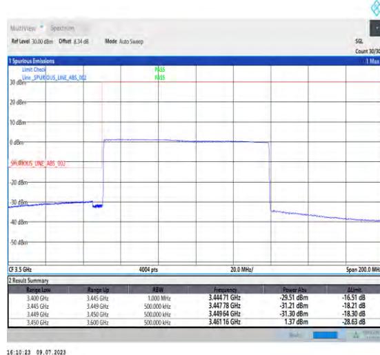
1-N77-3450-3550-PC1.5-30-90-L-6-CP-QPSK-Outer_Full-245@0-Ant3-1--PASS-see graph
