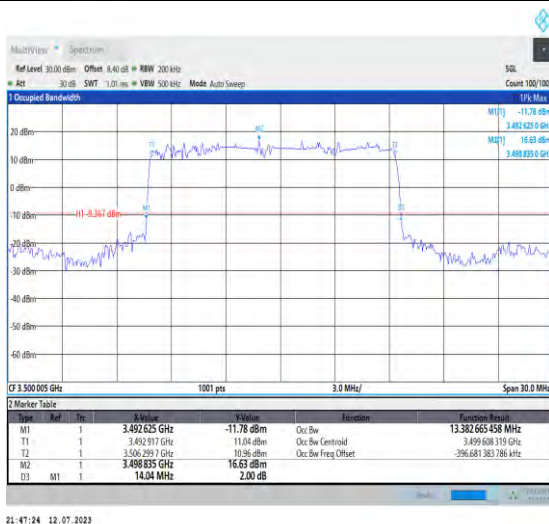
1-N77-3450-3550-PC1.5-30-15-M-2-DFT-PI2BPSK-Outer_Full-36@0-Ant3-13.383-14.040-≤30-PASS
