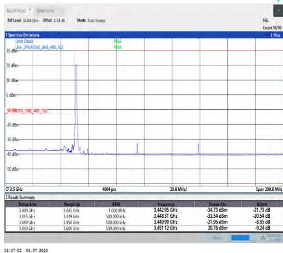
1-N77-3450-3550-PC1.5-30-90-L-1-DFT-PI2BPSK-Edge_1RB_Left-1@0-Ant3-1--PASS-see graph
