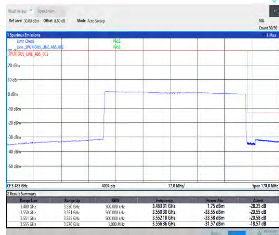
1-N77-3450-3550-PC1.5-30-90-H-6-CP-QPSK-Outer_Full-245@0-Ant3-1--PASS-see graph
