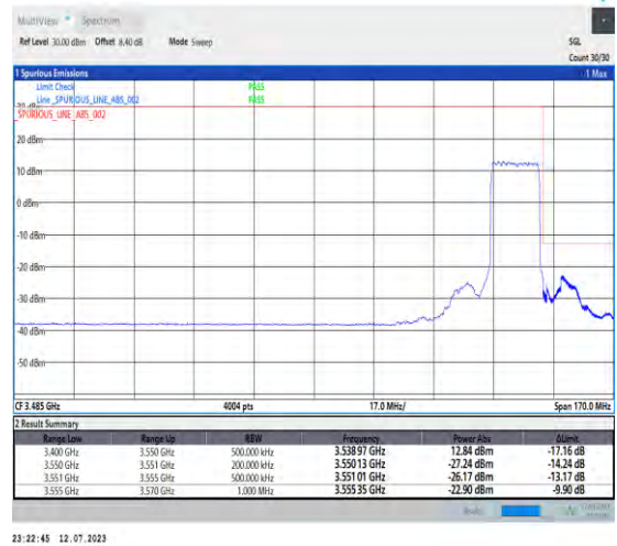
1-N77-3450-3550-PC1.5-30-15-H-3-DFT-PI2BPSK-Outer_Full-36@0-Ant3-1--PASS-see graph
