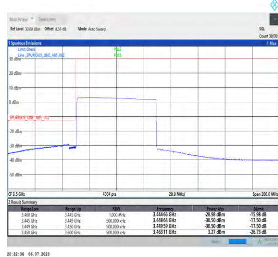
1-N77-3450-3550-PC1.5-30-60-L-6-CP-QPSK-Outer_Full-162@0-Ant3-1--PASS-see graph
