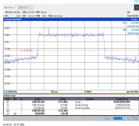
1-N77-3450-3550-PC1.5-30-30-M-4-DFT-64QAM-Ou ter_Full-75@0-Ant3-28.56-29.640-≤30-PASS
