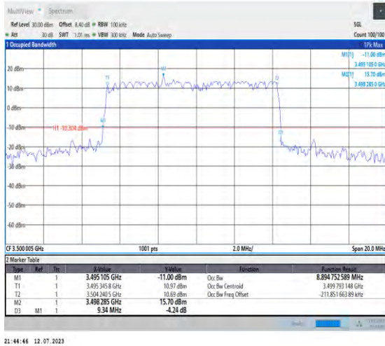
1-N77-3450-3550-PC1.5-30-10-M-1-DFT-QPSK-Out er_Full-24@0-Ant3-8.895-9.340-≤10-PASS
