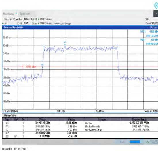
1-N77-3450-3550-PC1.5-30-10-M-9-CP-256QAM-Outer_Full-24@0-Ant3-9.273-9.680-≤10-PASS
