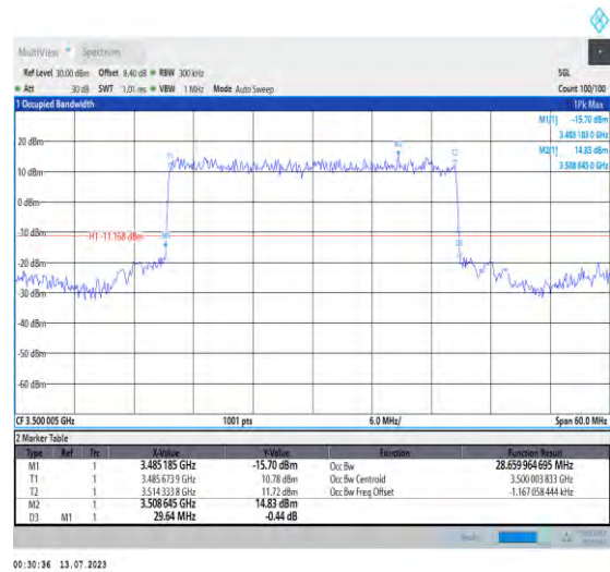
1-N77-3450-3550-PC1.5-30-30-M-2-DFT-PI2BPSK- Outer_Full-75@0-Ant3-28.66-29.640-≤30-PASS
