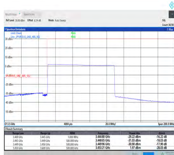
1-N77-3450-3550-PC1.5-30-80-L-3-DFT-PI2BPSK-Outer_Full-100@0-Ant3-1--PASS-see graph
