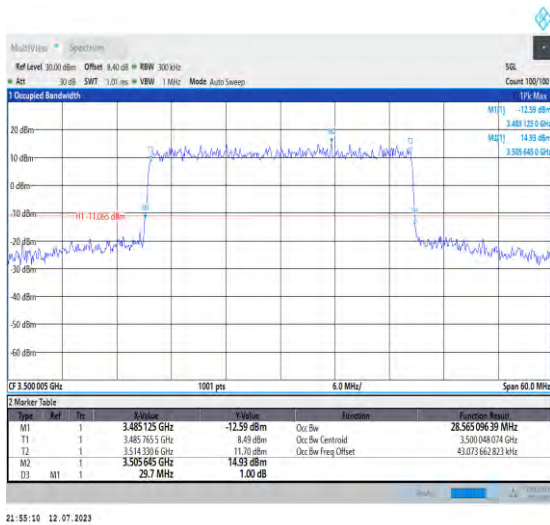
1-N77-3450-3550-PC1.5-30-30-M-1-DFT-QPSK-Out er_Full-75@0-Ant3-28.565-29.700-≤30-PASS
