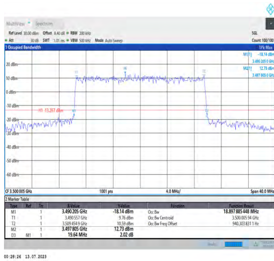
1-N77-3450-3550-PC1.5-30-20-M-7-CP-16QAM-Out er_Full-51@0-Ant3-18.898-19.640-≤20-PASS
