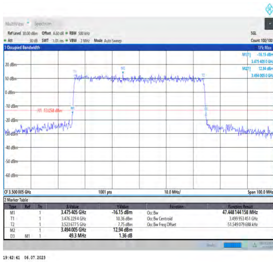
1-N77-3450-3550-PC1.5-30-50-M-7-CP-16QAM-Out er_Full-133@0-Ant3-47.448-49.300-≤50-PASS
