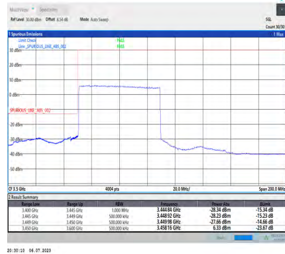
1-N77-3450-3550-PC1.5-30-60-L-3-DFT-PI2BPSK-Outer_Full-162@0-Ant3-1--PASS-see graph
