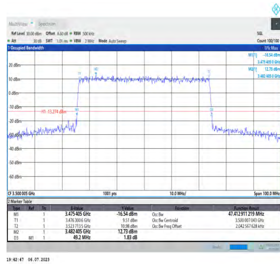
1-N77-3450-3550-PC1.5-30-50-M-8-CP-64QAM-Out er_Full-133@0-Ant3-47.413-49.200-≤50-PASS
