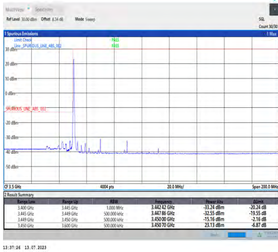
1-N77-3450-3550-PC1.5-30-40-L-1-DFT-PI2BPSK-Edge_1RB_Left-1@0-Ant3-1--PASS-see graph
