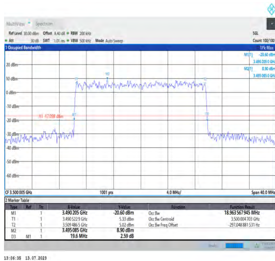
1-N77-3450-3550-PC1.5-30-20-M-9-CP-256QAM-Out er_Full-51@0-Ant3-18.964-19.600-≤20-PASS
