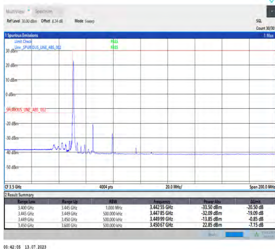
1-N77-3450-3550-PC1.5-30-30-L-4-CP-QPSK-Edge_1RB_Left-1@0-Ant3-1--PASS-see graph
