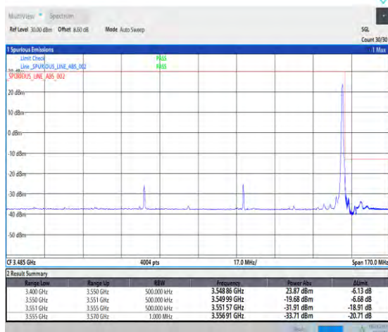
1-N77-3450-3550-PC1.5-30-90-H-5-CP-QPSK-Edge_1RB_Right-1@244-Ant3-1--PASS-see graph
