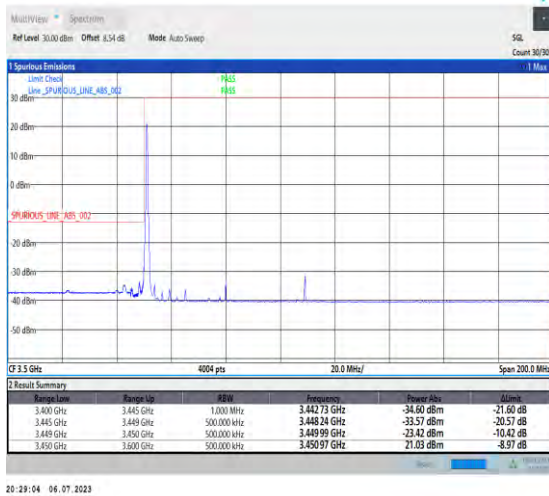
1-N77-3450-3550-PC1.5-30-60-L-1-DFT-PI2BPSK-Edge_1RB_Left-1@0-Ant3-1--PASS-see graph
