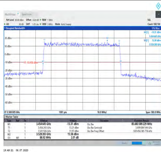
1-N77-3450-3550-PC1.5-30-90-M-3-DFT-16QAM-Out_Full-240@0-Ant3-85.684-88.920-≤90-PASS
