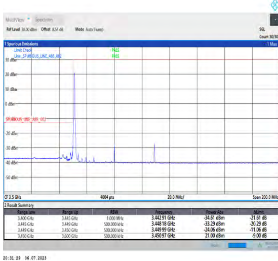
1-N77-3450-3550-PC1.5-30-60-L-4-CP-QPSK-Edge_1RB_Left-1@0-Ant3-1--PASS-see graph
