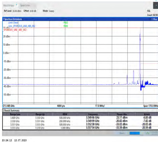
1-N77-3450-3550-PC1.5-30-15-H-5-CP-QPSK-Edge_1RB_Right-1@37-Ant3-1--PASS-see graph
