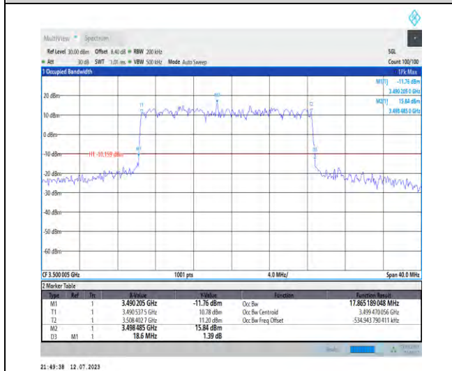
1-N77-3450-3550-PC1.5-30-20-M-1-DFT-QPSK-Out_Full-50@0-Ant3-17.865-18.600-≤20-PASS
