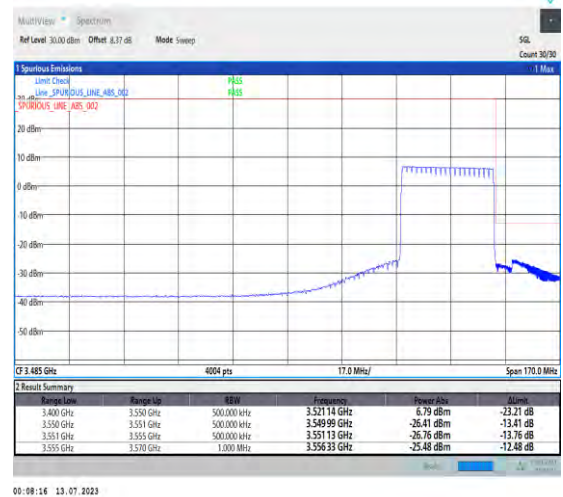
1-N77-3450-3550-PC1.5-30-30-H-6-CP-QPSK-Outer_Full-75@0-Ant3-1--PASS-see graph
