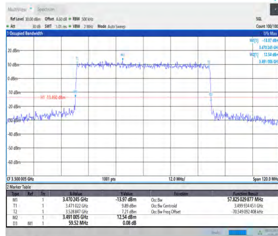
1-N77-3450-3550-PC1.5-30-60-M-7-CP-16QAM-Outer_Full-162@0-Ant3-57.825-59.520-≤60-PASS
