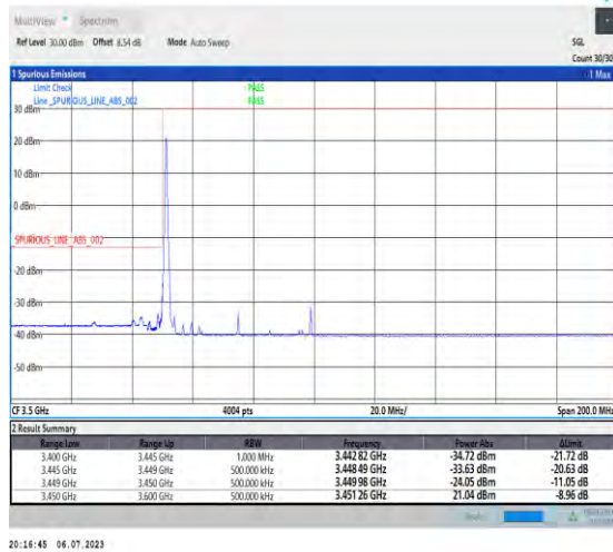
1-N77-3450-3550-PC1.5-30-50-L-1-DFT-PI2BPSK-Edge_1RB_Left-1@0-Ant3-1--PASS-see graph
