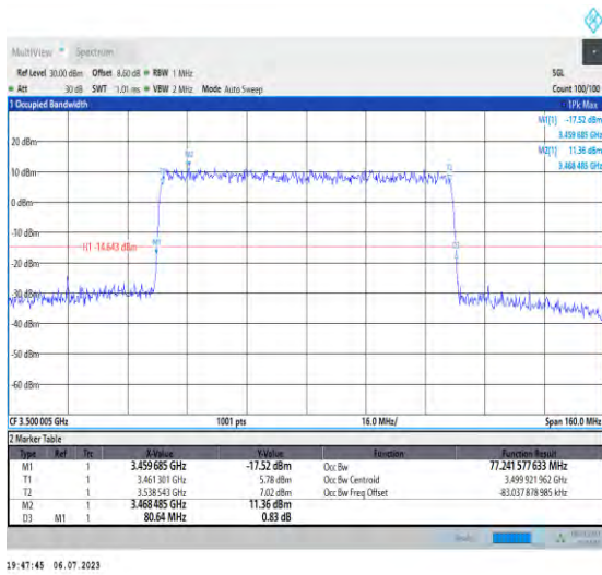
1-N77-3450-3550-PC1.5-30-80-M-9-CP-256QAM-Out_Full-217@0-Ant3-77.242-80.640-≤80-PASS
