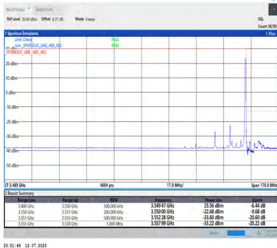
1-N77-3450-3550-PC1.5-30-20-H-2-DFT-PI2BPSK-Edge_1RB_Right-1@50-Ant3-1--PASS-see graph
