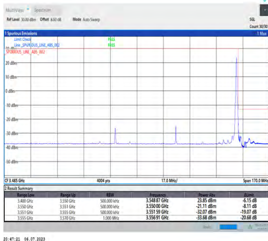
1-N77-3450-3550-PC1.5-30-80-H-5-CP-QPSK-Edge_1RB_Right-1@216-Ant3-1--PASS-see graph
