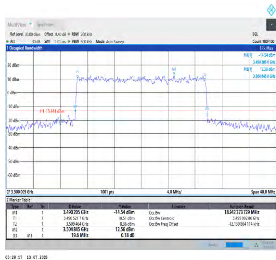
1-N77-3450-3550-PC1.5-30-20-M-6-CP-QPSK-Outer_Full-51@0-Ant3-18.942-19.600-≤20-PASS
