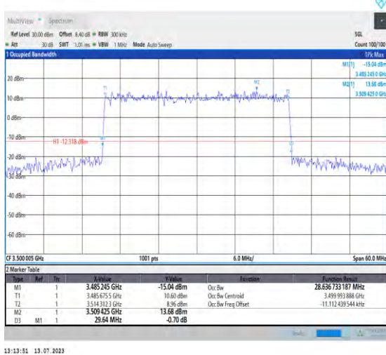
1-N77-3450-3550-PC1.5-30-30-M-3-DFT-16QAM-O uter_Full-75@0-Ant3-28.637-29.640-≤30-PASS
