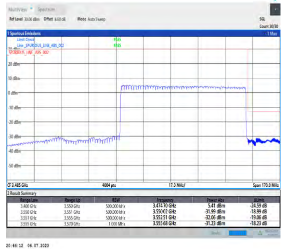
1-N77-3450-3550-PC1.5-30-80-H-3-DFT-PI2BPSK-Outet_Full-100@0-Ant3-1--PASS-see graph
