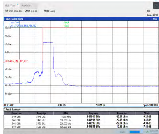
1-N77-3450-3550-PC1.5-30-15-L-3-DFT-PI2BPSK-Outer_Full-36@0-Ant3-1--PASS-see graph
