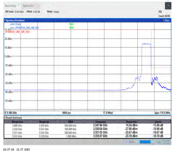
1-N77-3450-3550-PC1.5-30-10-H-3-DFT-PI2BPSK-Outer_Full-24@0-Ant3-1--PASS-see graph
