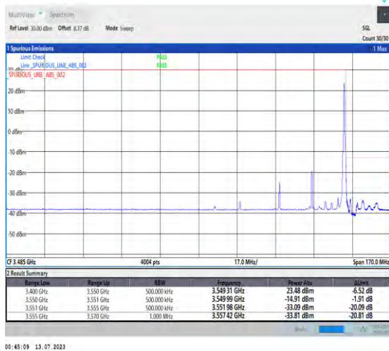
1-N77-3450-3550-PC1.5-30-30-H-5-CP-QPSK-Edge_1RB_Right-1@77-Ant3-1--PASS-see graph
