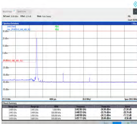
1-N77-3450-3550-PC1.5-30-80-L-1-DFT-PI2BPSK-Edge_1RB_Left-1@0-Ant3-1--PASS-see graph
