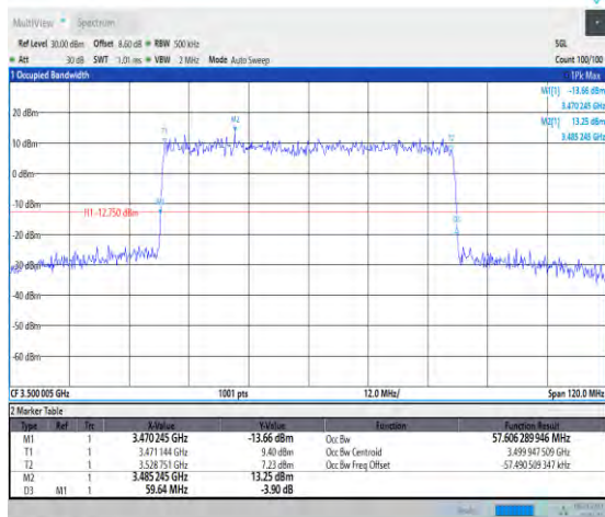
1-N77-3450-3550-PC1.5-30-60-M-8-CP-64QAM-Outer_Full-162@0-Ant3-57.606-59.640-≤60-PASS
