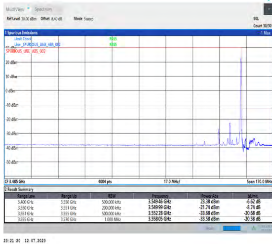
1-N77-3450-3550-PC1.5-30-15-H-2-DFT-PI2BPSK-Edge_1RB_Right-1@37-Ant3-1--PASS-see graph
