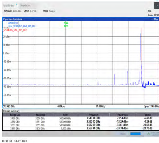
1-N77-3450-3550-PC1.5-30-30-H-2-DFT-PI2BPSK-Edge_1RB_Right-1@77-Ant3-1--PASS-see graph
