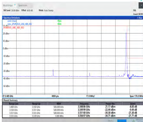
1-N77-3450-3550-PC1.5-30-90-H-2-DFT-PI2BPSK-Edge_1RB_Right-1@244-Ant3-1--PASS-see graph
