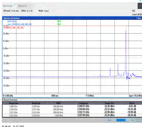
1-N77-3450-3550-PC1.5-30-20-H-5-CP-QPSK-Edge_1RB_Right-1@50-Ant3-1--PASS-see graph
