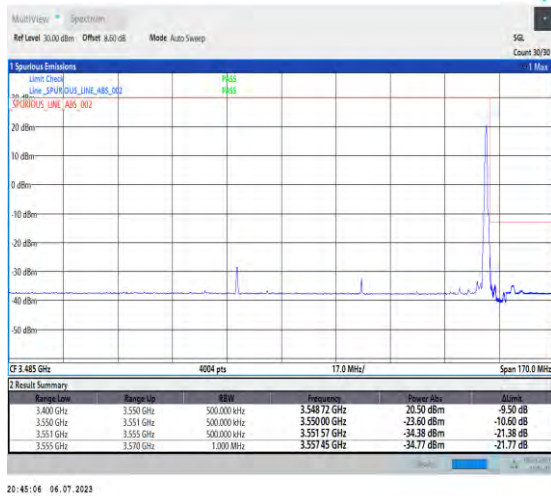
1-N77-3450-3550-PC1.5-30-80-H-2-DFT-PI2BPSK-Edge_1RB_Right-1@216-Ant3-1--PASS-see graph
