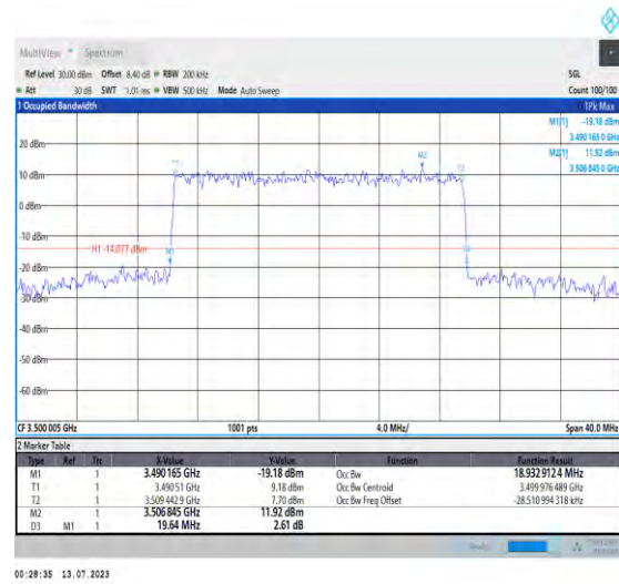
1-N77-3450-3550-PC1.5-30-20-M-8-CP-64QAM-Out er_Full-51@0-Ant3-18.933-19.640-≤20-PASS
