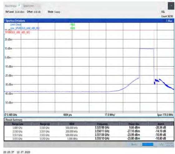
1-N77-3450-3550-PC1.5-30-15-H-6-CP-QPSK-Outer_Full-38@0-Ant3-1--PASS-see graph
