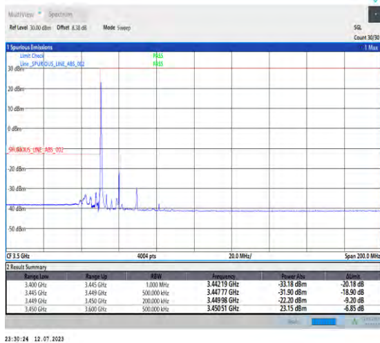
1-N77-3450-3550-PC1.5-30-20-L-4-CP-QPSK-Edge_1RB_Left-1@0-Ant3-1--PASS-see graph
