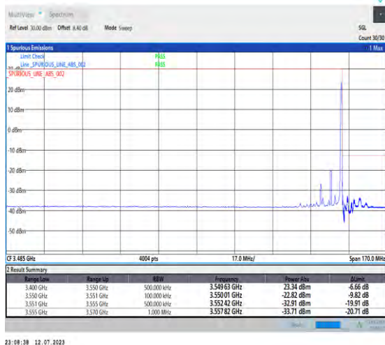
1-N77-3450-3550-PC1.5-30-10-H-5-CP-QPSK-Edge_1RB_Right-1@23-Ant3-1--PASS-see graph
