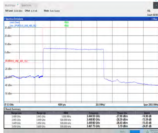
1-N77-3450-3550-PC1.5-30-80-L-3-DFT-PI2BPSK-Outer_Full-100@0-Ant3-1--PASS-see graph
