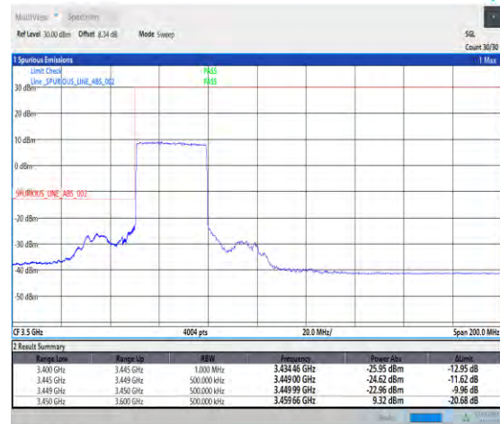
1-N77-3450-3550-PC1.5-30-30-L-3-DFT-PI2BPSK-Outer_Full-75@0-Ant3-1--PASS-see graph
