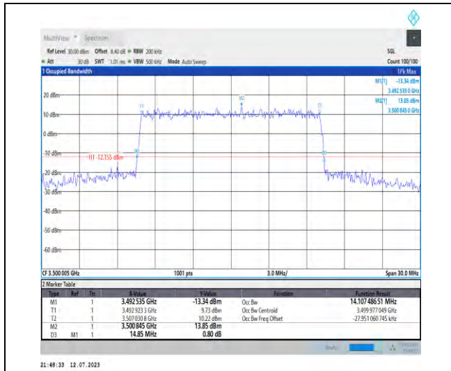
1-N77-3450-3550-PC1.5-30-15-M-8-CP-64QAM-Out_Full-38@0-Ant3-14.107-14.850-≤30-PASS
