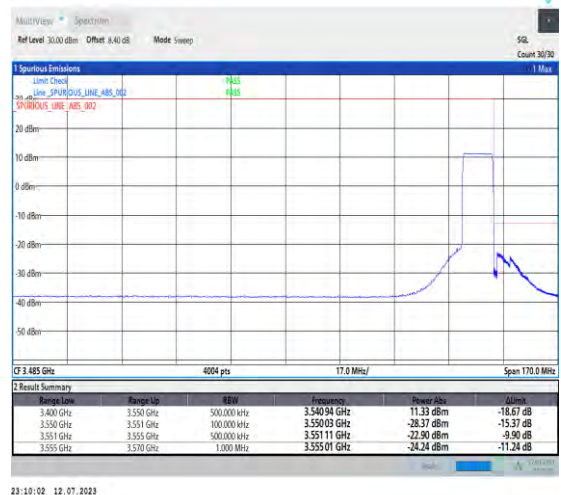
1-N77-3450-3550-PC1.5-30-10-H-6-CP-QPSK-Outer_Full-24@0-Ant3-1--PASS-see graph
