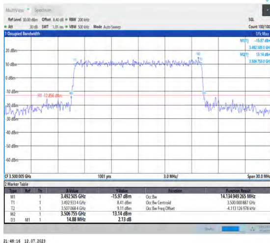
1-N77-3450-3550-PC1.5-30-15-M-6-CP-QPSK-Outer_Full-38@0-Ant3-14.135-14.880-≤30-PASS
