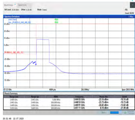
1-N77-3450-3550-PC1.5-30-20-L-6-CP-QPSK-Outer_Full-51@0-Ant3-1--PASS-see graph
